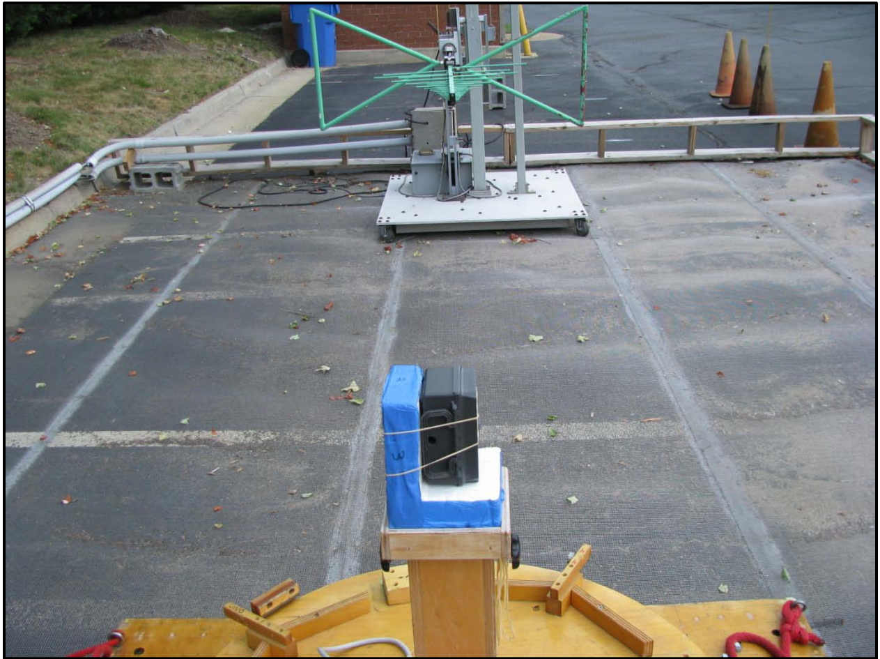
Photograph 4: Radiated Emissions
