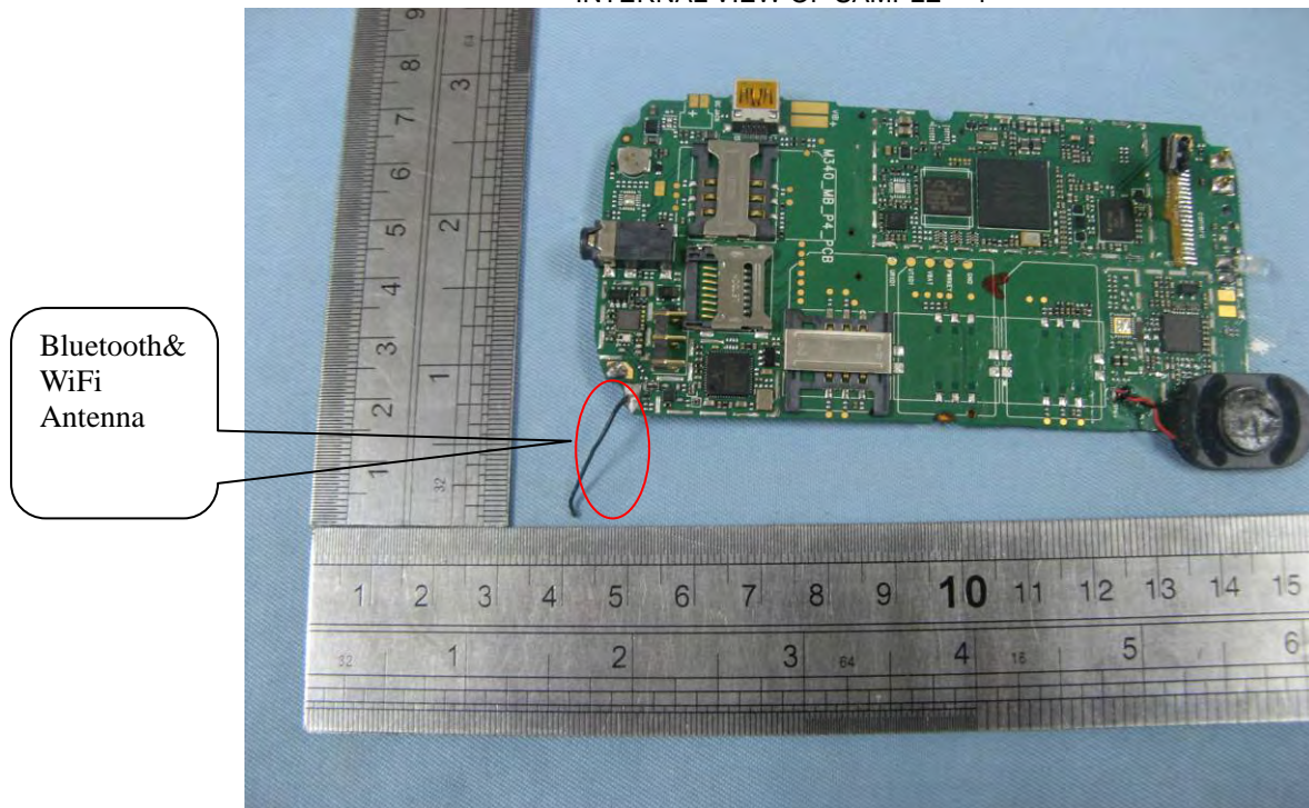
INTERNAL VIEW OF SAMPLE – 4
