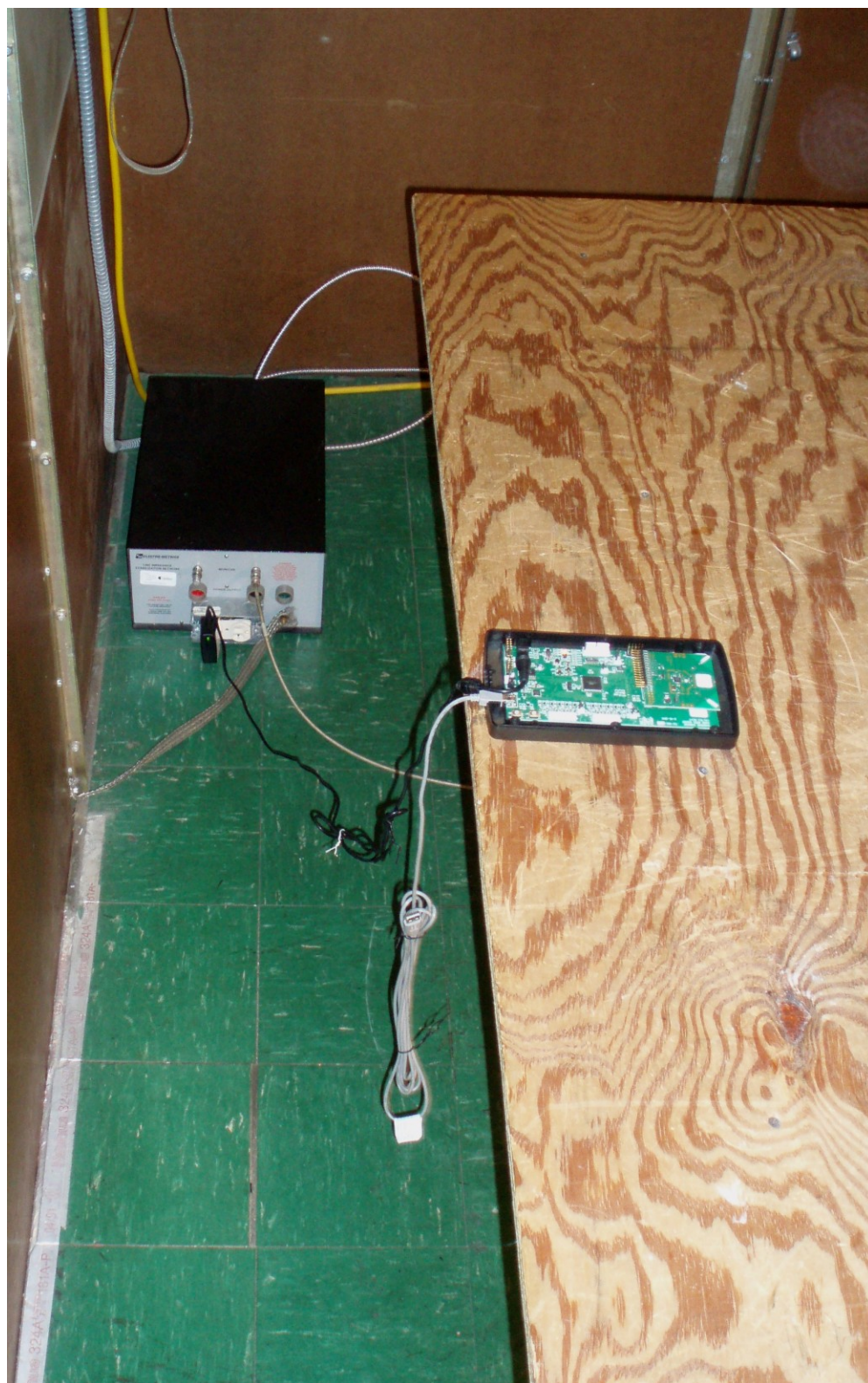
POWERLINE CONDUCTED EMISSIONS TEST SET UP PHOTO
