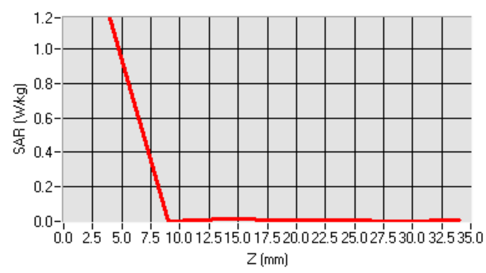
SAR, Z Axis Scan (X = 22, Y = 17)
