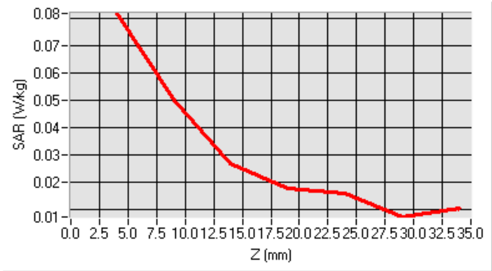
SAR, Z Axis Scan (X = -16, Y = -2)
