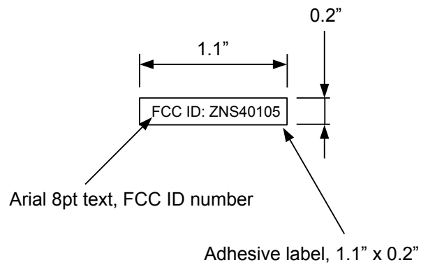
FCC ID Label detail and dimensions
