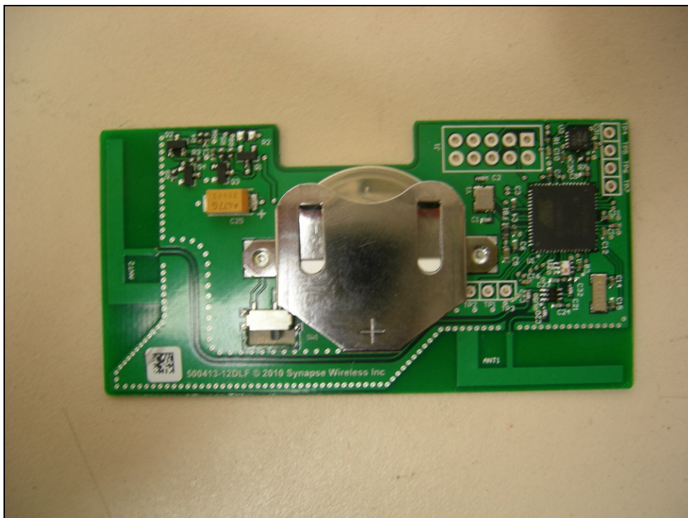
Figure 2: PCB – Front
