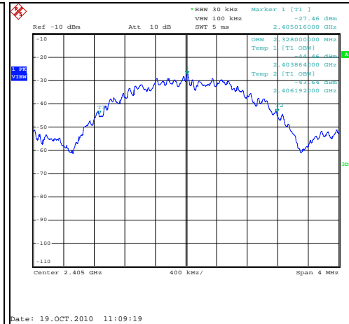
Figure 7.3.2-4: 99% – Low Channel
