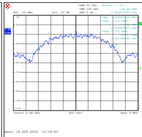
Figure 7.3.2-6: 99% – High Channel
