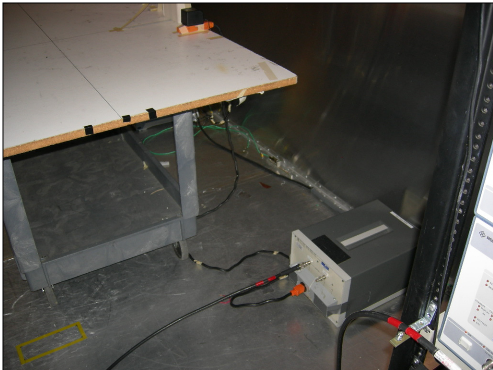
Figure 6: Conducted Emissions
