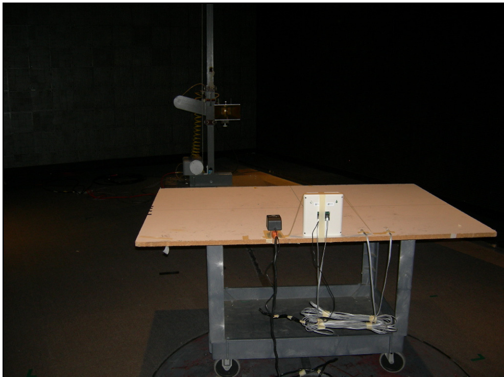
Figure 2: Radiated Emissions with Power Supply
