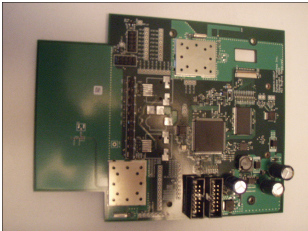
Figure 4: PCB Front – With Shields
