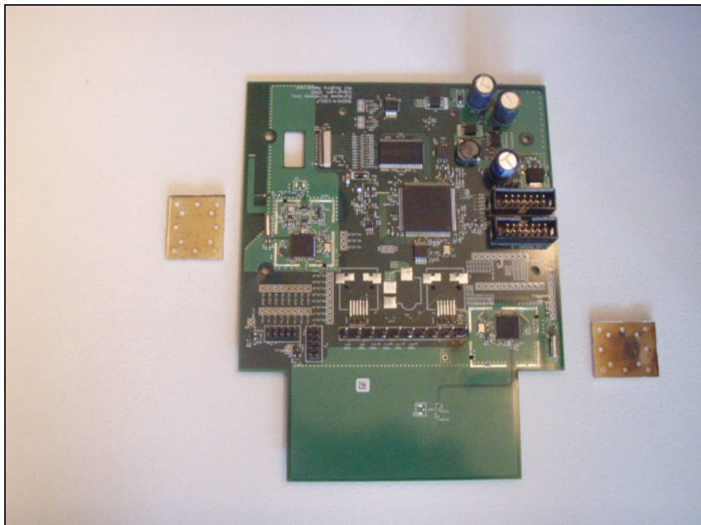
Figure 6: PCB Front – Without Shields
