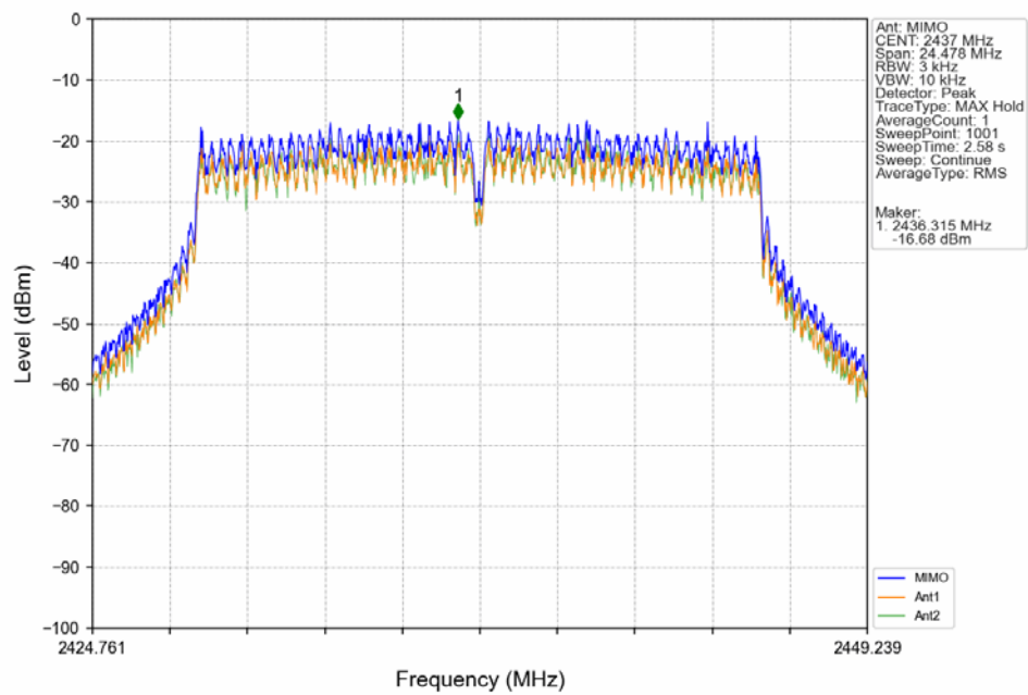
802.11n(HT20)_MCH_2437MHz_MIMO NTN
