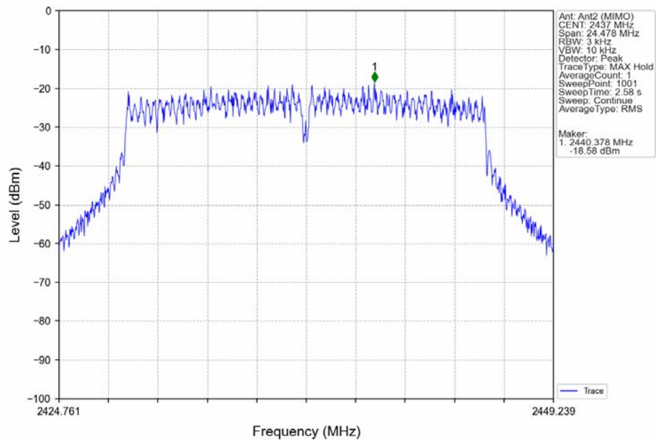
802.11n(HT20)_MCH_2437MHz_MIMO NTN
