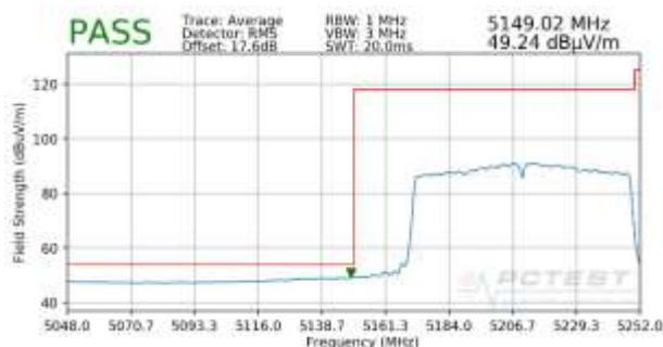
Plot 7-111. Radiated Lower Band Edge Plot (Average – UNII Band 1)
