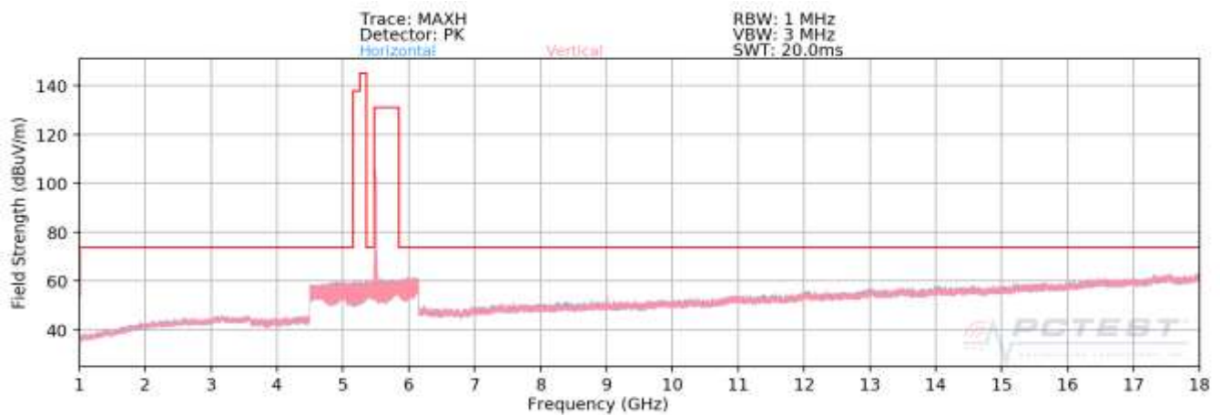
Plot 7-79. Radiated Spurious Plot above 1GHz (802.11a – U2C Ch. 116)
