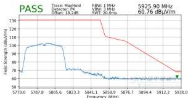
Plot 7-110. Radiated Upper Band Edge Plot (Peak – UNII Band 3)
