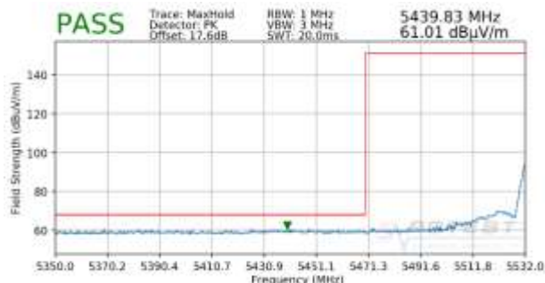
Plot 7-108. Radiated Lower Band Edge Plot (Peak – UNII Band 2C)
