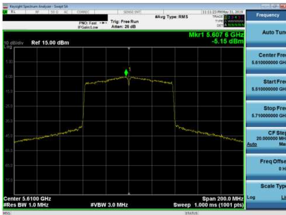
Plot 7-66. Power Spectral Density Plot (80MHz BW 802.11ac (UNII Band 2C) – Ch. 122)
