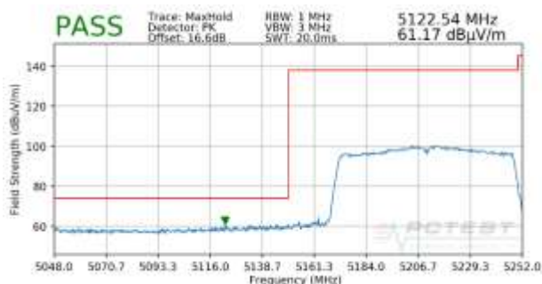
Plot 7-112. Radiated Lower Band Edge Plot (Peak – UNII Band 1)
