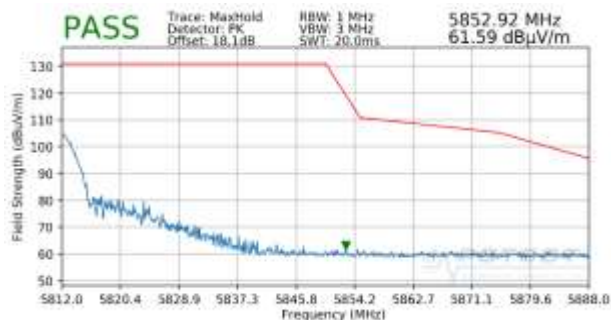
Plot 7-95. Radiated Upper Band Edge Plot (Peak – UNII Band 3)
