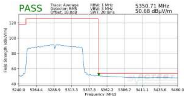
Plot 7-113. Radiated Upper Band Edge Plot (Average – UNII Band 2A)
