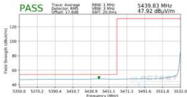
Plot 7-107. Radiated Lower Band Edge Plot (Average – UNII Band 2C)
