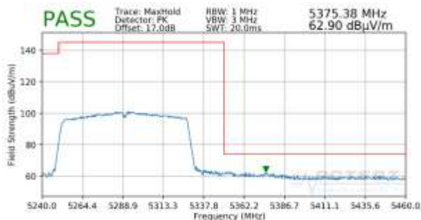
Plot 7-114. Radiated Upper Band Edge Plot (Peak – UNII Band 2A)
