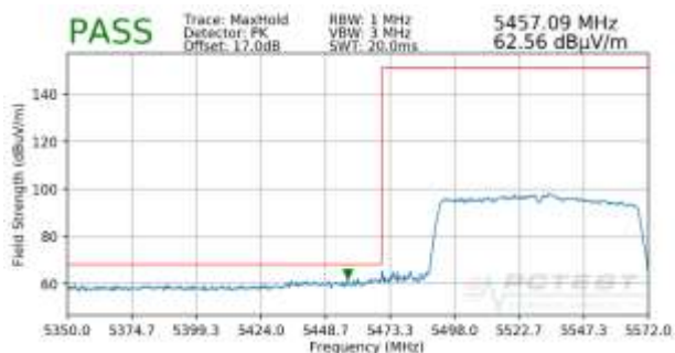
Plot 7-116. Radiated Lower Band Edge Plot (Peak – UNII Band 2C)
