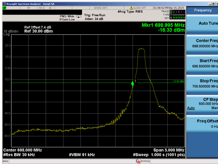
LTE Band 12 / 1.4MHz / QPSK - RB Size/Offset (1/0)
