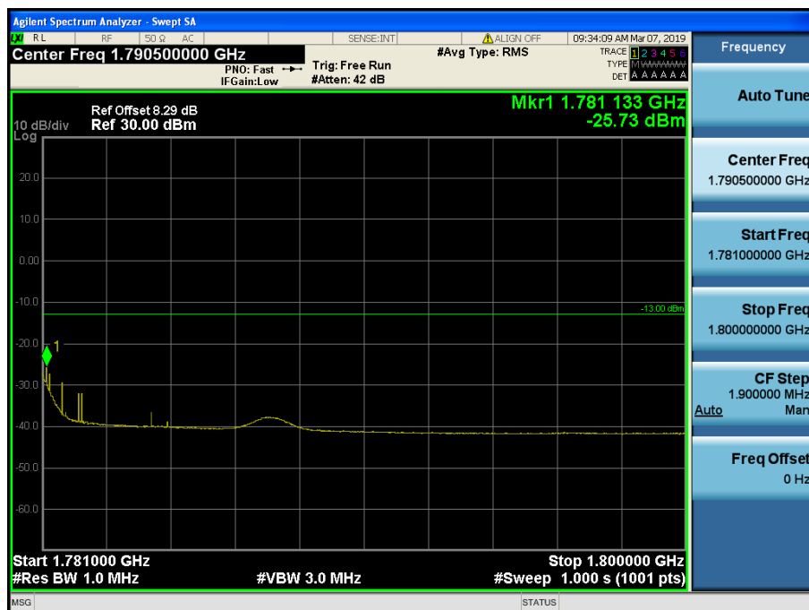
LTE Band 66, 4 / 20MHz / QPSK - RB Size/Offset (1/99)
