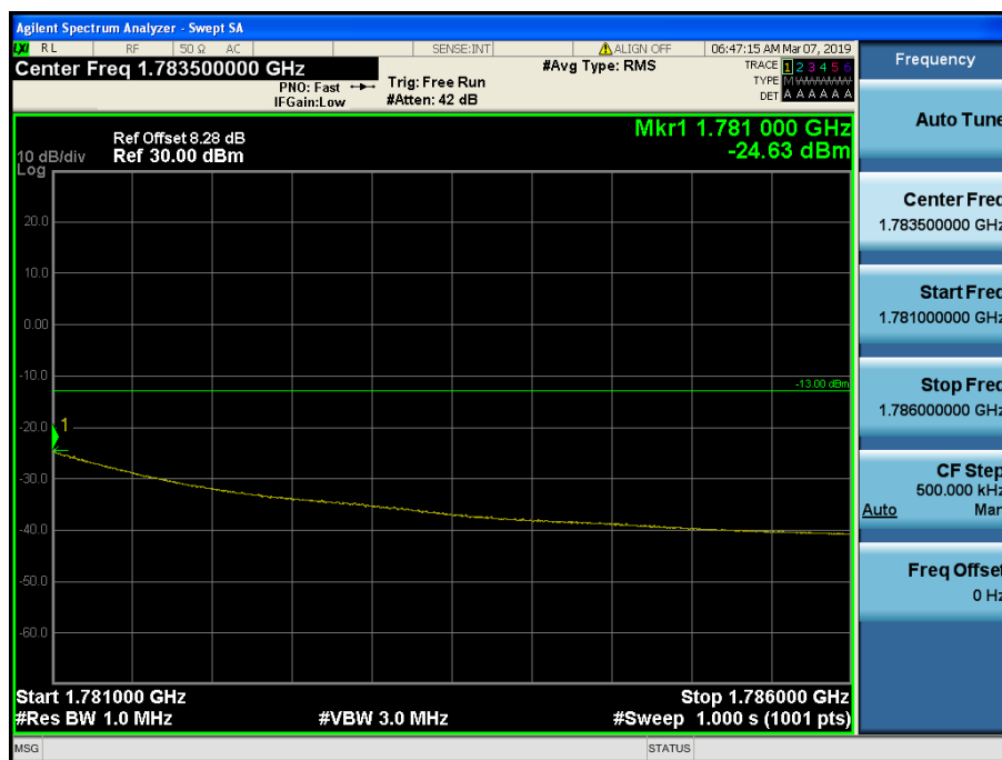
LTE Band 66, 4 / 3MHz / QPSK - RB Size/Offset (12/6)
