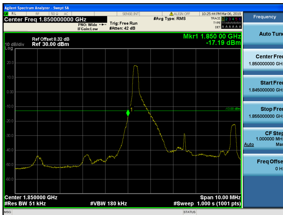
LTE Band 2 / 5MHz / 16QAM Size/offset (1/0)
