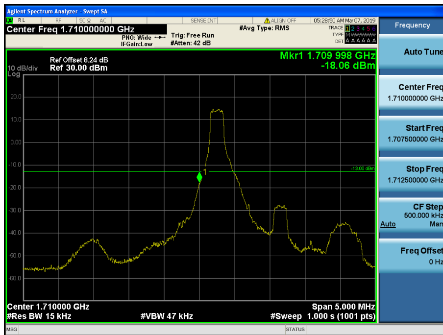
LTE Band 66, 4 / 1.4MHz / QPSK - RB Size/Offset (1/0)
