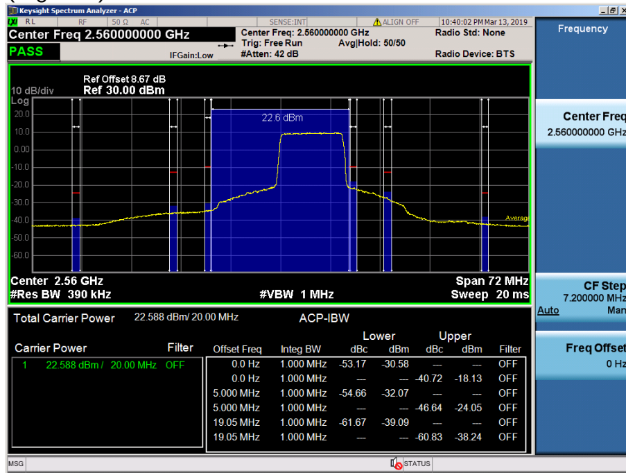
LTE Band 7 / 20MHz / QPSK - RB Size/Offset (50/50)
