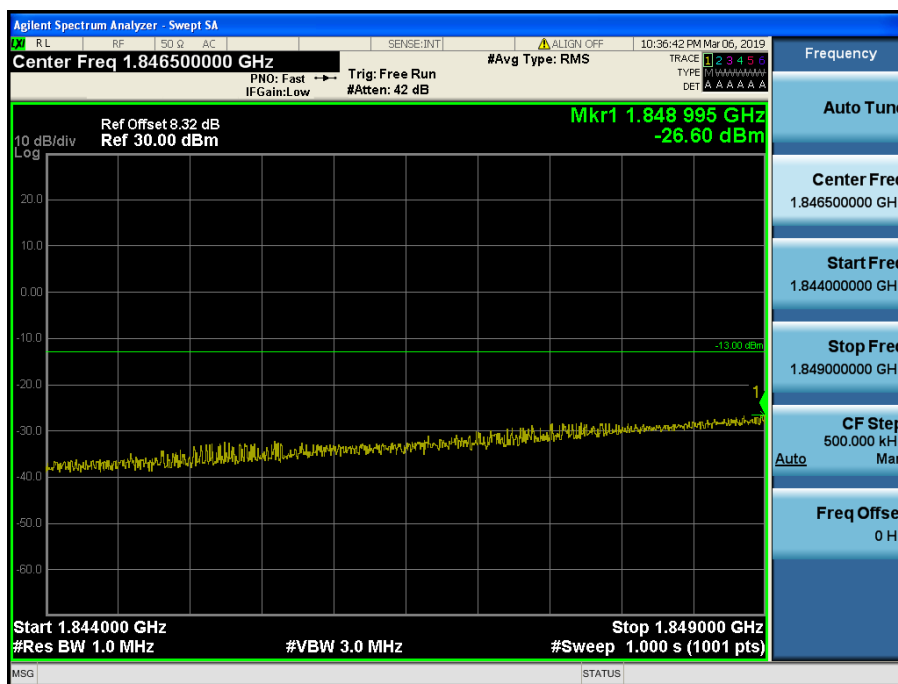
LTE Band 2 / 5MHz / 16QAM Size/Offset (12/6)
