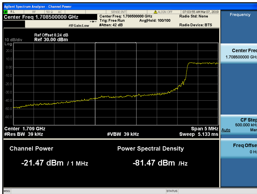
LTE Band 66, 4 / 5MHz / QPSK Offset/Size (12/0)
