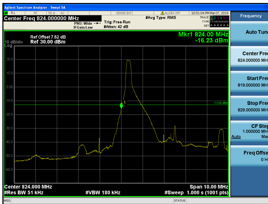
LTE Band 5 / 5MHz / 16QAM Size/Offset (1/0)
