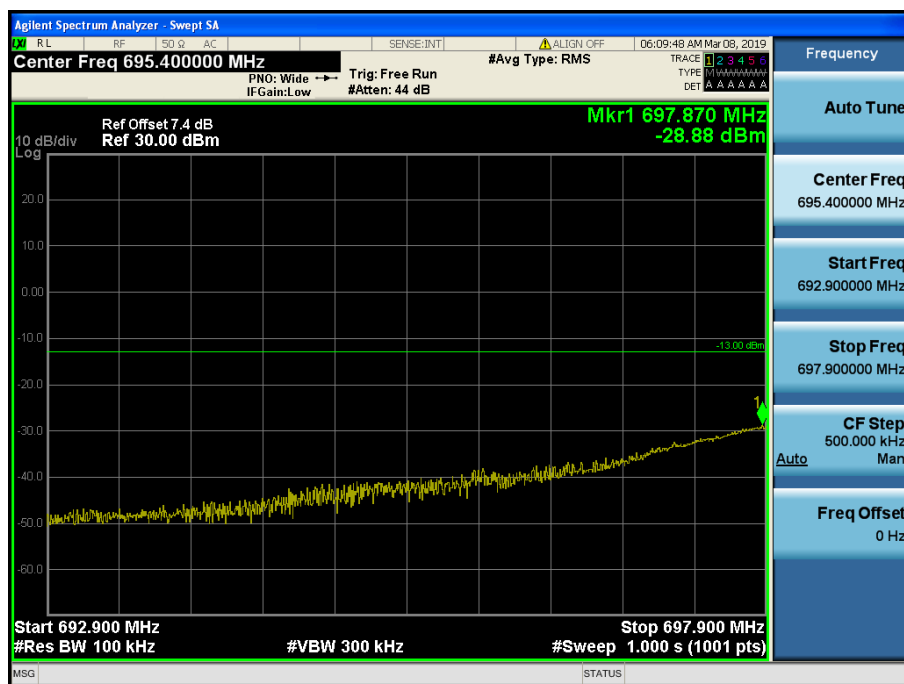
LTE Band 12, 17 / 5MHz / 16QAM Offset/Size (12/0)
