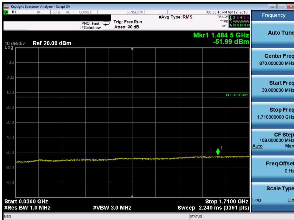
Plot 7-83. Conducted Spurious Plot (Band 66/4 - 10.0MHz QPSK - RB Size 1, RB Offset 0 - Mid Channel)
