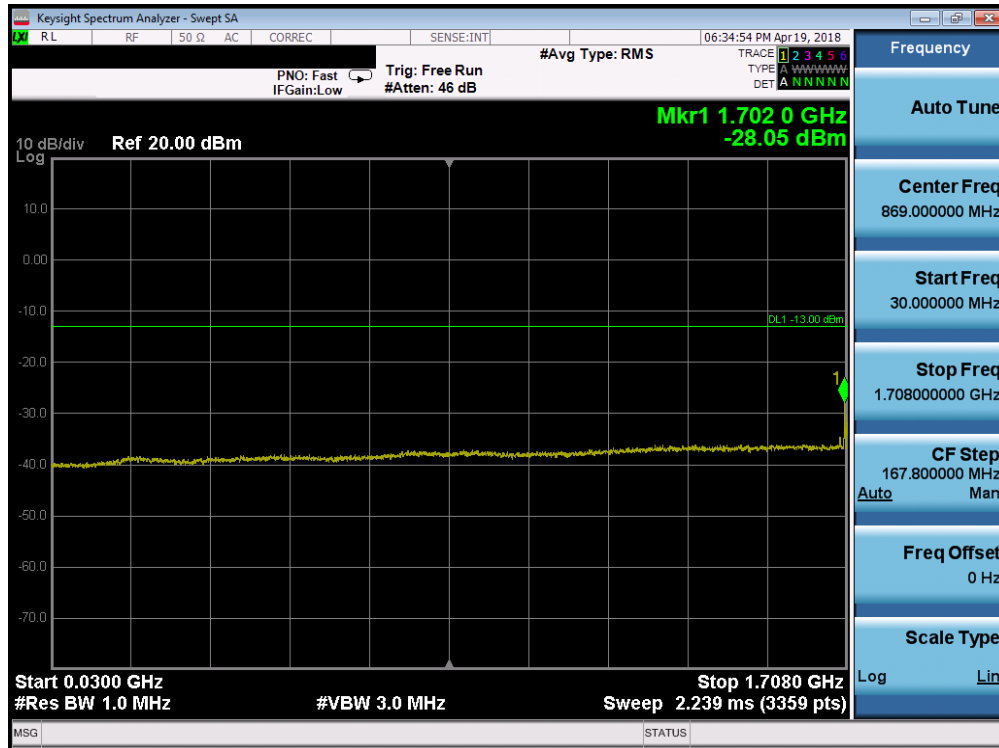
Plot 7-80. Conducted Spurious Plot (Band 66/4 - 10.0MHz QPSK - RB Size 1, RB Offset 0 - Low Channel)
