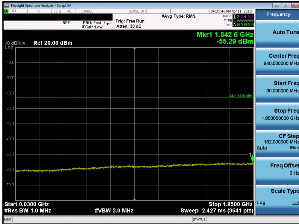
Plot 7-95. Conducted Spurious Plot (Band 2 - 10.0MHz QPSK - RB Size 1, RB Offset 0 - High Channel)
