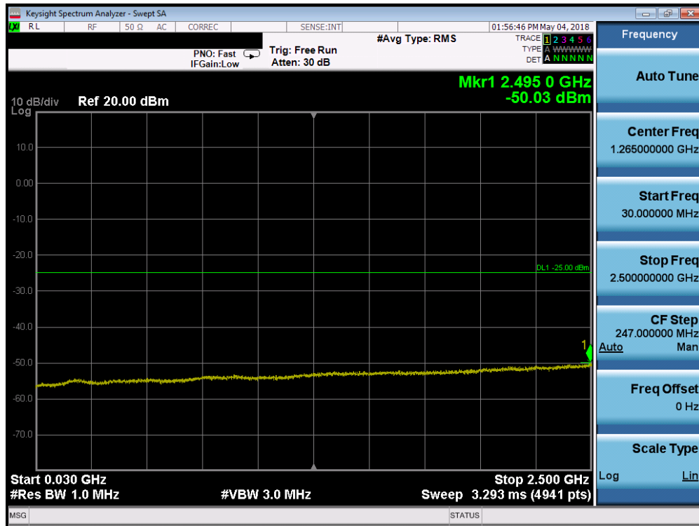
Plot 7-104. Conducted Spurious Plot (Band 7 - 10.0MHz QPSK - RB Size 1, RB Offset 0 - High Channel)
