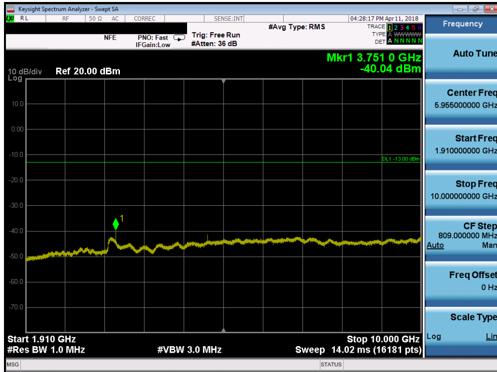
Plot 7-93. Conducted Spurious Plot (Band 2 - 10.0MHz QPSK - RB Size 1, RB Offset 0 - Mid Channel)
