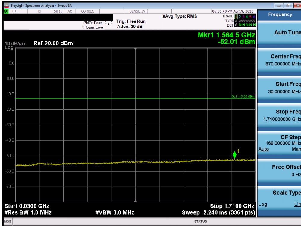
Plot 7-86. Conducted Spurious Plot (Band 66/4 - 10.0MHz QPSK - RB Size 1, RB Offset 0 - High Channel)
