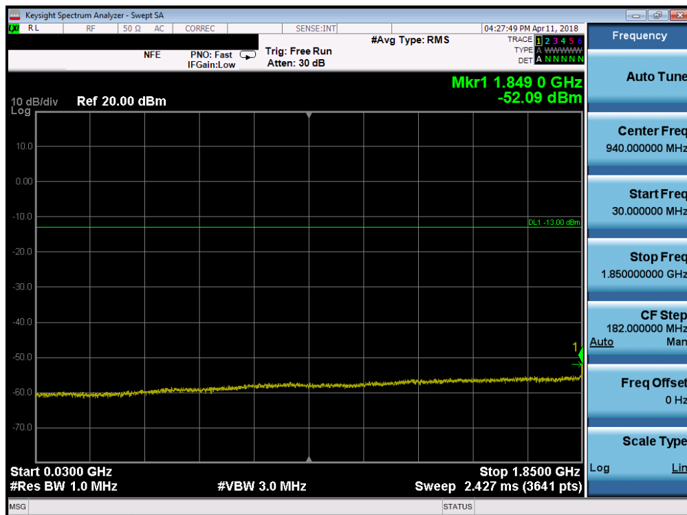
Plot 7-92. Conducted Spurious Plot (Band 2 - 10.0MHz QPSK - RB Size 1, RB Offset 0 - Mid Channel)
