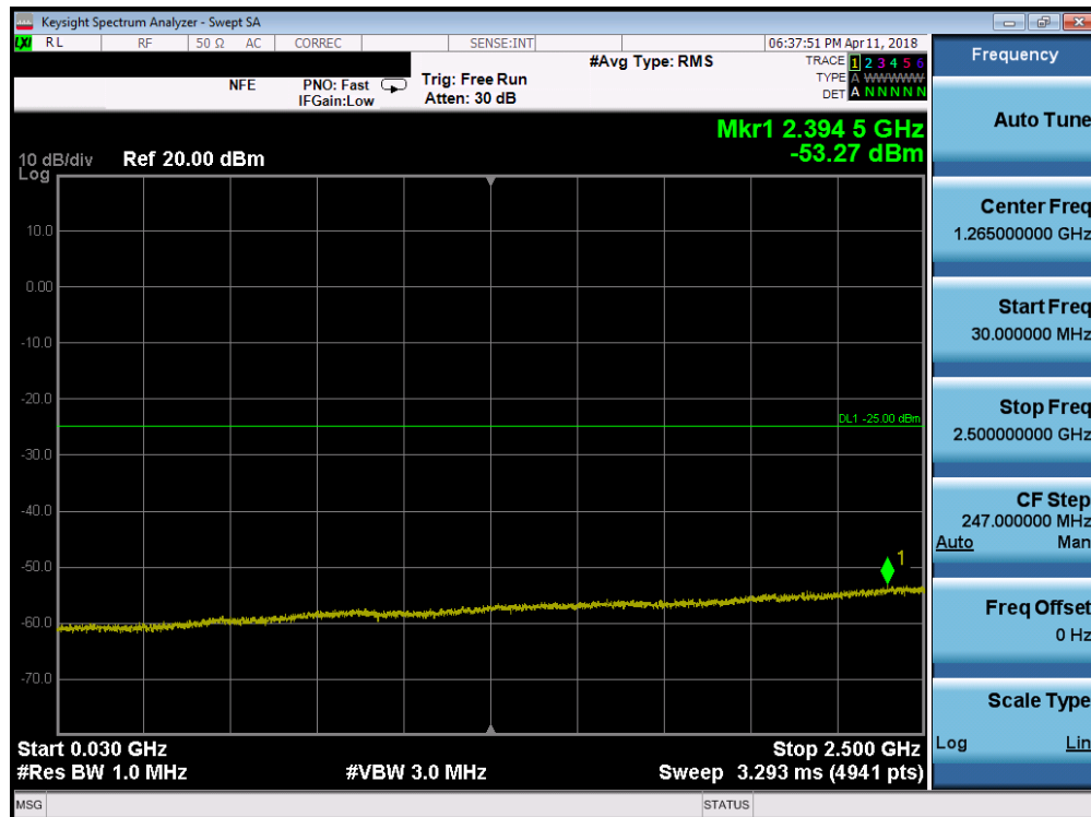
Plot 7-101. Conducted Spurious Plot (Band 7 - 10.0MHz QPSK - RB Size 1, RB Offset 0 - Mid Channel)
