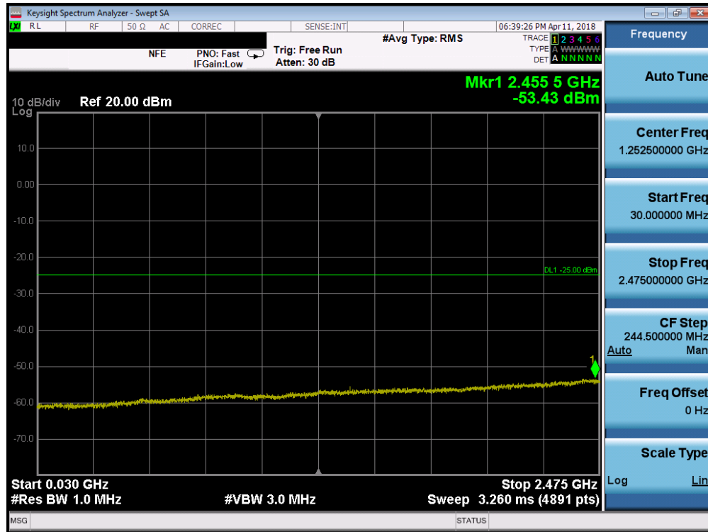
Plot 7-98. Conducted Spurious Plot (Band 7 - 10.0MHz QPSK - RB Size 1, RB Offset 0 - Low Channel)
