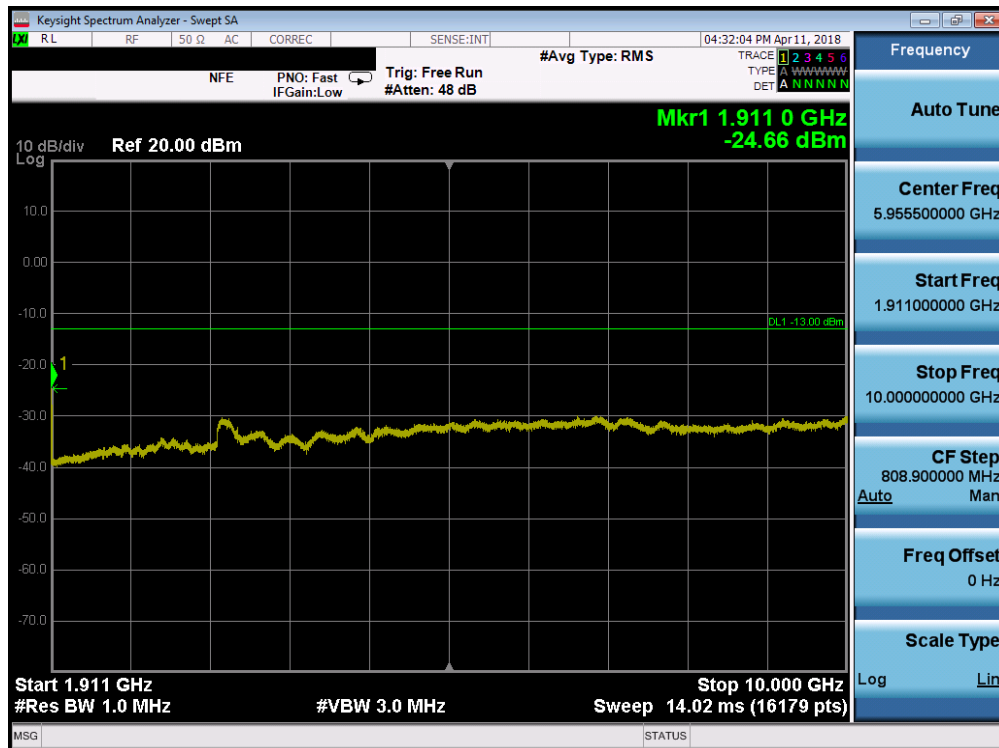
Plot 7-96. Conducted Spurious Plot (Band 2 - 10.0MHz QPSK - RB Size 1, RB Offset 0 - High Channel)
