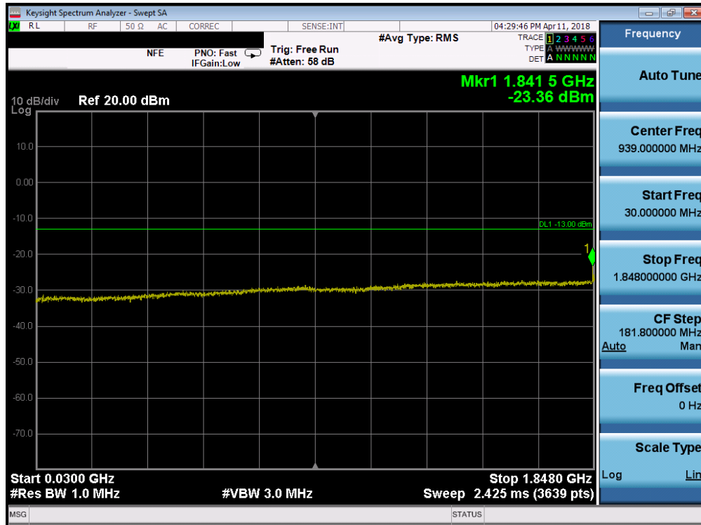
Plot 7-89. Conducted Spurious Plot (Band 2 - 10.0MHz QPSK - RB Size 1, RB Offset 0 - Low Channel)
