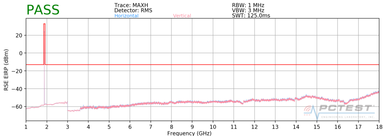
Plot 7-79. Radiated Spurious Plot above 1GHz (PCS GPRS)
