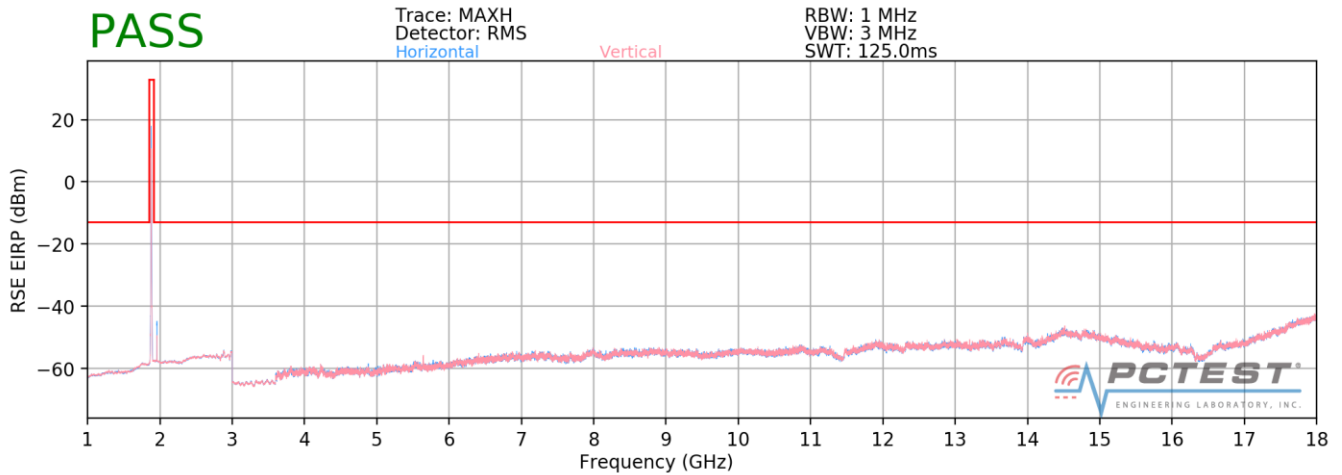
Plot 7-80. Radiated Spurious Plot above 1GHz (PCS WCDMA)
