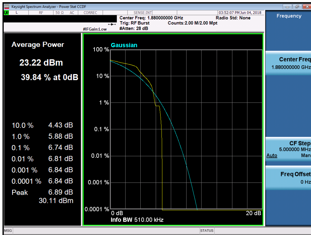
Plot 7-72. Peak-Average Ratio Plot (PCS EDGE Mode)
