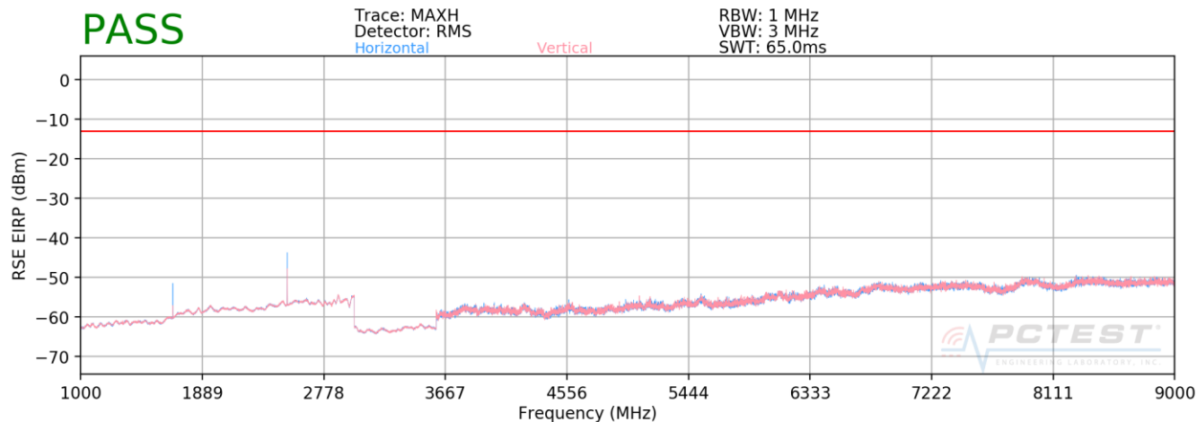
Plot 7-76. Radiated Spurious Plot above 1GHz (Cellular GPRS)
