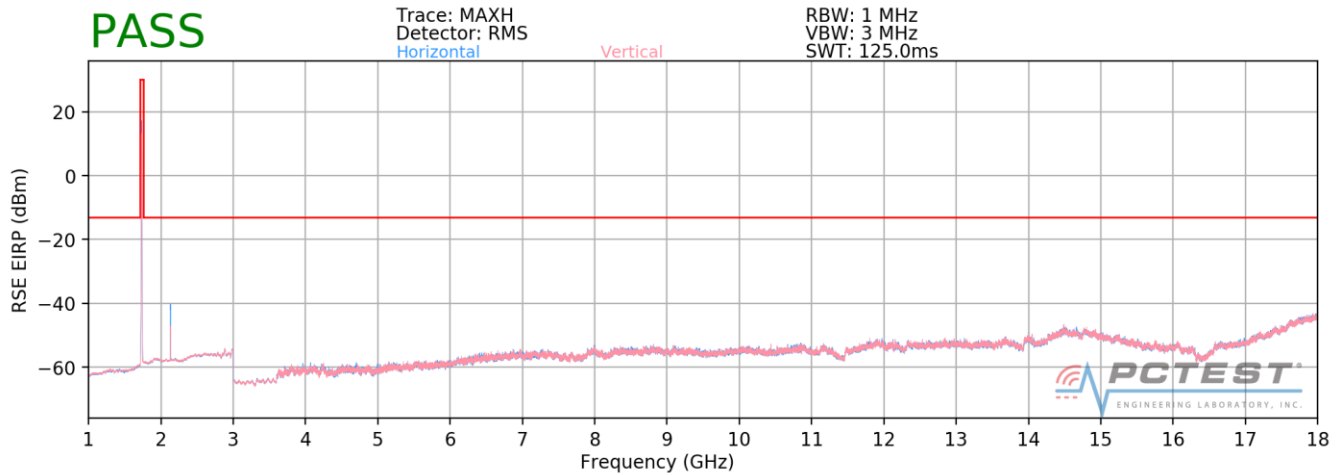
Plot 7-78. Radiated Spurious Plot above 1GHz (AWS WCDMA)
