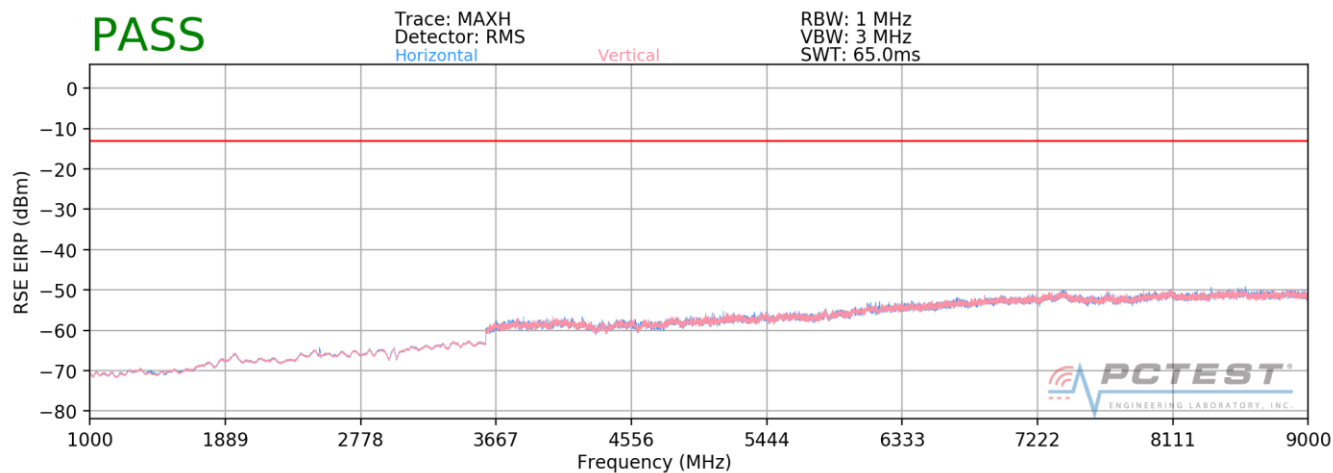
Plot 7-77. Radiated Spurious Plot above 1GHz (Cellular WCDMA)
