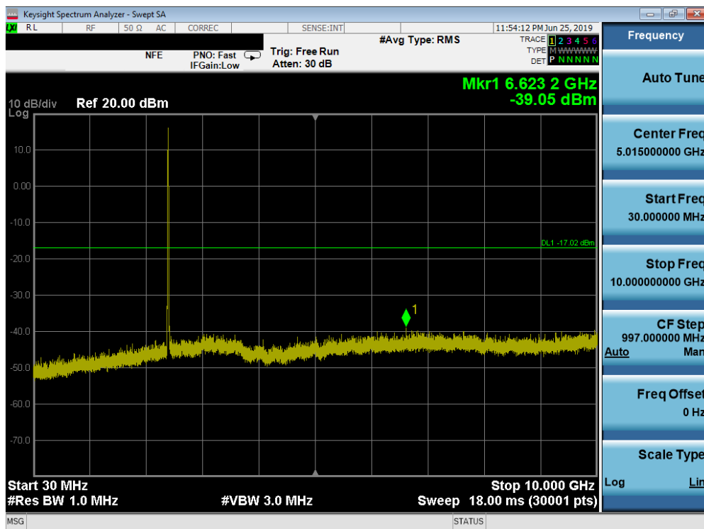
Plot 7-33. Conducted Spurious Plot (802.11b – Ch. 1)
