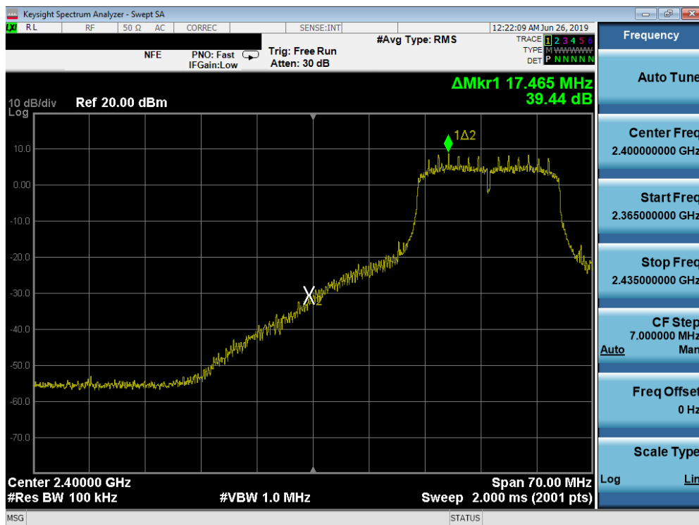
Plot 7-29. Band Edge Plot (802.11n (2.4GHz) – Ch. 3)
