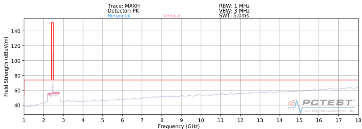
Plot 7-41. Radiated Spurious Plot above 1GHz (802.11b – Ch. 11)
