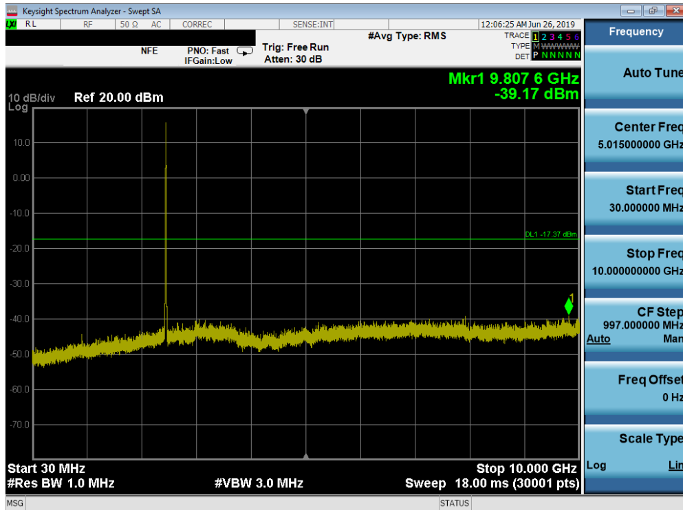
Plot 7-37. Conducted Spurious Plot (802.11b – Ch. 11)
