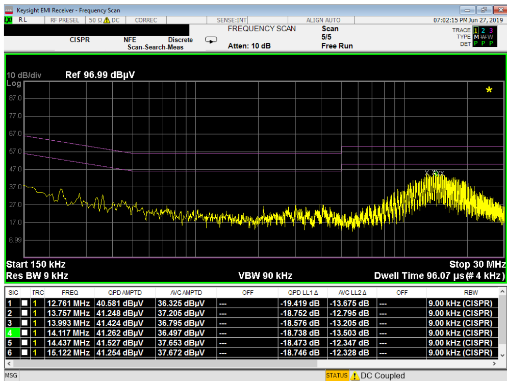
Plot 7-57. Line Conducted Plot with 802.11b (N)
