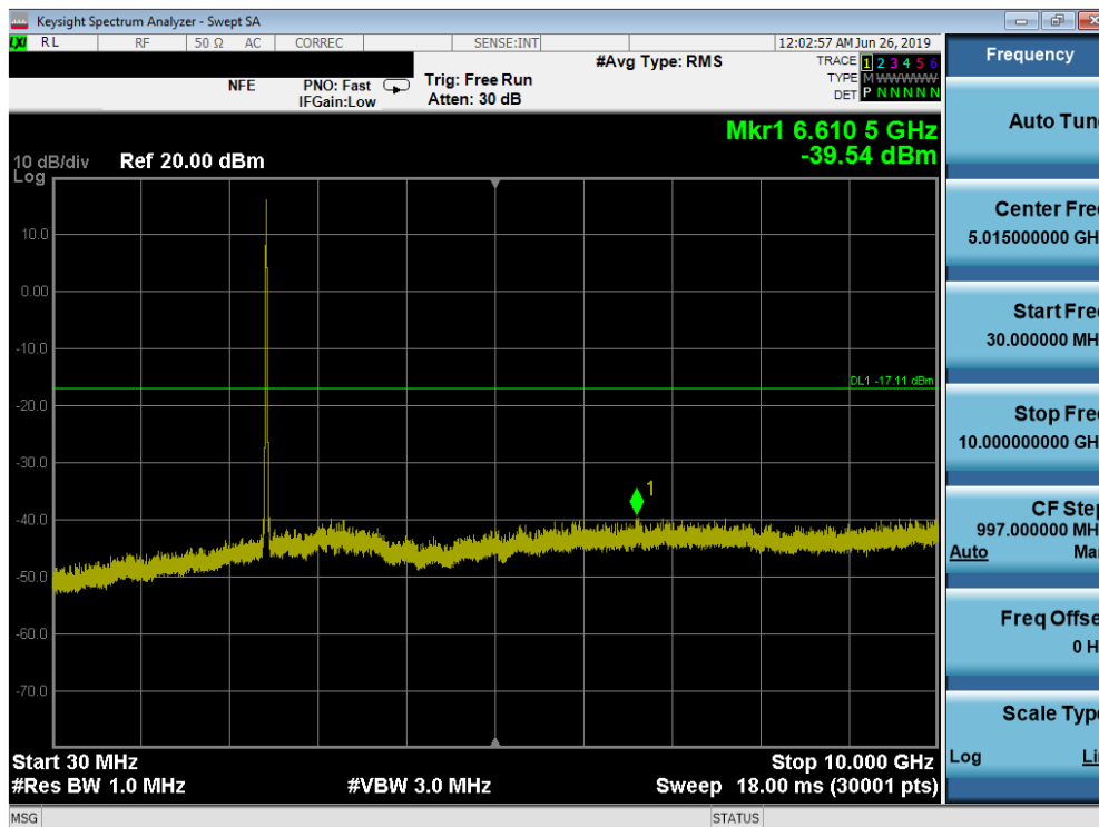
Plot 7-35. Conducted Spurious Plot (802.11b – Ch. 6)
