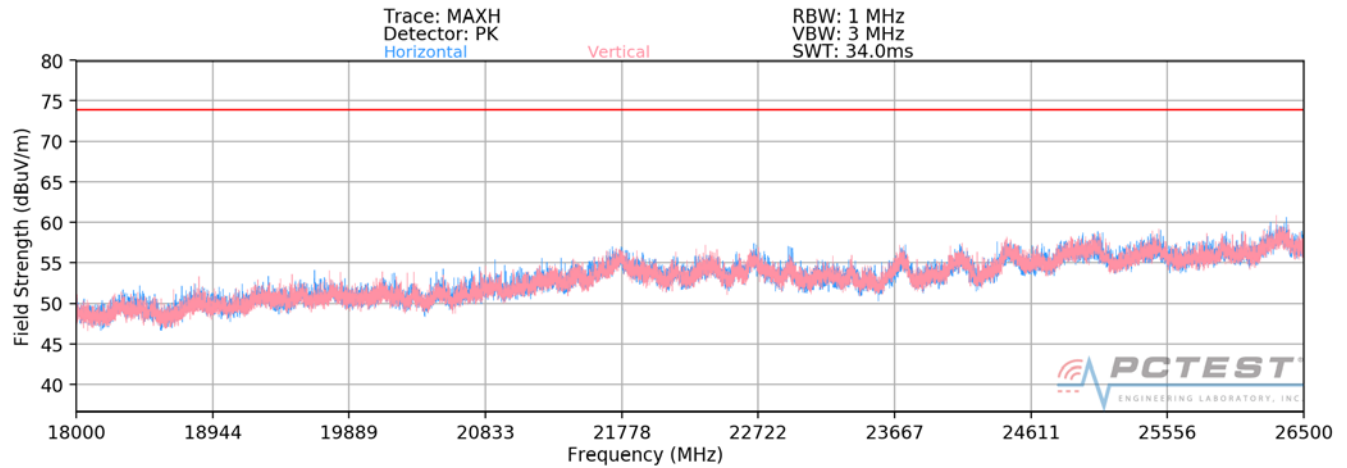
Plot 7-42. Radiated Spurious Plot above 18GHz
