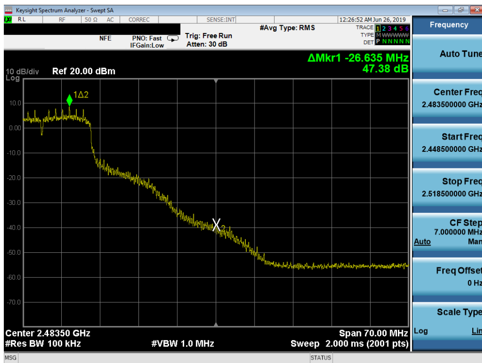
Plot 7-30. Band Edge Plot (802.11n (2.4GHz) – Ch. 9)
