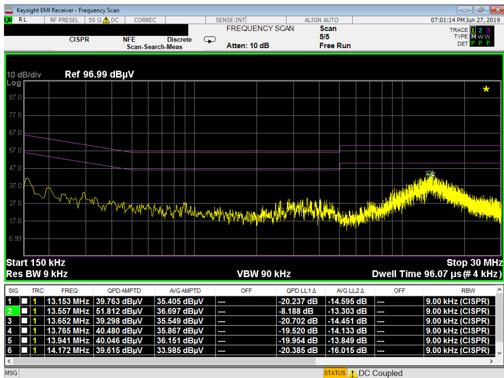
Plot 7-56. Line Conducted Plot with 802.11b (L1)
