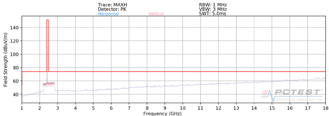
Plot 7-39. Radiated Spurious Plot above 1GHz (802.11b – Ch. 1)
