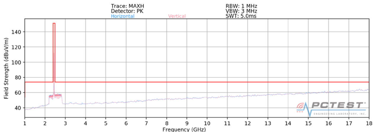
Plot 7-40. Radiated Spurious Plot above 1GHz (802.11b – Ch. 6)
