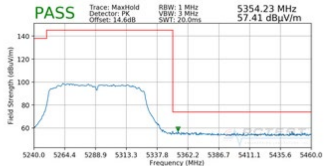
Plot 7-102. Radiated Upper Band Edge Plot (Peak – UNII Band 2A)
