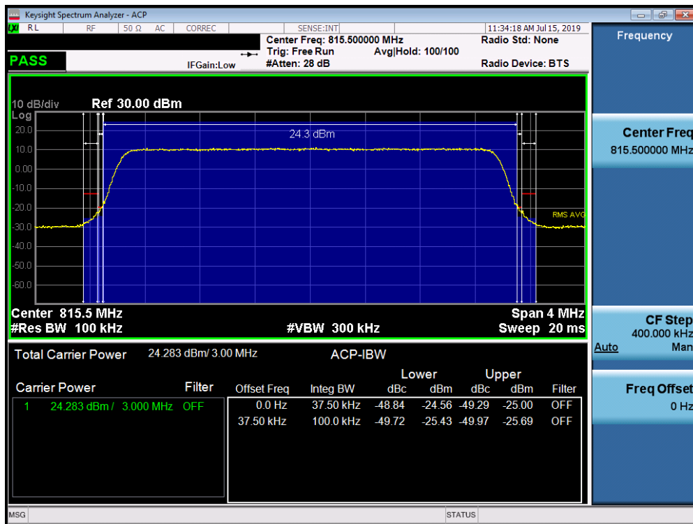
Plot 7-31. Channel Edge Plot (LTE Band 26, 3MHz QPSK – RB Size 15– Low Channel)
