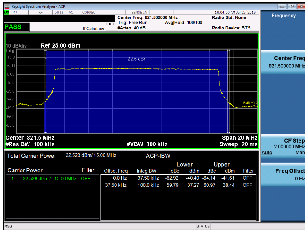
Plot 7-36. Channel Edge Plot (LTE Band 26, 15MHz QPSK – RB Size 75)
