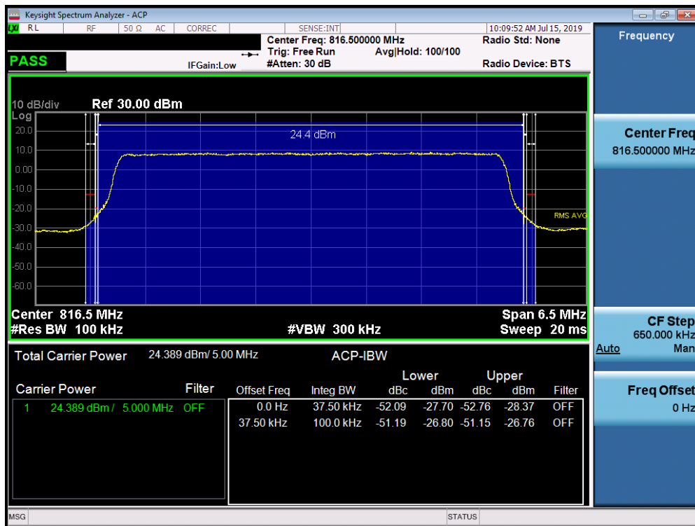
Plot 7-33. Channel Edge Plot (LTE Band 26, 5MHz QPSK – RB Size 25– Low Channel)
