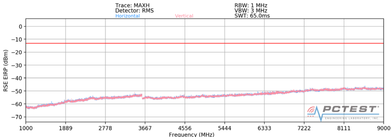
Plot 7-39. Radiated Spurious Plot above 1GHz (LTE Mode)
