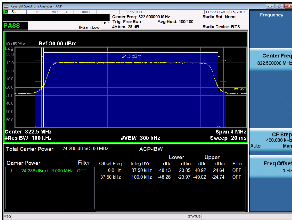
Plot 7-32. Channel Edge Plot (LTE Band 26, 3MHz QPSK – RB Size 15 – High Channel)
