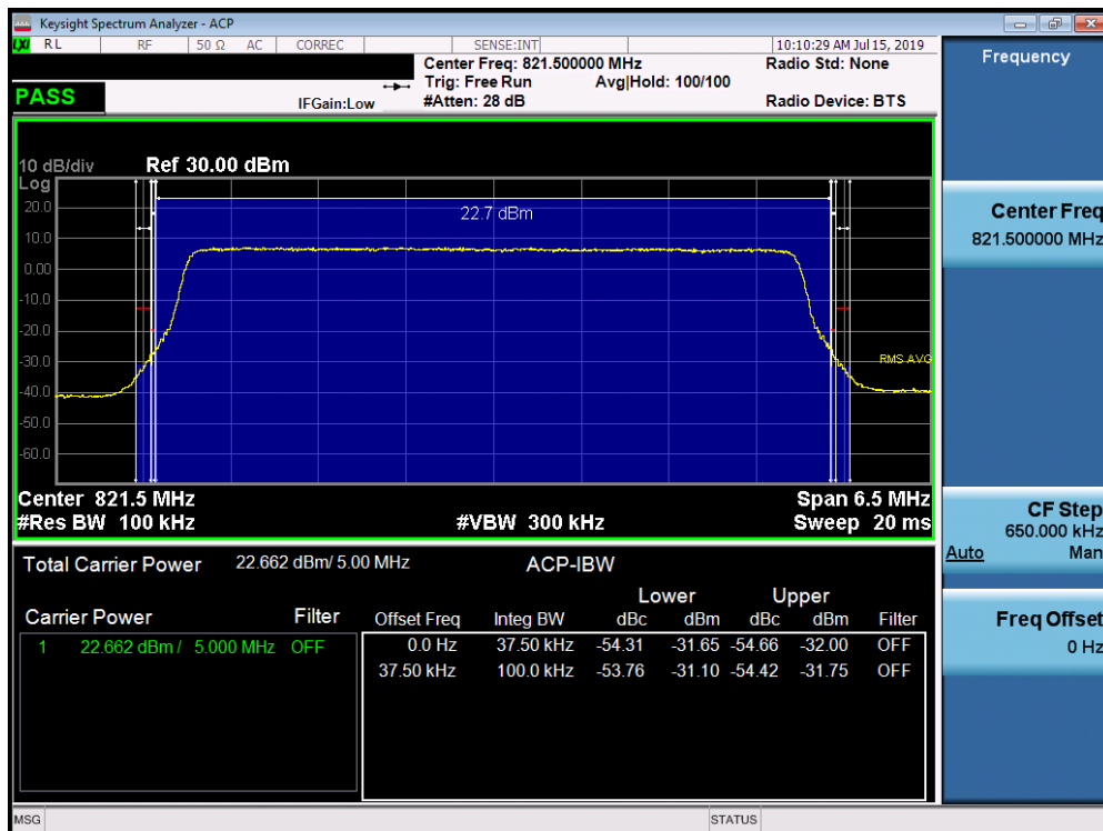
Plot 7-34. Channel Edge Plot (LTE Band 26, 5MHz QPSK – RB Size 25 – High Channel)
