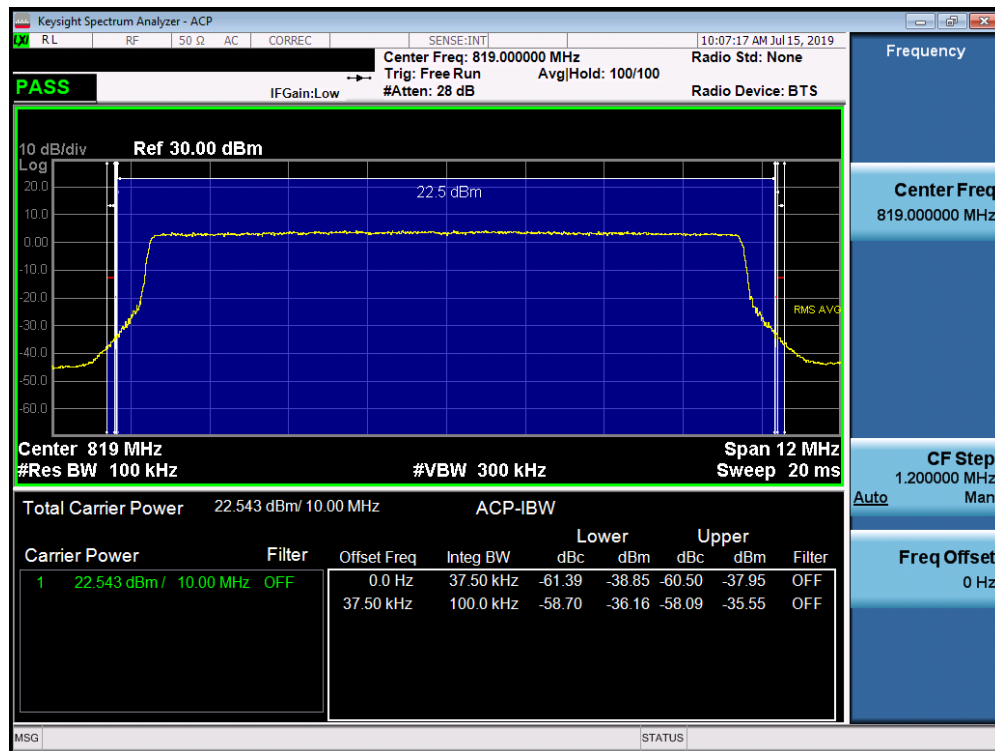
Plot 7-35. Channel Edge Plot (LTE Band 26, 10MHz QPSK – RB Size 50)
