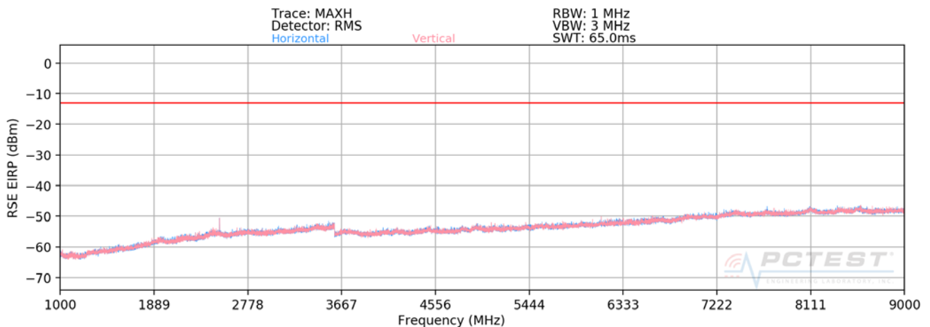
Plot 7-38. Radiated Spurious Plot above 1GHz (CDMA BC10 Mode)
