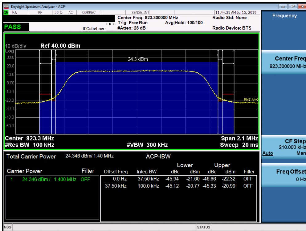
Plot 7-30. Channel Edge Plot (LTE Band 26, 1.4MHz QPSK – RB Size 6 – High Channel)
