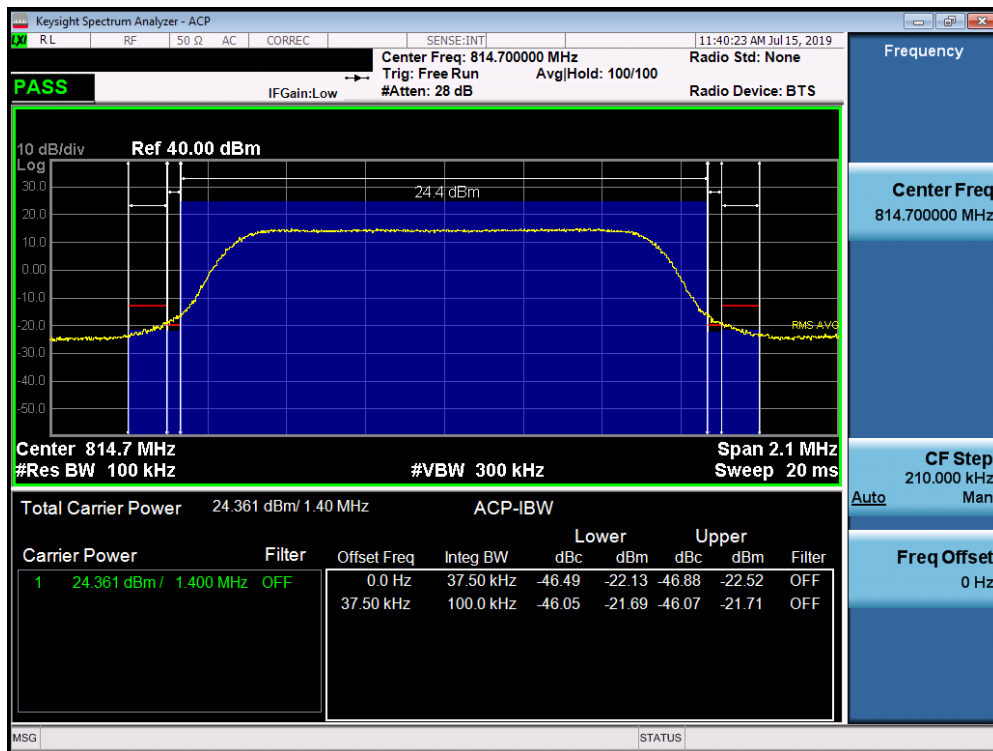
Plot 7-29. Channel Edge Plot (LTE Band 26, 1.4MHz QPSK – RB Size 6– Low Channel)
