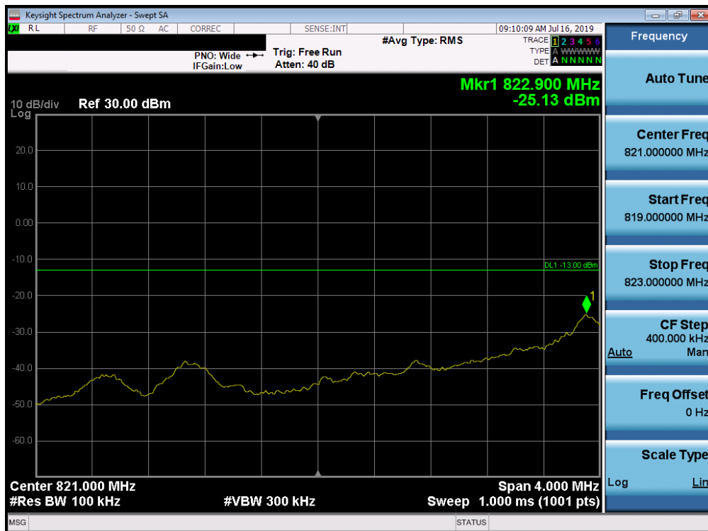
Plot 7-78. 4MHz Span Plot (Cellular CDMA Mode - Low Channel)
