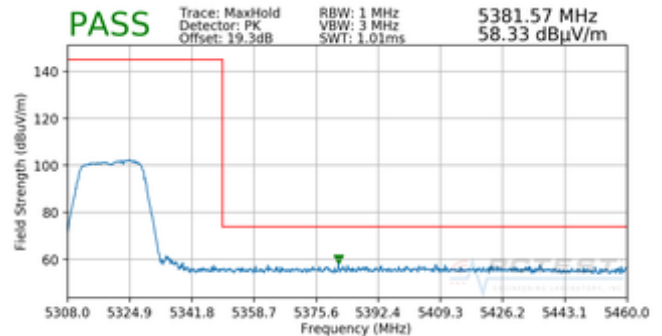
Plot 7-86. Radiated Upper Band Edge Plot (Peak – UNII Band 2A)
