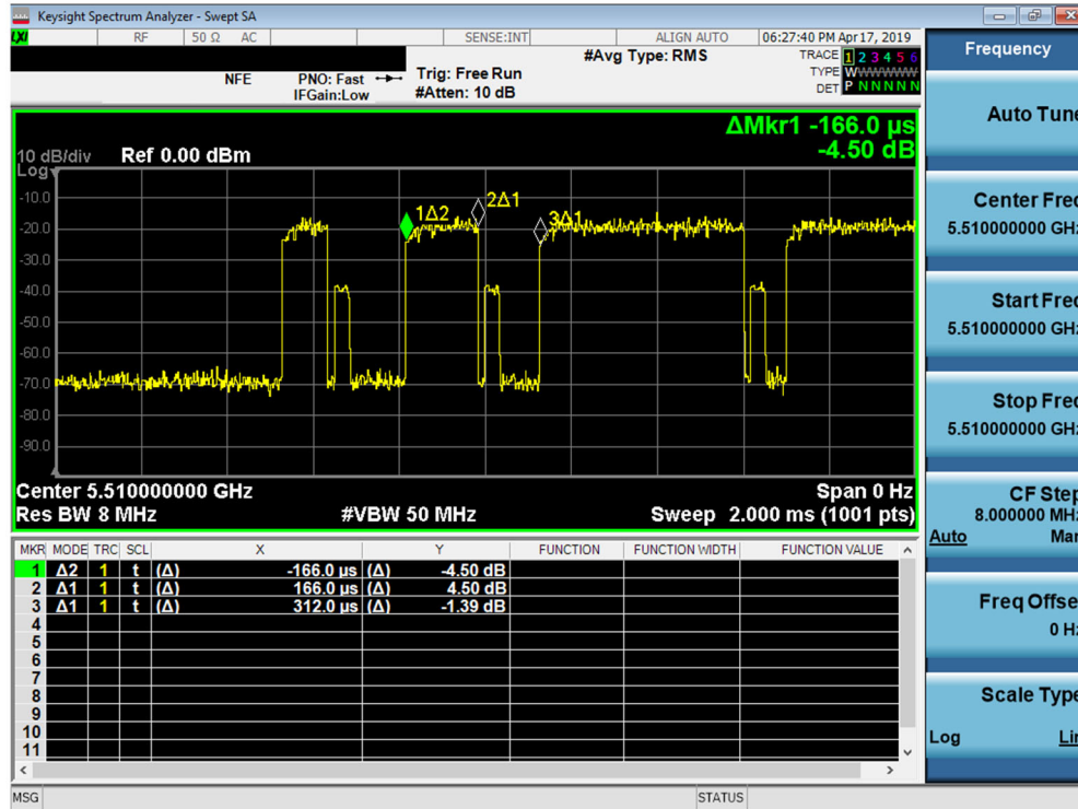
Figure 5-1. Band 2C Pulse Width / Period
