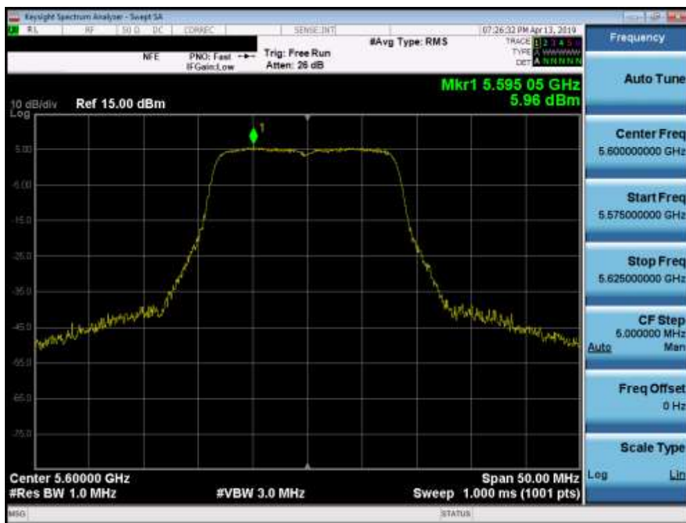
Plot 7-59. Power Spectral Density Plot (802.11a (UNII Band 2C) – Ch. 120)
