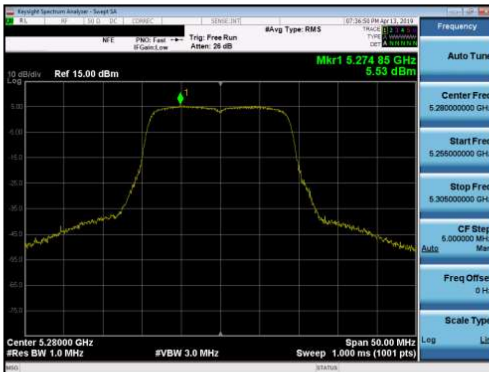
Plot 7-53. Power Spectral Density Plot (20MHz BW 802.11n (UNII Band 2A) – Ch. 56)
