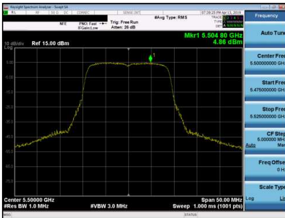
Plot 7-61. Power Spectral Density Plot (20MHz BW 802.11n (UNII Band 2C) – Ch. 100)
