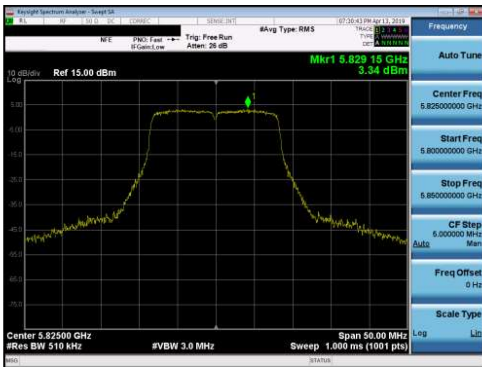
Plot 7-72. Power Spectral Density Plot (802.11a (UNII Band 3) – Ch. 165)
