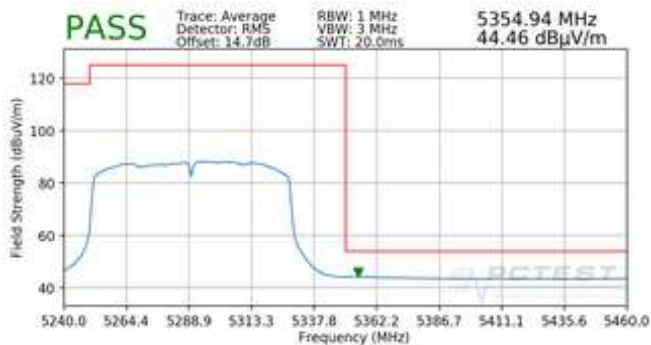
Plot 7-108. Radiated Upper Band Edge Plot (Average – UNII Band 2A)
