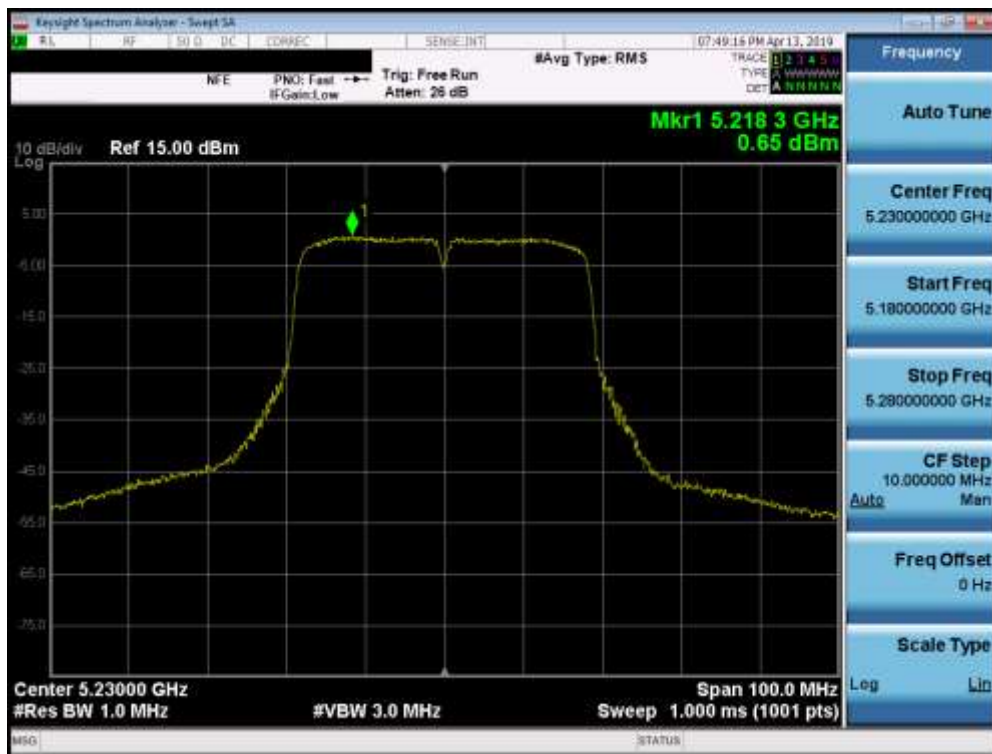
Plot 7-47. Power Spectral Density Plot (40MHz BW 802.11n (UNII Band 1) – Ch. 46)
