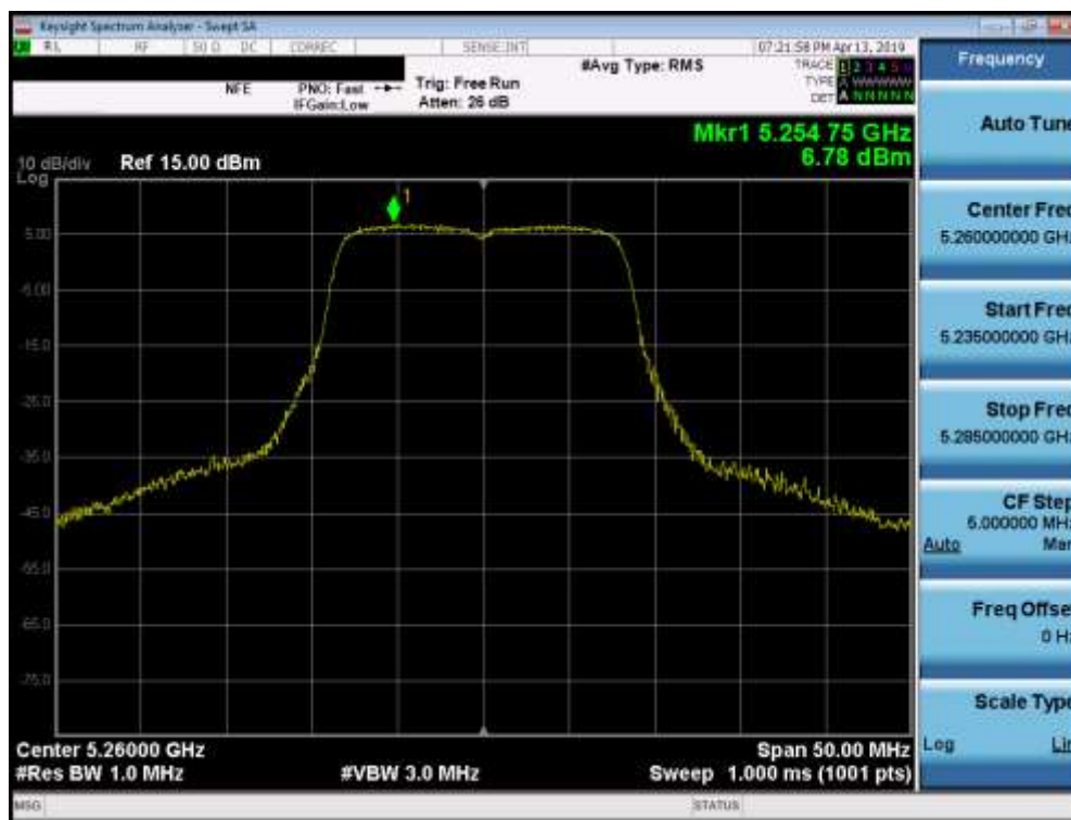
Plot 7-49. Power Spectral Density Plot (802.11a (UNII Band 2A) – Ch. 52)
