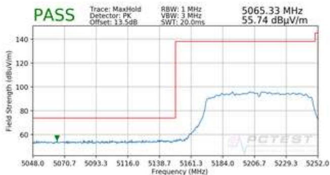
Plot 7-107. Radiated Lower Band Edge Plot (Peak – UNII Band 1)
