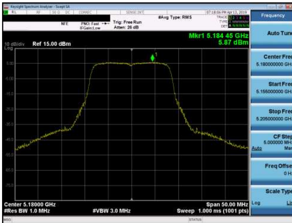
Plot 7-40. Power Spectral Density Plot (802.11a (UNII Band 1) – Ch. 36)
