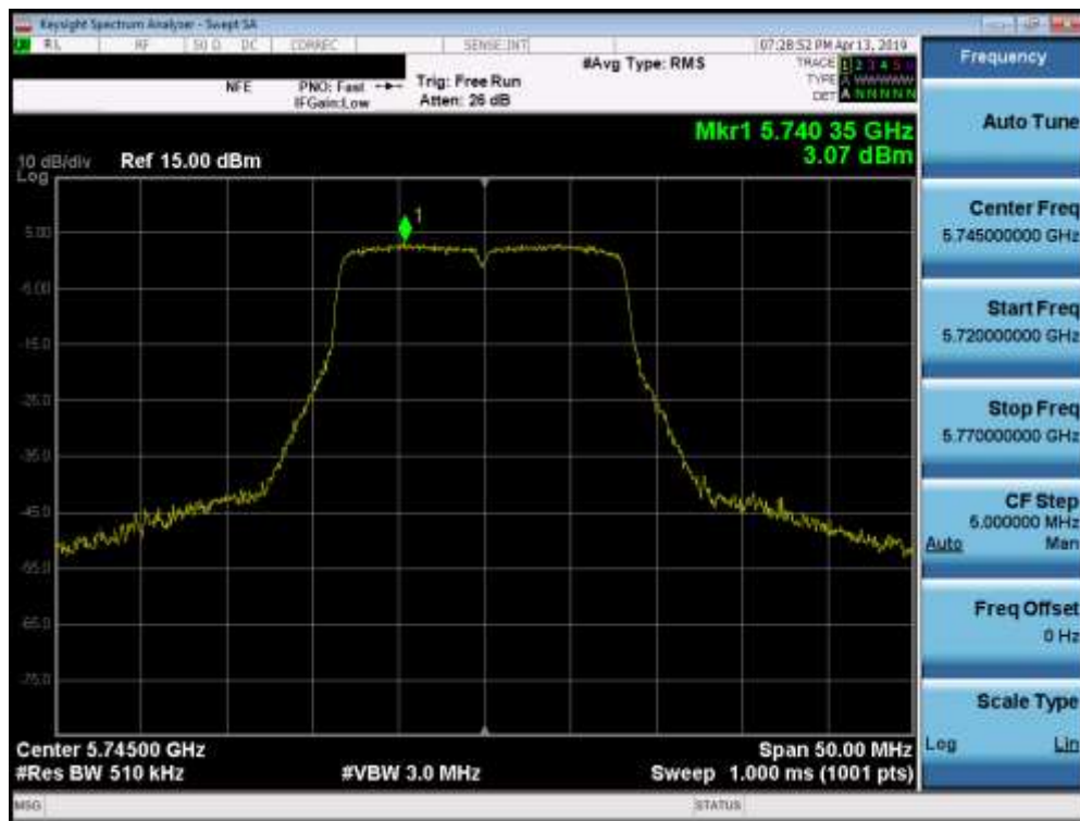
Plot 7-70. Power Spectral Density Plot (802.11a (UNII Band 3) – Ch. 149)
