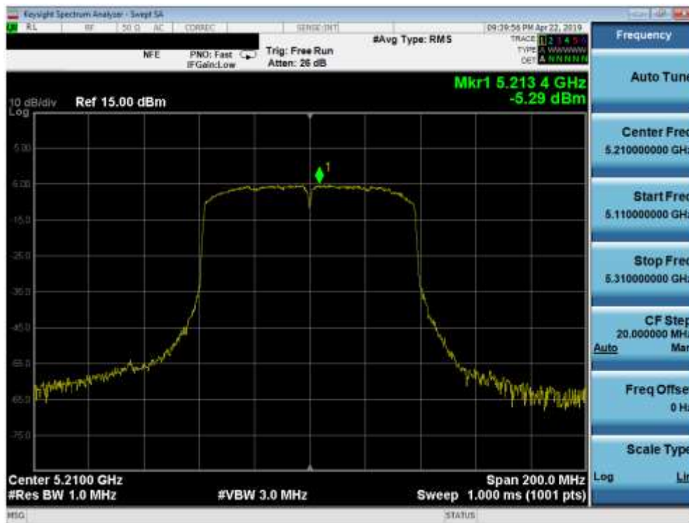
Plot 7-48. Power Spectral Density Plot (80MHz BW 802.11ac (UNII Band 1) – Ch. 42)
