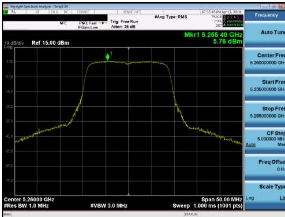
Plot 7-52. Power Spectral Density Plot (20MHz BW 802.11n (UNII Band 2A) – Ch. 52)
