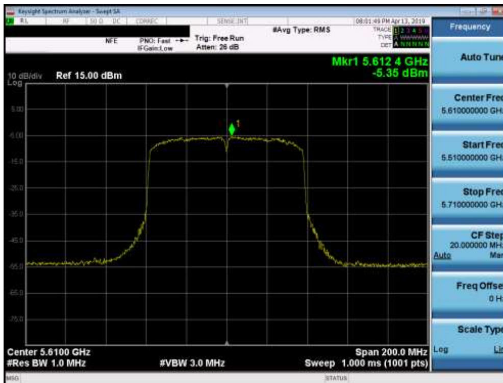
Plot 7-68. Power Spectral Density Plot (80MHz BW 802.11ac (UNII Band 2C) – Ch. 122)
