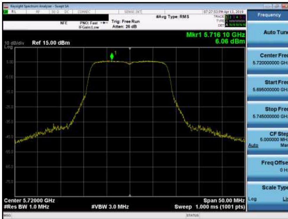
Plot 7-60. Power Spectral Density Plot (802.11a (UNII Band 2C) – Ch. 144)
