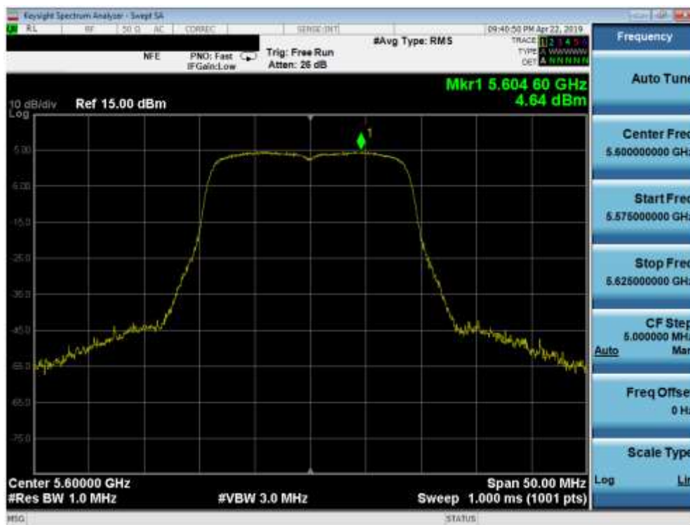
Plot 7-62. Power Spectral Density Plot (20MHz BW 802.11n (UNII Band 2C) – Ch. 120)
