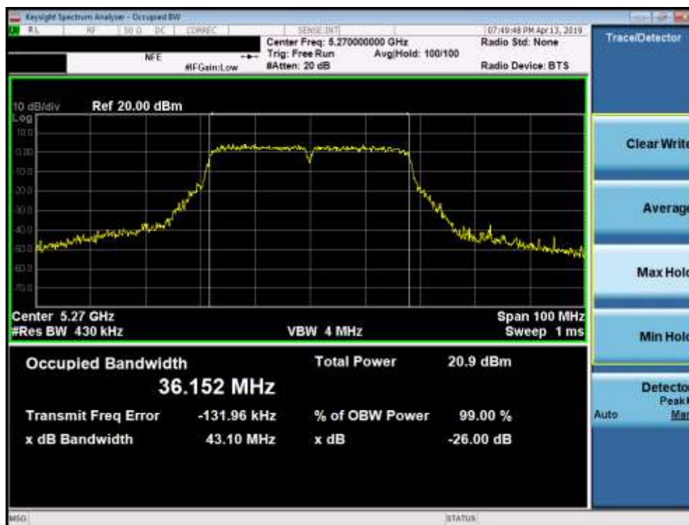
Plot 7-16. 26dB Bandwidth Plot (40MHz BW 802.11n (UNII Band 2A) – Ch. 54)
