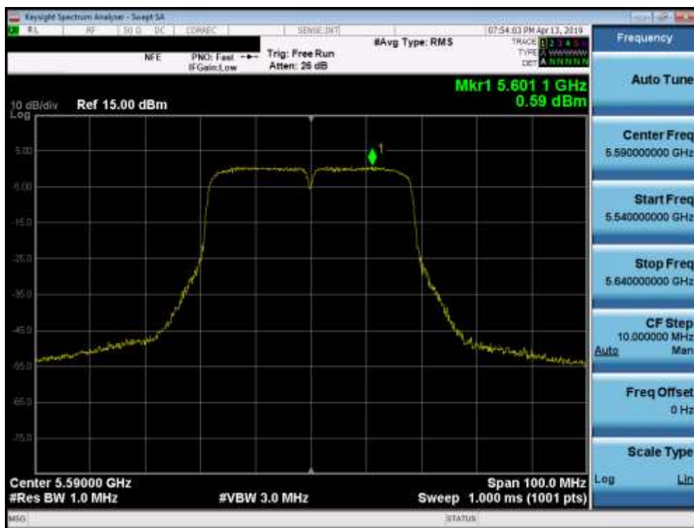
Plot 7-65. Power Spectral Density Plot (40MHz BW 802.11n (UNII Band 2C) – Ch. 118)
