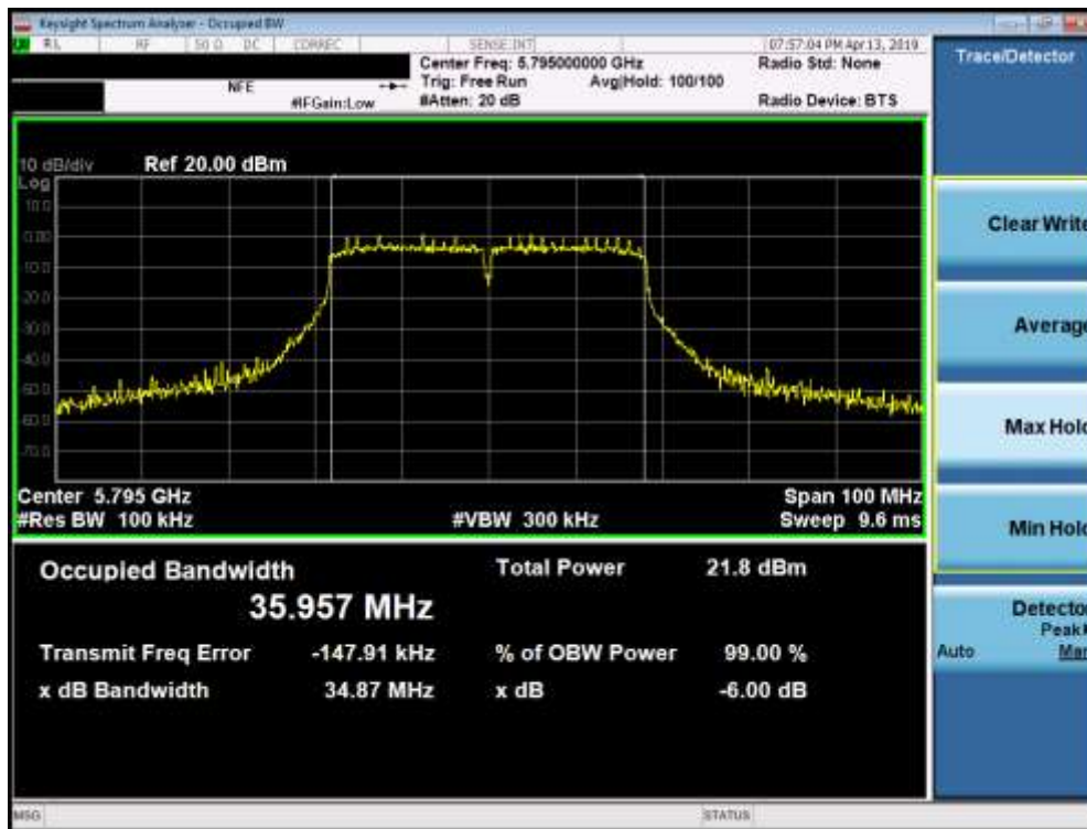
Plot 7-38. 6dB Bandwidth Plot (40MHz BW 802.11n (UNII Band 3) – Ch. 159)
