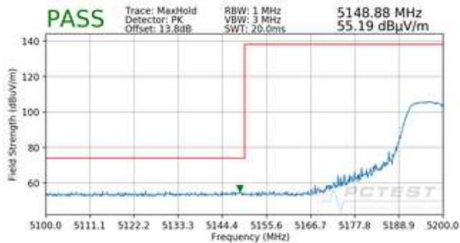
Plot 7-88. Radiated Lower Band Edge Plot (Peak – UNII Band 1)
