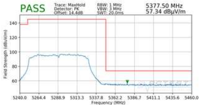
Plot 7-109. Radiated Upper Band Edge Plot (Peak – UNII Band 2A)
