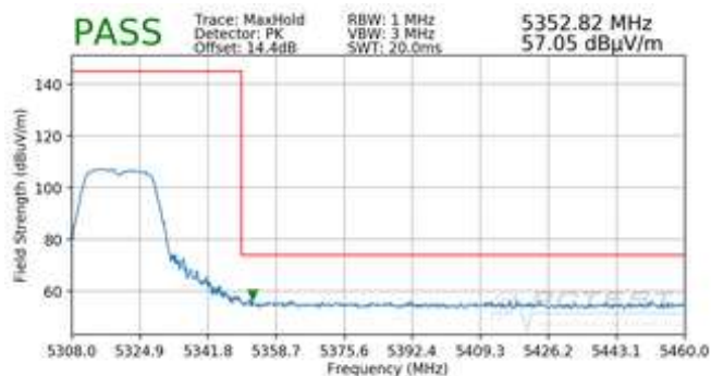
Plot 7-92. Radiated Upper Band Edge Plot (Peak – UNII Band 2A)
