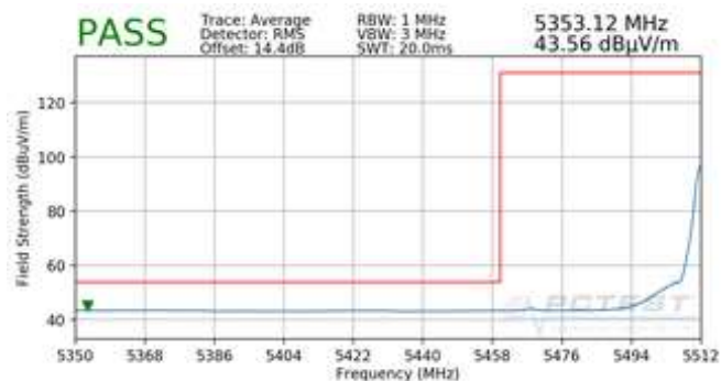
Plot 7-95. Radiated Lower Band Edge Plot (Average – UNII Band 2C)
