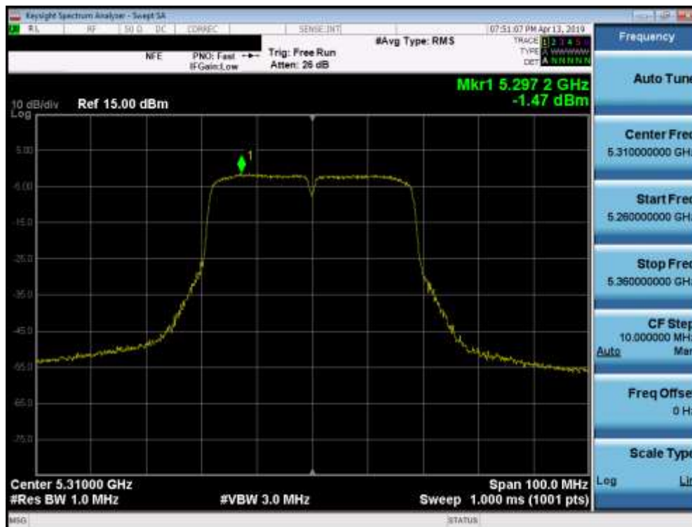
Plot 7-56. Power Spectral Density Plot (40MHz BW 802.11n (UNII Band 2A) – Ch. 62)
