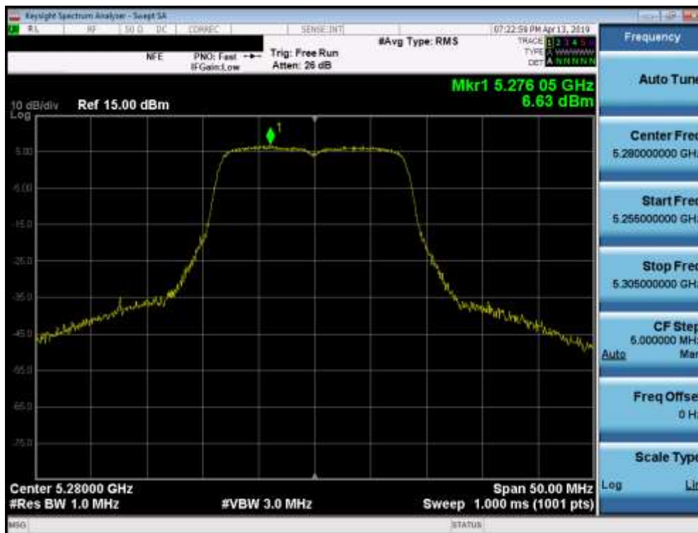
Plot 7-50. Power Spectral Density Plot (802.11a (UNII Band 2A) – Ch. 56)
