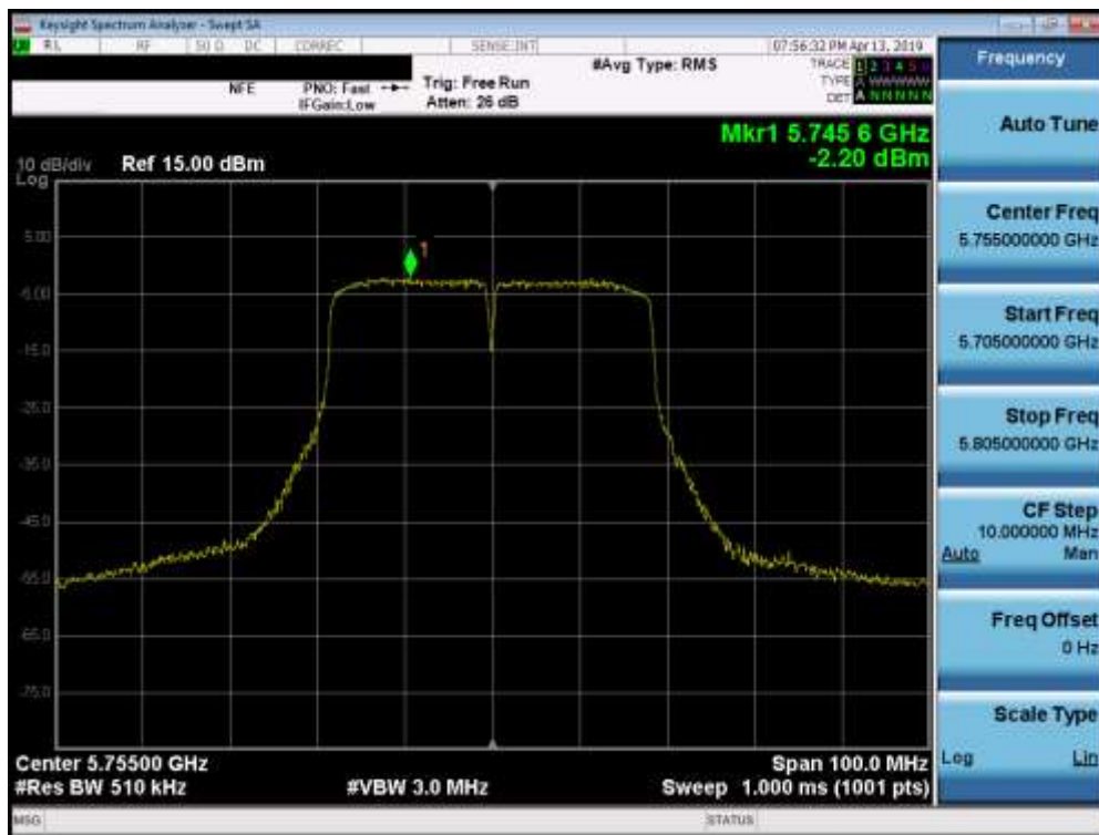
Plot 7-76. Power Spectral Density Plot (40MHz BW 802.11n (UNII Band 3) – Ch. 151)
