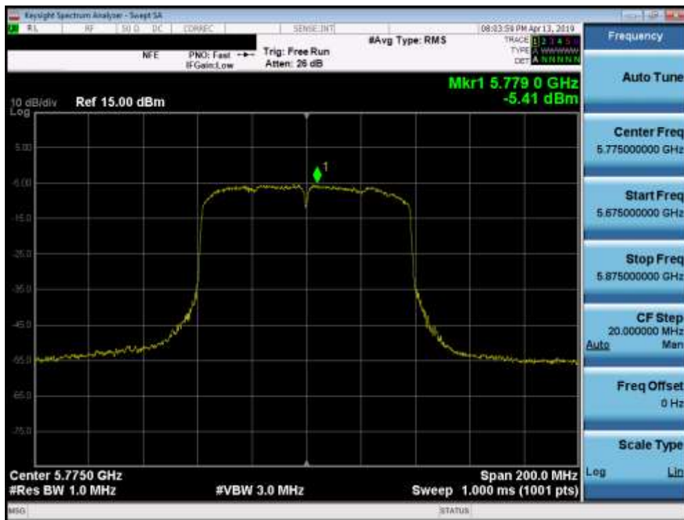
Plot 7-78. Power Spectral Density Plot (80MHz BW 802.11ac (UNII Band 3) – Ch. 155)
