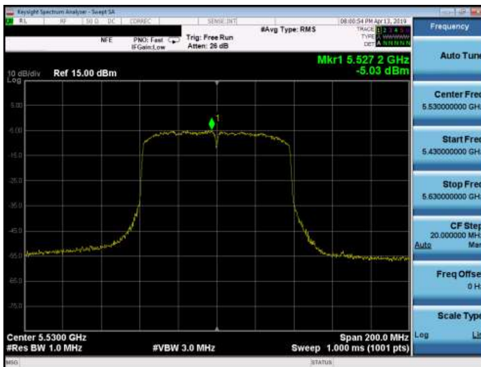
Plot 7-67. Power Spectral Density Plot (80MHz BW 802.11ac (UNII Band 2C) – Ch. 106)
