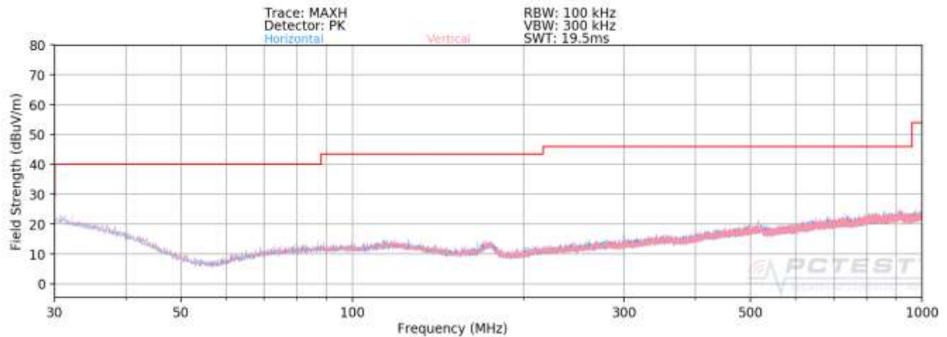
Plot 7-113. Radiated Spurious Plot below 1GHz (802.11a – U3 Ch. 157)
