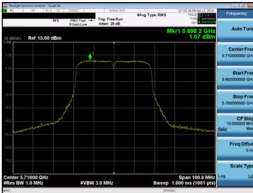
Plot 7-66. Power Spectral Density Plot (40MHz BW 802.11n (UNII Band 2C) – Ch. 142)
