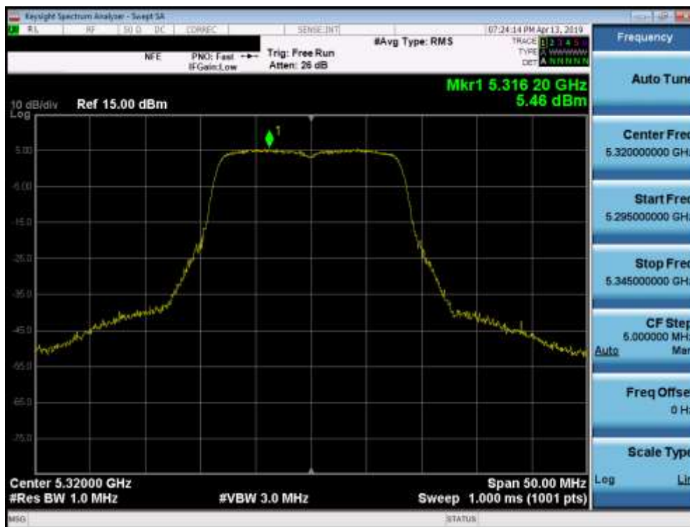
Plot 7-51. Power Spectral Density Plot (802.11a (UNII Band 2A) – Ch. 64)
