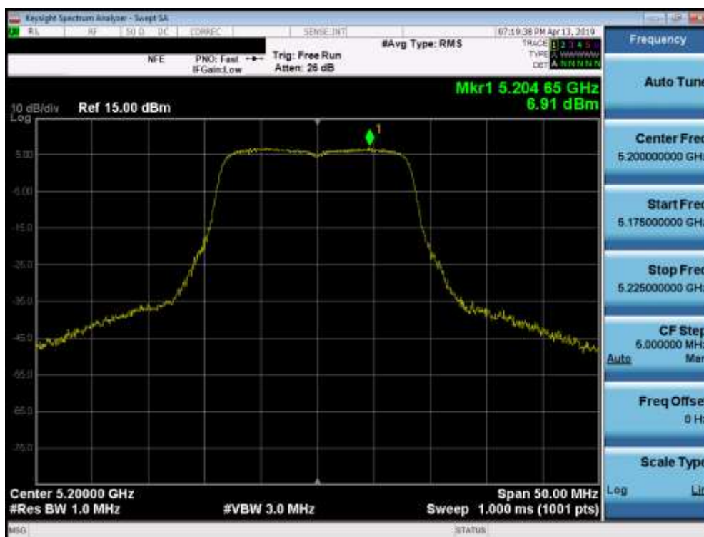
Plot 7-41. Power Spectral Density Plot (802.11a (UNII Band 1) – Ch. 40)
