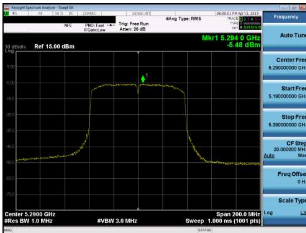
Plot 7-57. Power Spectral Density Plot (80MHz BW 802.11ac (UNII Band 2A) – Ch. 58)
