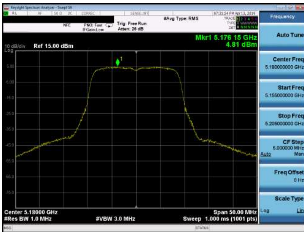
Plot 7-43. Power Spectral Density Plot (20MHz BW 802.11n (UNII Band 1) – Ch. 36)
