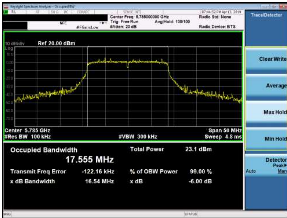
Plot 7-35. 6dB Bandwidth Plot (20MHz BW 802.11n (UNII Band 3) – Ch. 157)
