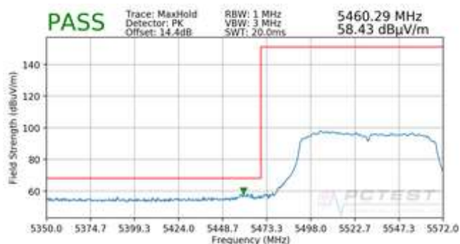
Plot 7-111. Radiated Lower Band Edge Plot (Peak – UNII Band 2C)
