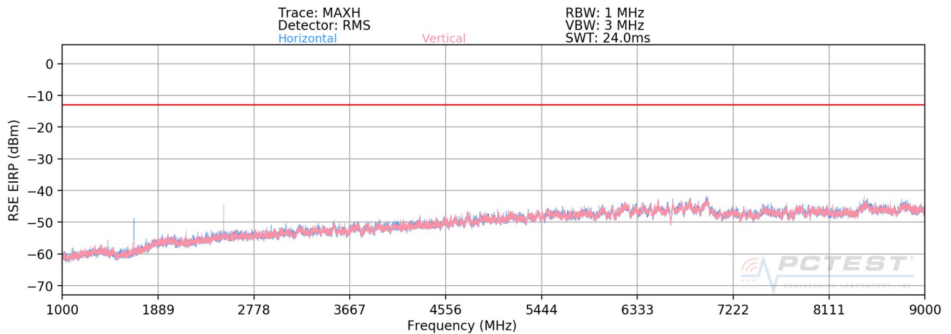
Plot 7-28. Radiated Spurious Plot above 1GHz (Band 26)
