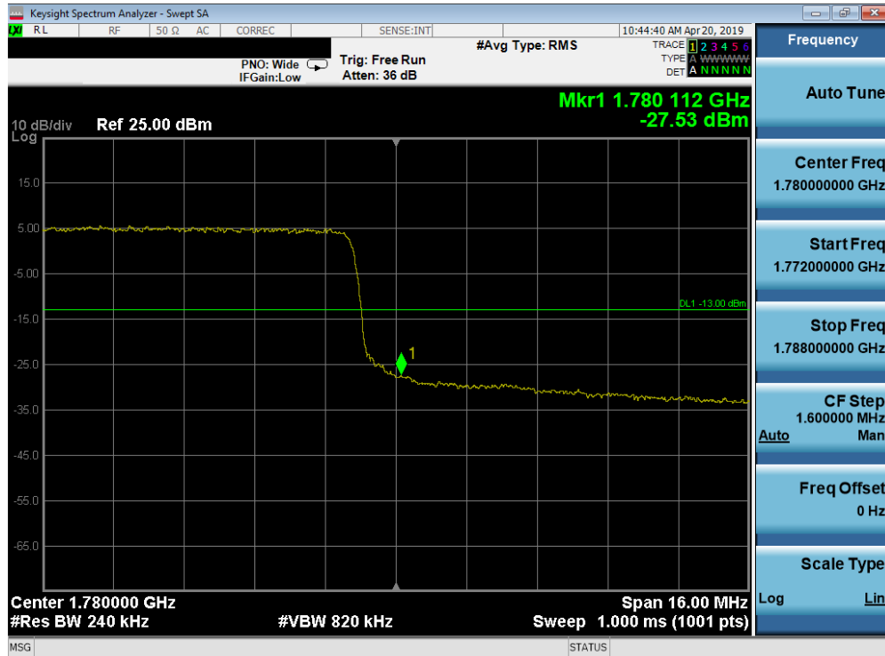
Plot 7-224. Upper Band Edge Plot (Band 66 - 20.0MHz QPSK - Full RB Configuration)
