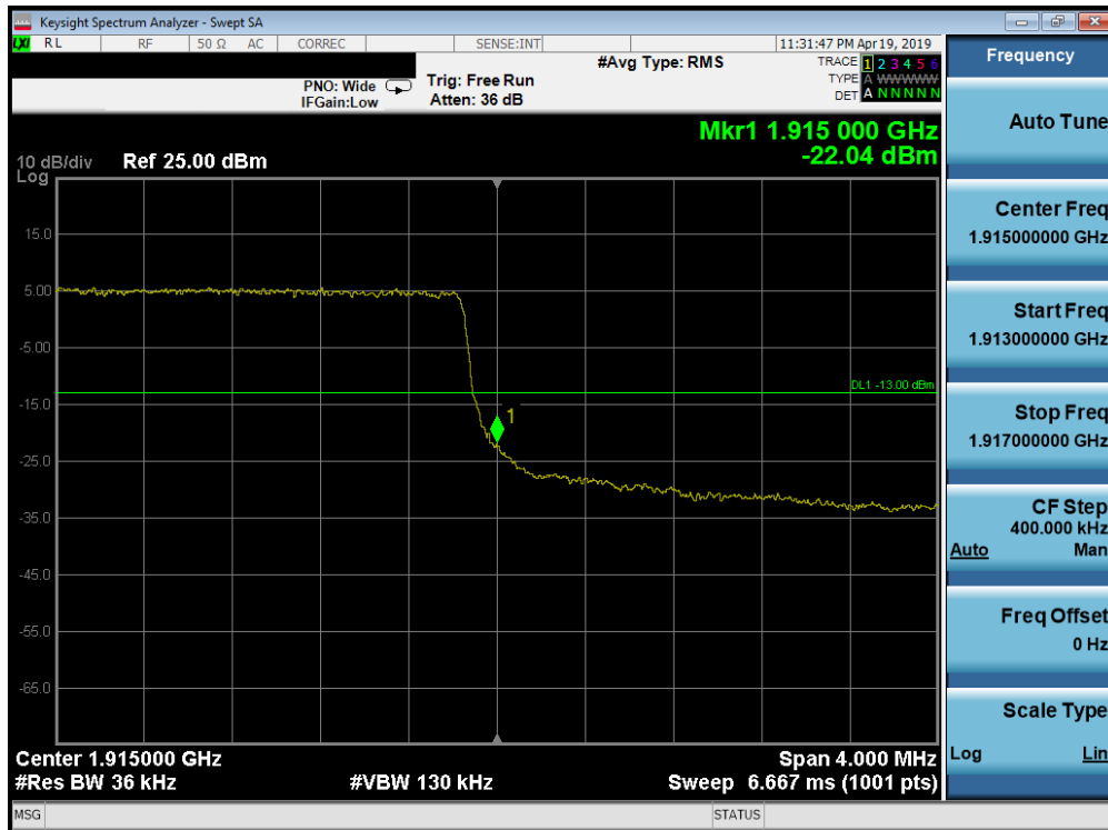
Plot 7-236. Upper Band Edge Plot (Band 25 - 3.0MHz QPSK - Full RB Configuration)
