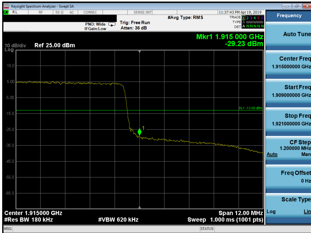
Plot 7-254. Upper Band Edge Plot (Band 25 - 15.0MHz QPSK - Full RB Configuration)
