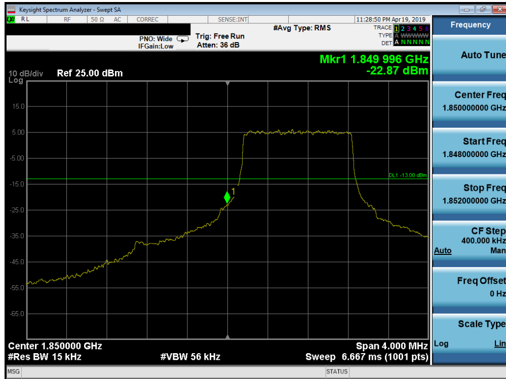
Plot 7-226. Lower Band Edge Plot (Band 25/2 - 1.4MHz QPSK - Full RB Configuration)
