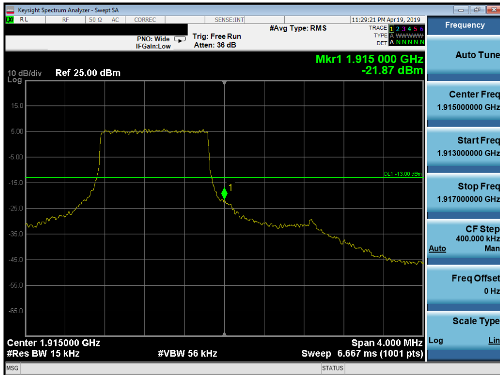
Plot 7-230. Upper Band Edge Plot (Band 25 - 1.4MHz QPSK - Full RB Configuration)
