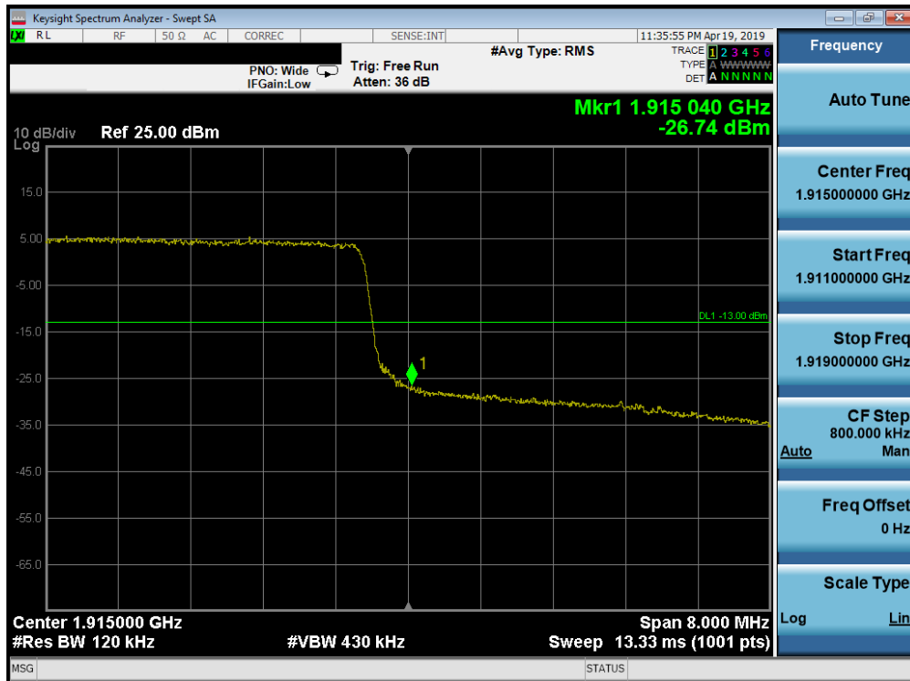
Plot 7-248. Upper Band Edge Plot (Band 25 - 10.0MHz QPSK - Full RB Configuration)
