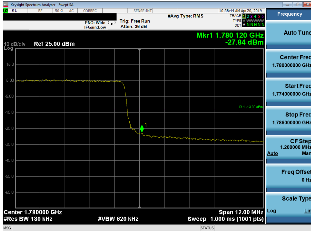
Plot 7-218. Upper Band Edge Plot (Band 66 - 15.0MHz QPSK - Full RB Configuration)
