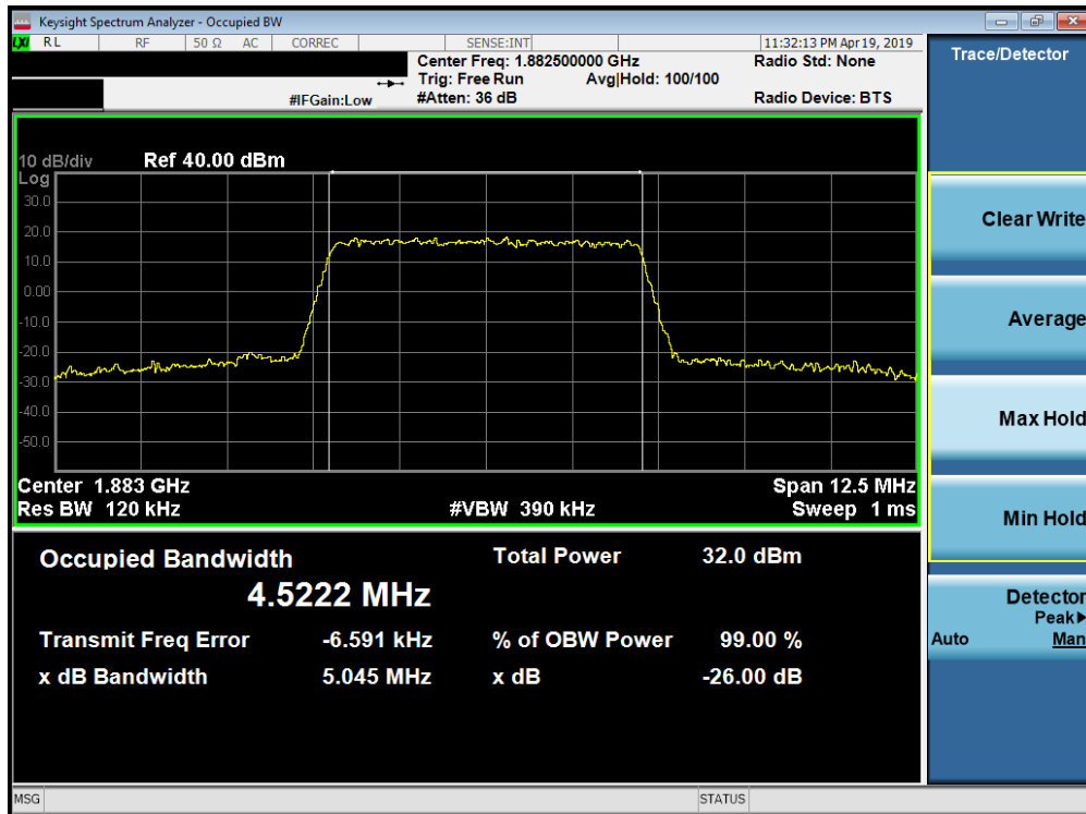
Plot 7-64. Occupied Bandwidth Plot (Band 25/2 - 5.0MHz QPSK - Full RB Configuration)
