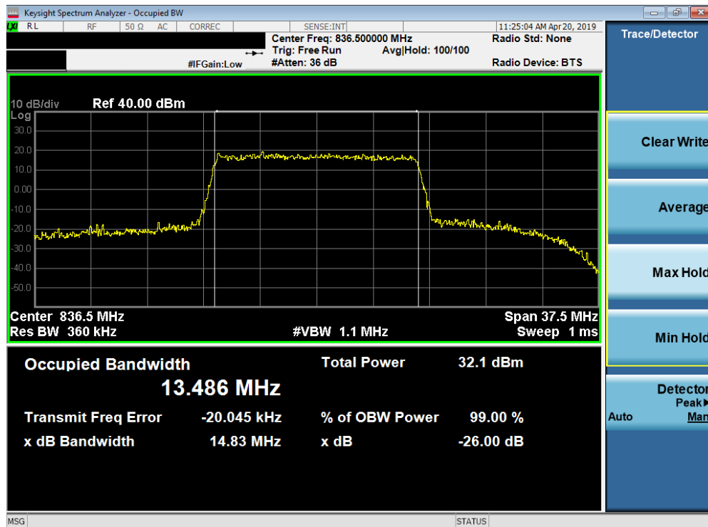
Plot 7-38. Occupied Bandwidth Plot (Band 26 - 15.0MHz 16-QAM - Full RB Configuration)
