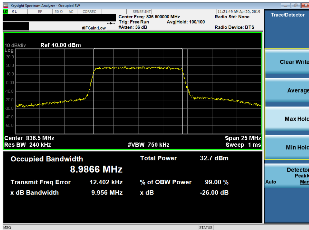
Plot 7-34. Occupied Bandwidth Plot (Band 26/5 - 10.0MHz QPSK - Full RB Configuration)
