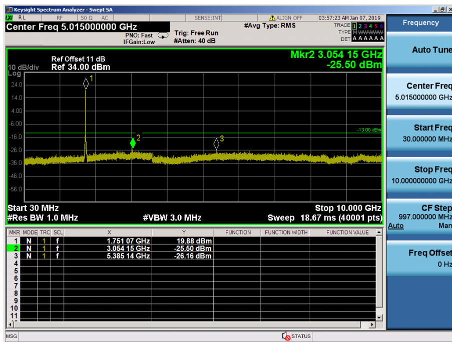
LTE Band 66, 4 / 20MHz / 64QAM - RB Size/Offset (100/0)–Mid Channel
