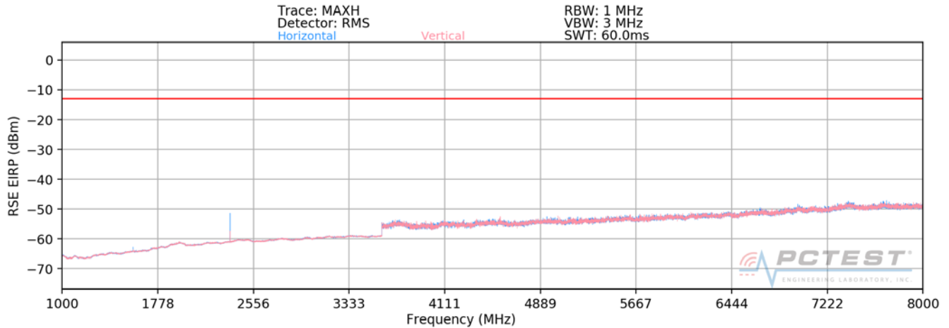
Plot 7-17. Radiated Spurious Plot above 1GHz (Band 14)
