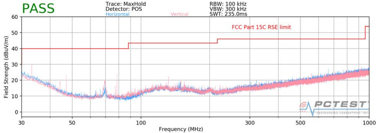
Plot 7-39. Radiated Spurious Plot below 1GHz (802.11b)
