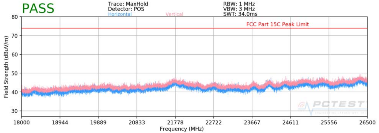
Plot 7-34. Radiated Spurious Plot above 18GHz (802.11b)
