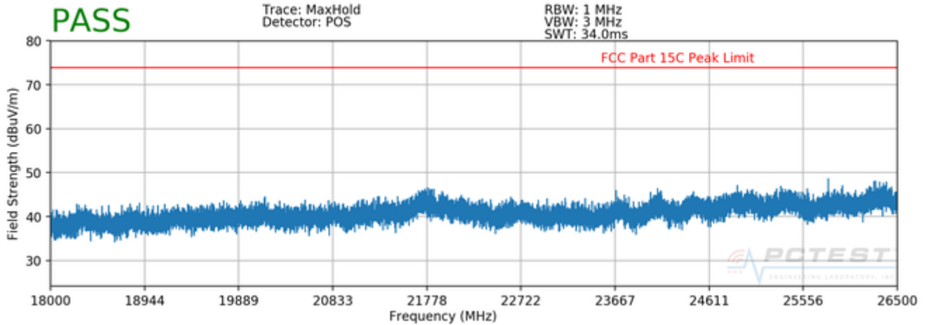
Plot 7-46. Radiated Spurious Plot above 18GHz (V)
