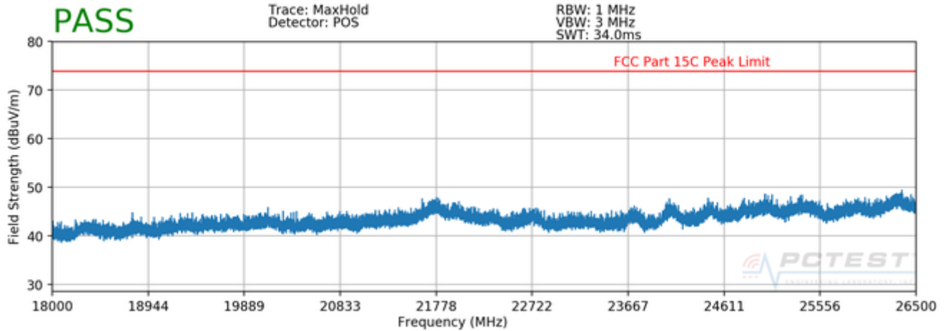
Plot 7-45. Radiated Spurious Plot above 18GHz (H)
