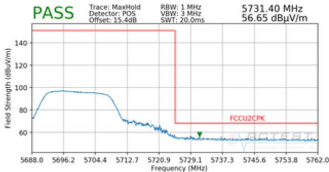
Plot 7-80. Radiated Upper Band Edge Plot (Peak – UNII Band 2C)
