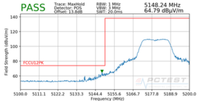
Plot 7-75. Radiated Lower Band Edge Plot (Peak – UNII Band 1)
