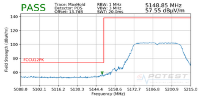
Plot 7-84. Radiated Lower Band Edge Plot (Peak – UNII Band 1)
