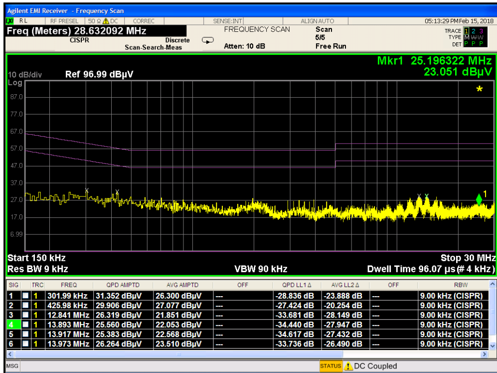
Plot 8-1. Line Conducted Plot with 802.11a UNII Band 1 (L1)
