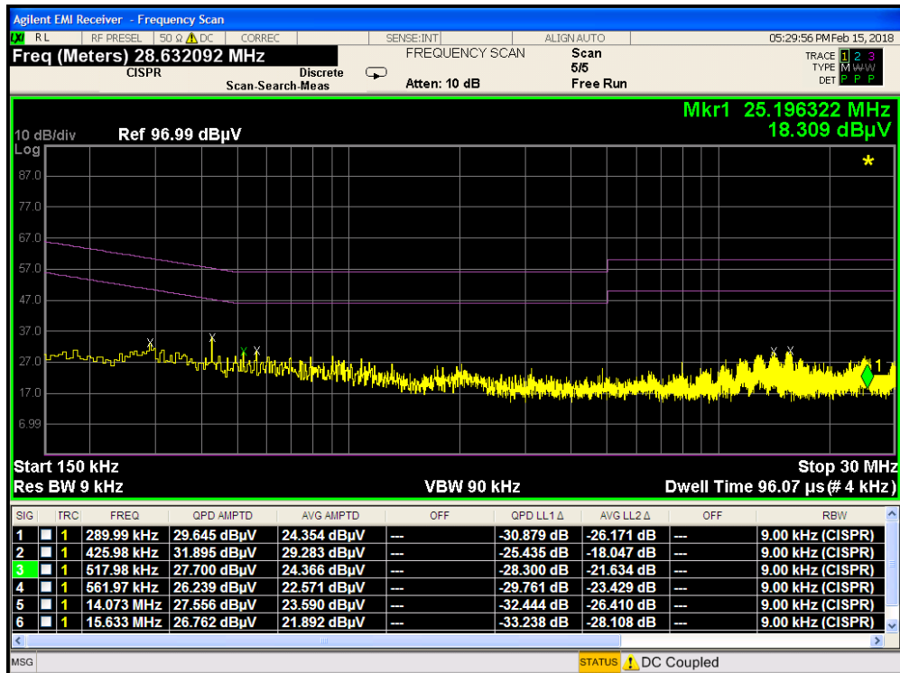
Plot 8-6. Line Conducted Plot with 802.11a UNII Band 2C (N)
