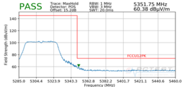
Plot 7-86. Radiated Upper Band Edge Plot (Peak – UNII Band 2A)
