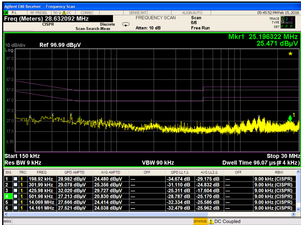
Plot 8-8. Line Conducted Plot with 802.11a UNII Band 3 (N)
