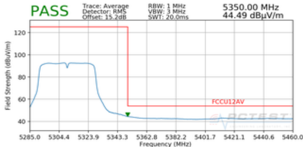
Plot 7-85. Radiated Upper Band Edge Plot (Average – UNII Band 2A)
