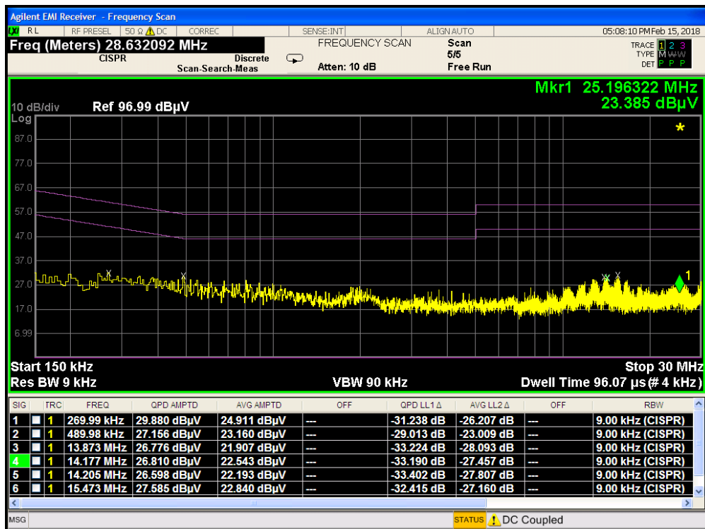
Plot 8-2. Line Conducted Plot with 802.11a UNII Band 1 (N)
