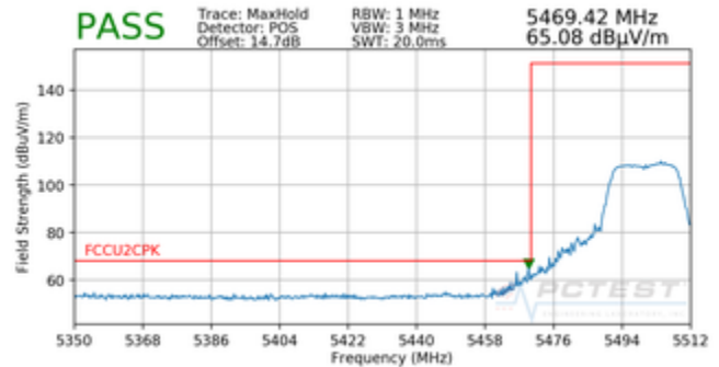
Plot 7-79. Radiated Lower Band Edge Plot (Peak – UNII Band 2C)
