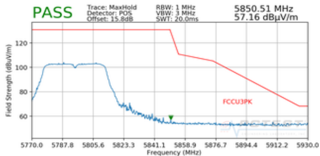
Plot 7-91. Radiated Upper Band Edge Plot (Peak – UNII Band 3)
