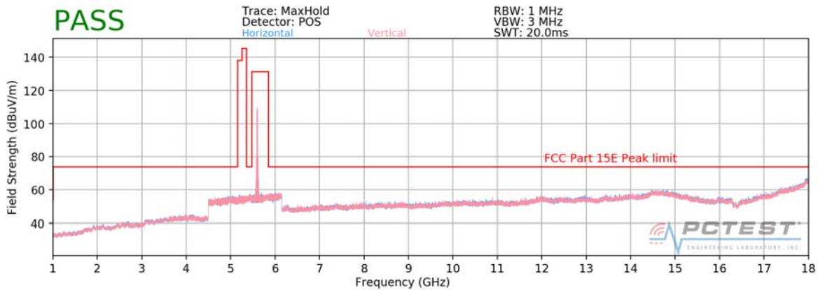
Plot 7-69. Radiated Spurious Plot above 1GHz (802.11a – U2C Ch. 120)
