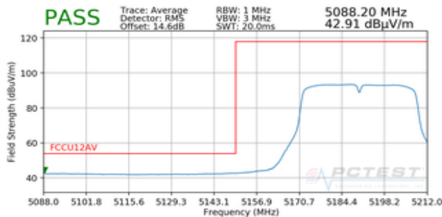
Plot 7-83. Radiated Lower Band Edge Plot (Average – UNII Band 1)
