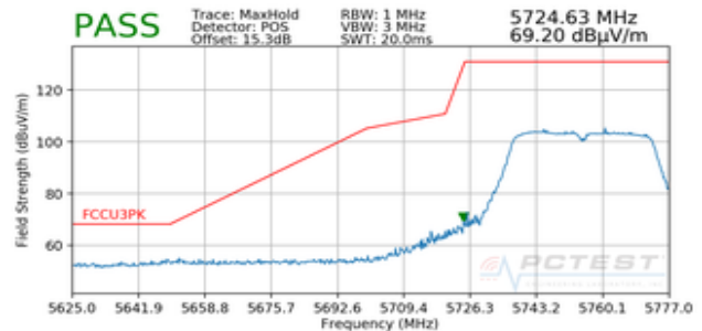
Plot 7-90. Radiated Lower Band Edge Plot (Peak – UNII Band 3)
