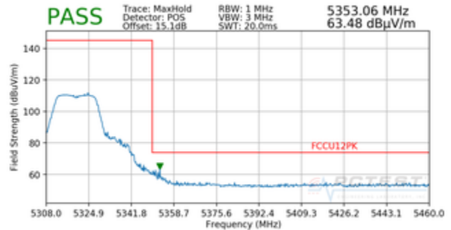
Plot 7-77. Radiated Upper Band Edge Plot (Peak – UNII Band 2A)
