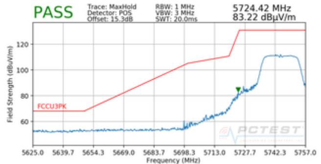
Plot 7-81. Radiated Lower Band Edge Plot (Peak – UNII Band 3)
