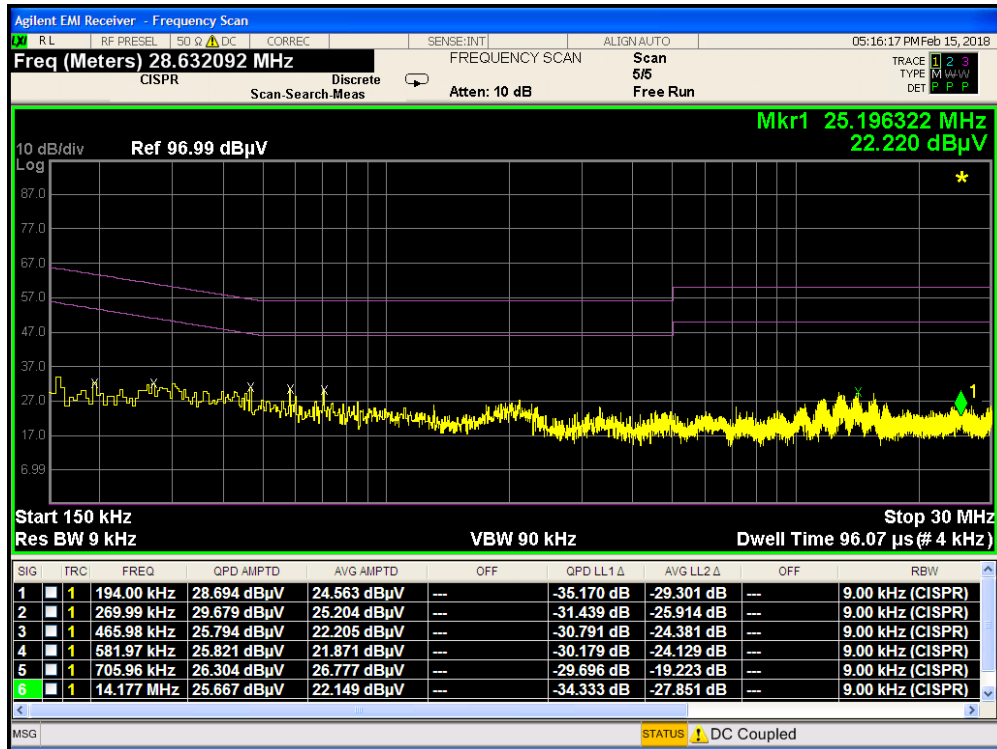
Plot 8-3. Line Conducted Plot with 802.11a UNII Band 2A (L1)
