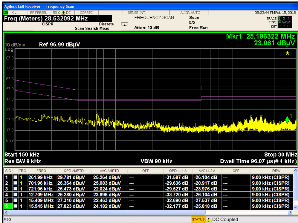
Plot 8-4. Line Conducted Plot with 802.11a UNII Band 2A (N)
