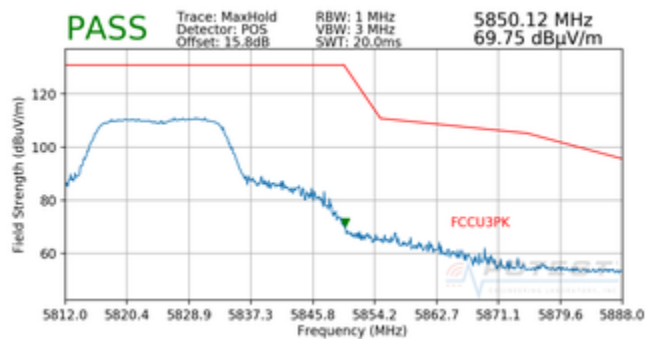
Plot 7-82. Radiated Upper Band Edge Plot (Peak – UNII Band 3)
