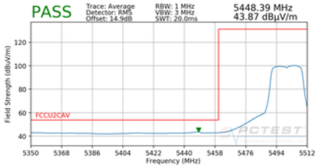
Plot 7-78. Radiated Lower Band Edge Plot (Average – UNII Band 2C)
