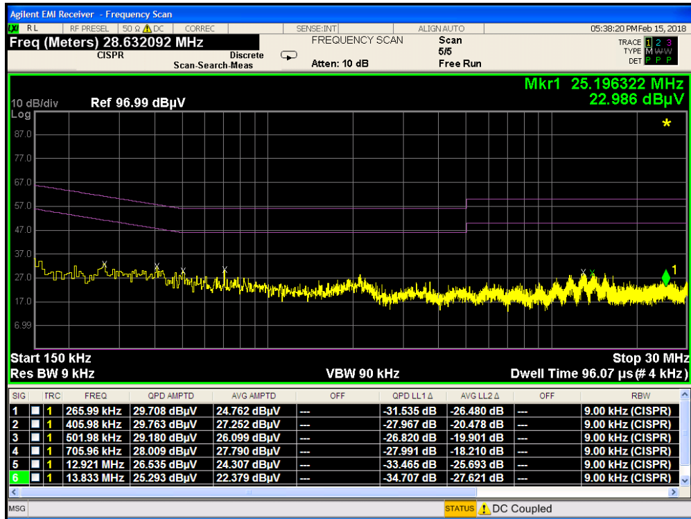
Plot 8-7. Line Conducted Plot with 802.11a UNII Band 3 (L1)
