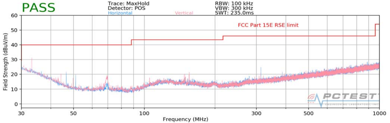
Plot 7-92. Radiated Spurious Plot below 1GHz (802.11a – U3 Ch. 157)
