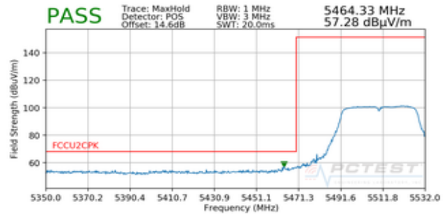
Plot 7-88. Radiated Lower Band Edge Plot (Peak – UNII Band 2C)
