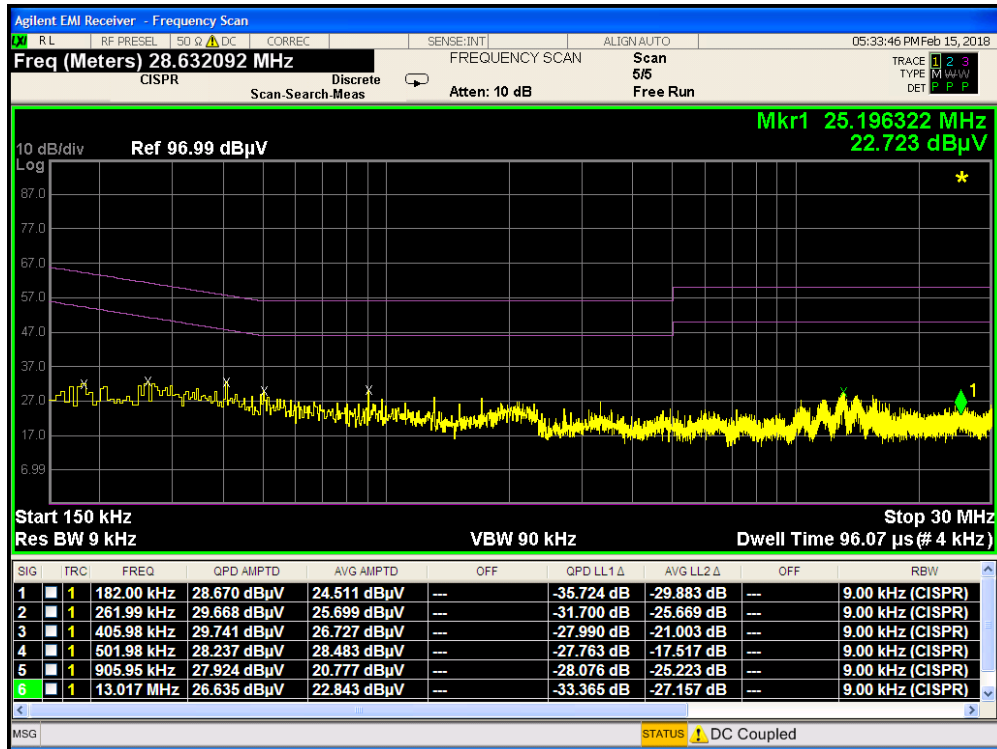
Plot 8-5. Line Conducted Plot with 802.11a UNII Band 2C (L1)
