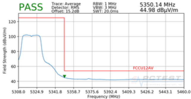
Plot 7-76. Radiated Upper Band Edge Plot (Average – UNII Band 2A)
