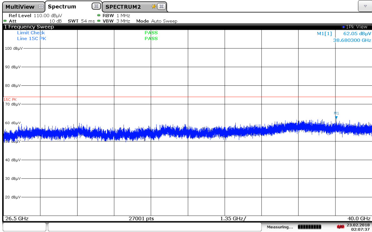
Plot 7-73. Radiated Spurious Plot 26.5GHz - 40GHz (802.11a) (V)
