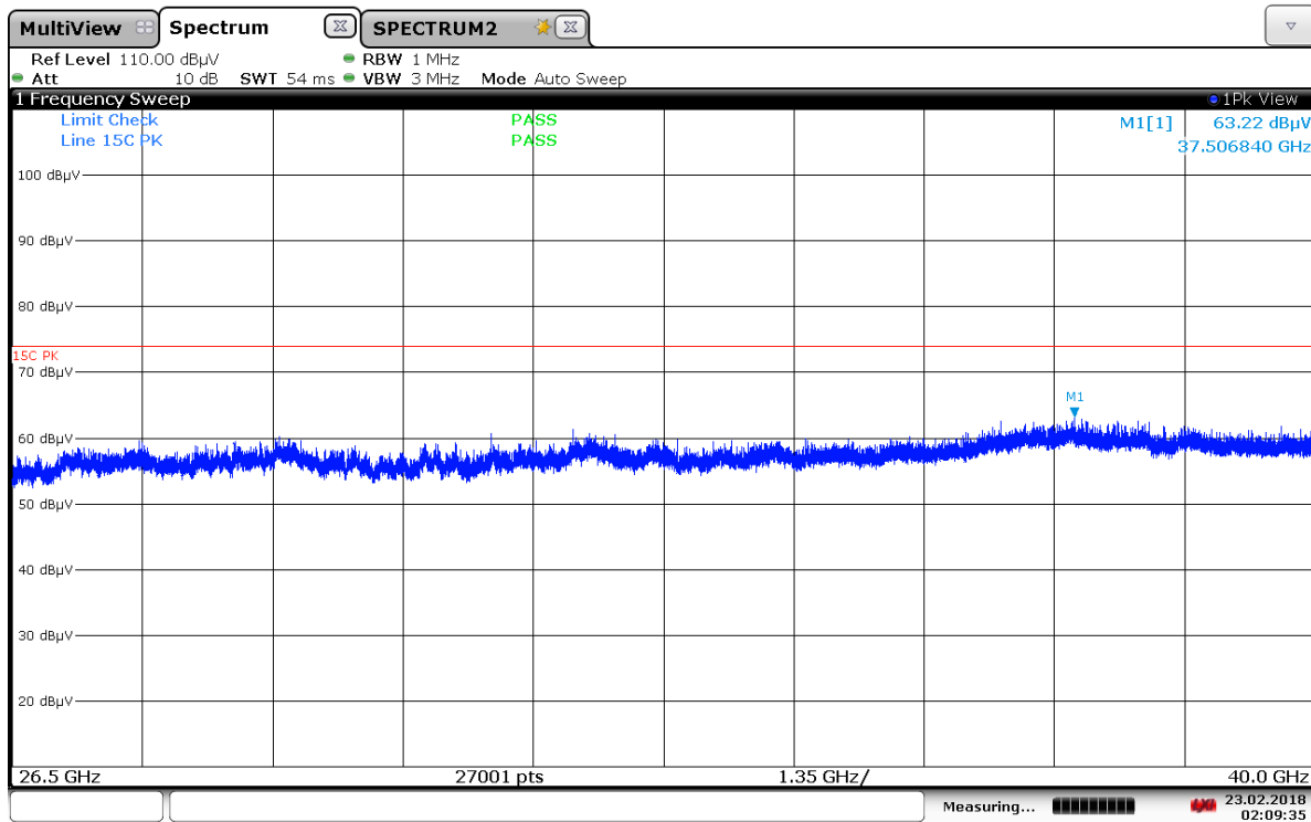
Plot 7-72. Radiated Spurious Plot 26.5GHz - 40GHz (802.11a) (H)
