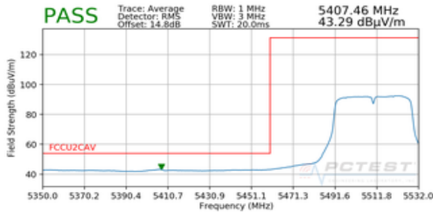
Plot 7-87. Radiated Lower Band Edge Plot (Average – UNII Band 2C)
