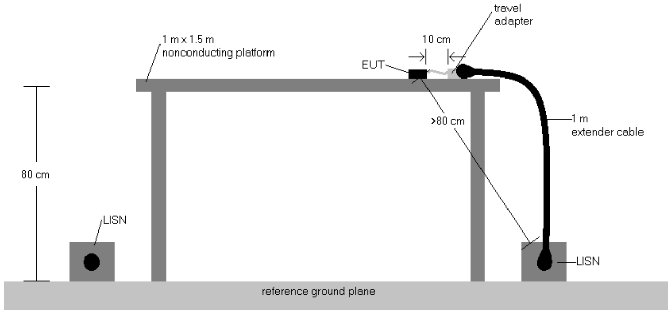
Figure 8-1. Test Instrument & Measurement Setup
