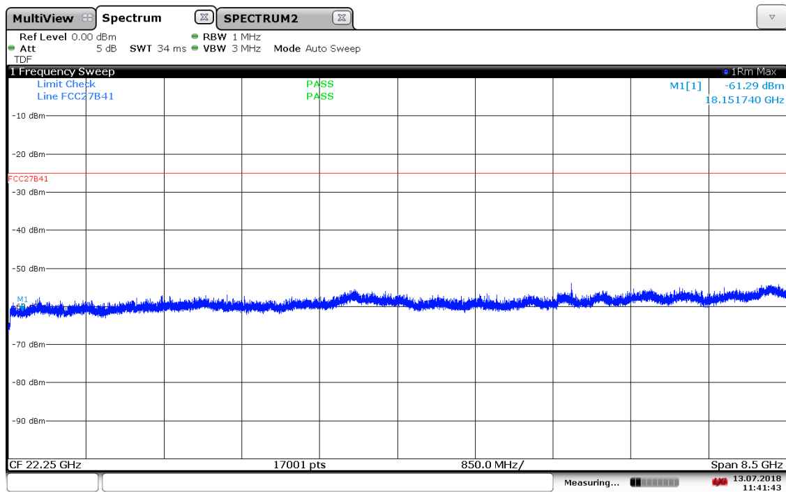
Plot 7-8. Radiated Spurious Plot 18GHz – 26.5GHz (Band 41), V Pol
