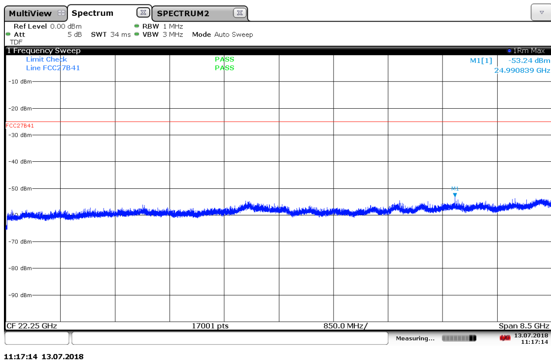
Plot 7-10. Radiated Spurious Plot 18GHz - 26.5GHz (Band 41), H Pol
