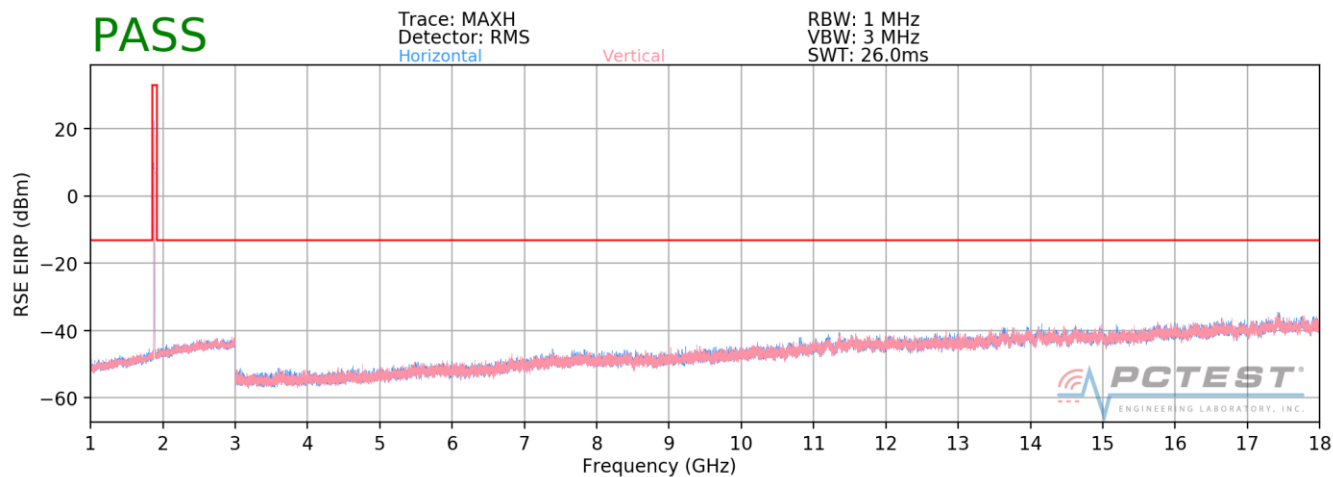
Plot 7-6. Radiated Spurious Plot above 1GHz (PCS CDMA)
