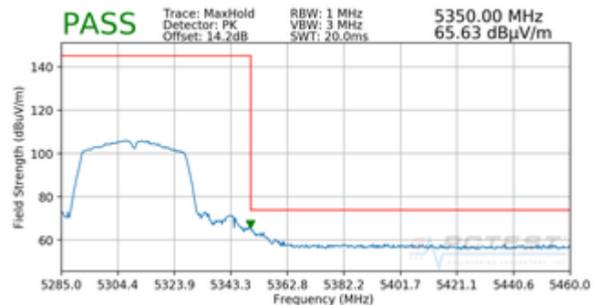
Plot 7-17. Radiated Upper Band Edge Plot (Peak – UNII Band 2A)
