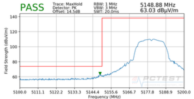
Plot 7-8. Radiated Lower Band Edge Plot (Peak – UNII Band 1)
