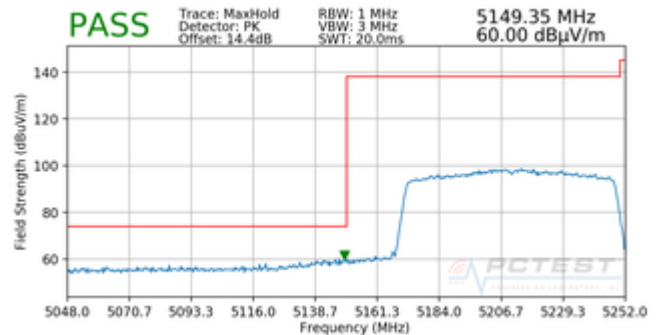
Plot 7-22. Radiated Lower Band Edge Plot (Peak – UNII Band 1)
