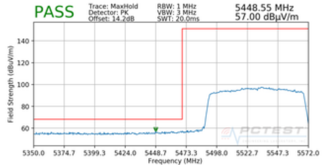
Plot 7-26. Radiated Lower Band Edge Plot (Peak – UNII Band 2C)
