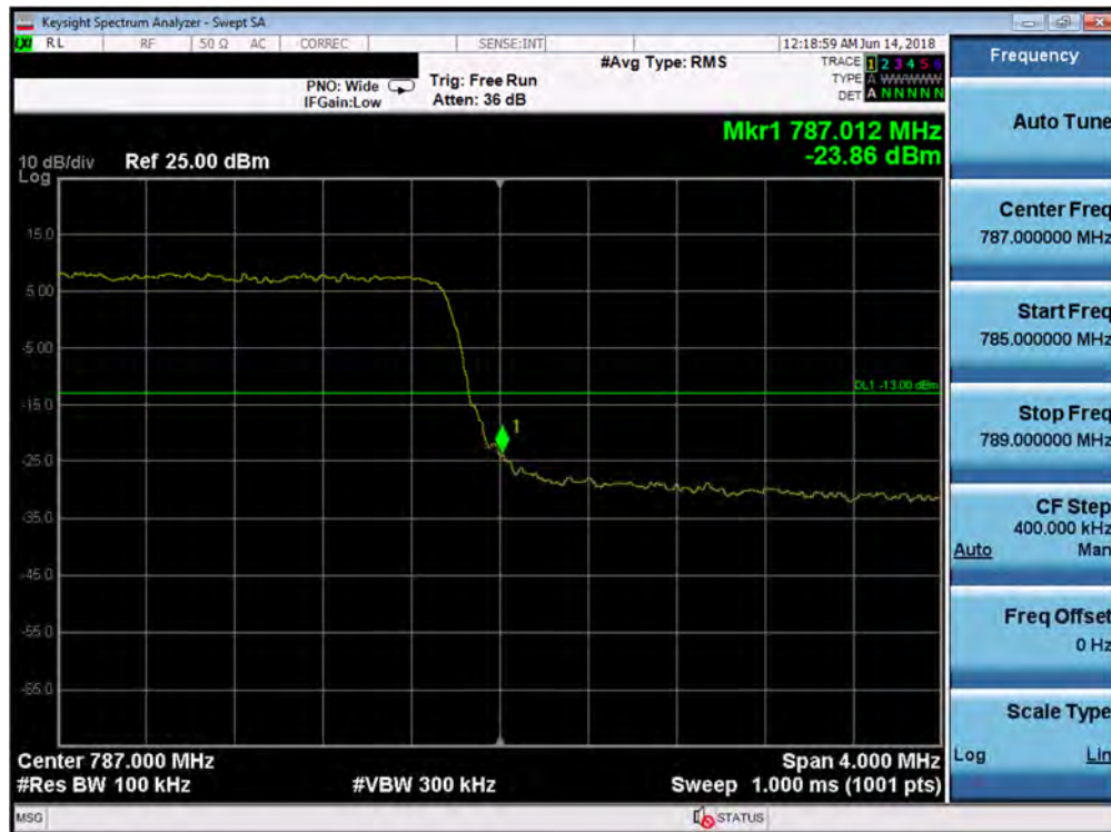
Plot 7-136. Upper Band Edge Plot (Band 13 - 5.0MHz QPSK - Full RB Configuration)
