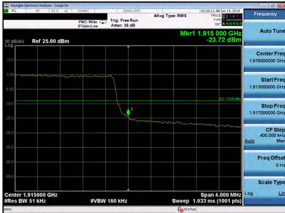
Plot 7-193. Upper Band Edge Plot (Band 25 - 5.0MHz QPSK - Full RB Configuration)
