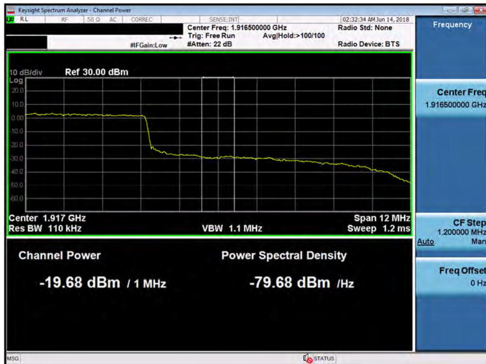
Plot 7-206. Upper Extended Band Edge Plot (Band 25 - 15.0MHz QPSK - Full RB Configuration)
