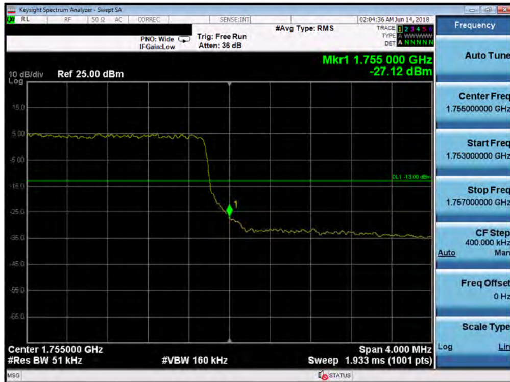
Plot 7-163. Upper Band Edge Plot (Band 4 - 5.0MHz QPSK - Full RB Configuration)
