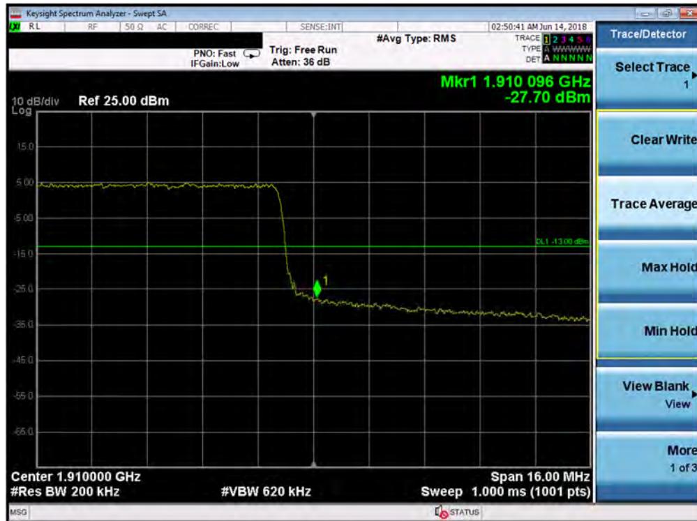
Plot 7-209. Upper Band Edge Plot (Band 2 - 20.0MHz QPSK - Full RB Configuration)
