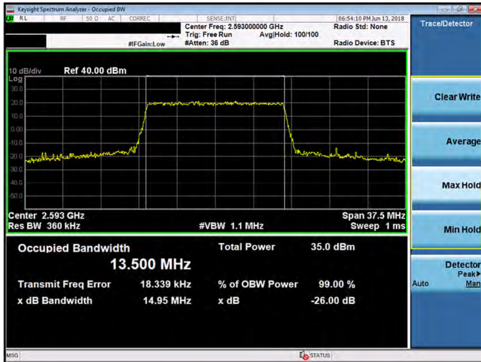
Plot 7-59. Occupied Bandwidth Plot (Band 41 PC2 - 15.0MHz QPSK - Full RB Configuration)
