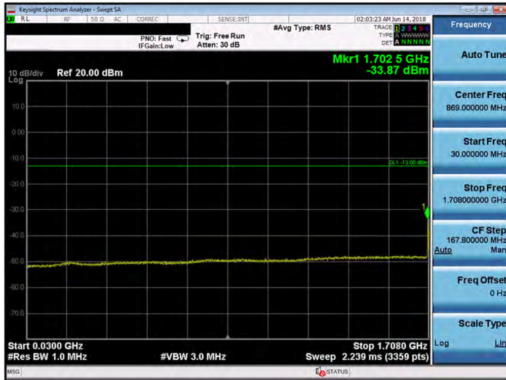
Plot 7-90. Conducted Spurious Plot (Band 4 - 5.0MHz QPSK - RB Size 1, RB Offset 0 - Low Channel)
