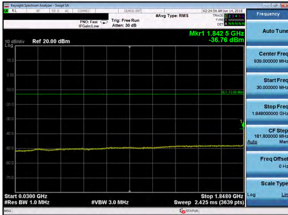
Plot 7-99. Conducted Spurious Plot (Band 25/2 - 5.0MHz QPSK - RB Size 1, RB Offset 0 - Low Channel)
