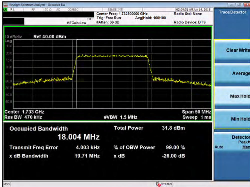
Plot 7-34. Occupied Bandwidth Plot (Band 4 - 20.0MHz 16-QAM - Full RB Configuration)
