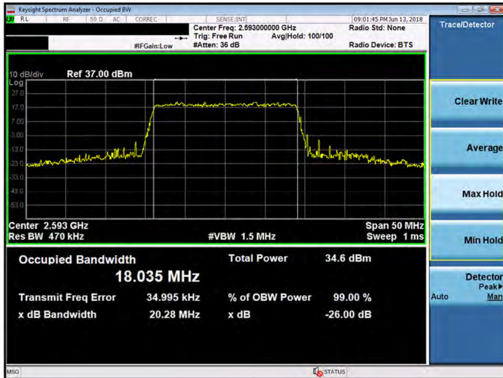
Plot 7-62. Occupied Bandwidth Plot (Band 41 PC2 - 20.0MHz 16-QAM - Full RB Configuration)
