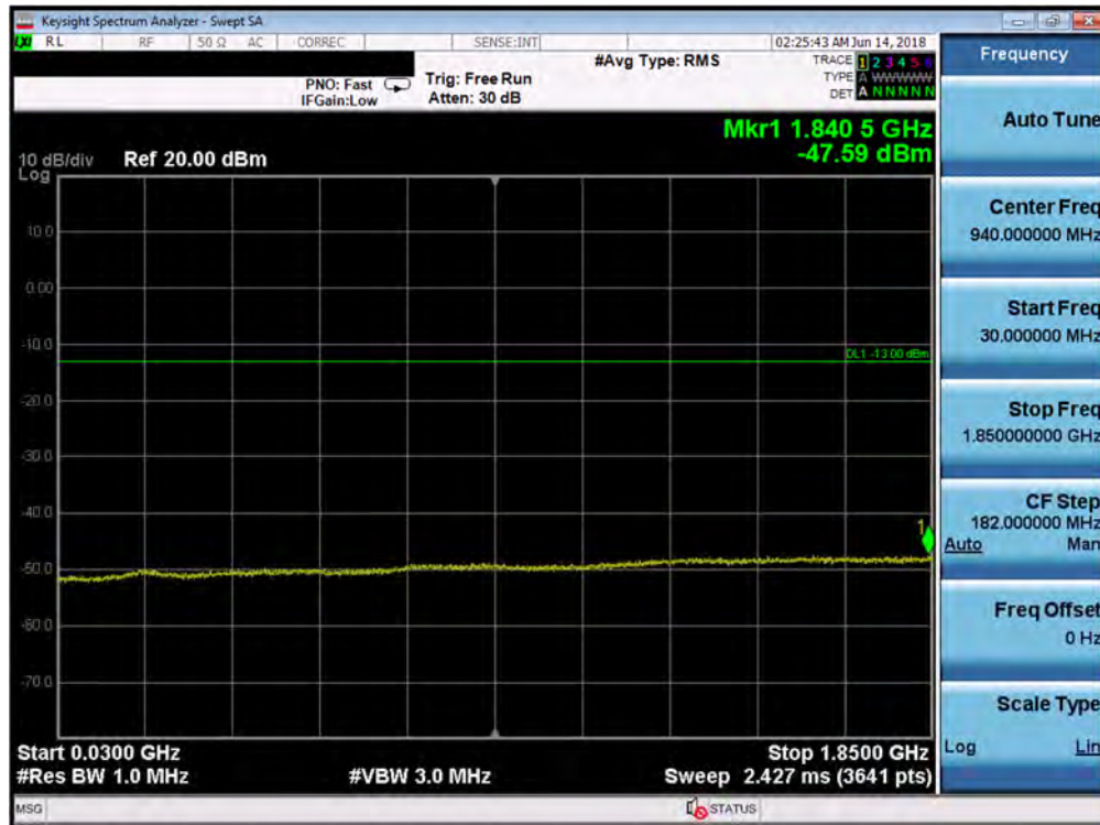
Plot 7-105. Conducted Spurious Plot (Band 25/2 - 5.0MHz QPSK - RB Size 1, RB Offset 0 - High Channel)
