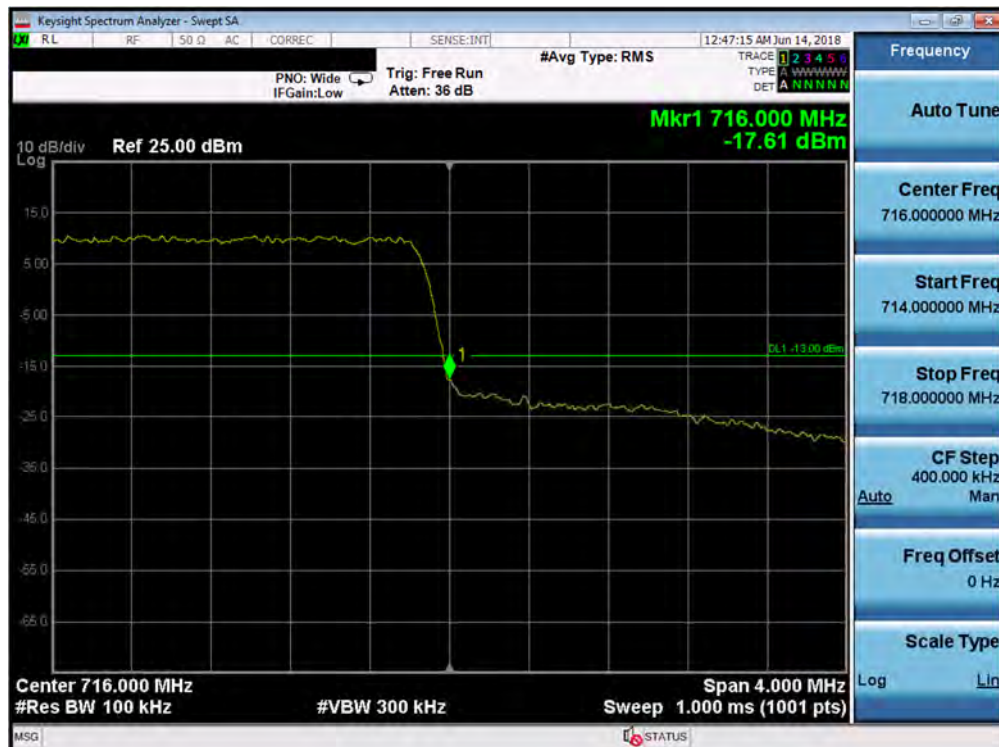
Plot 7-129. Upper Band Edge Plot (Band 12 - 3.0MHz QPSK - Full RB Configuration)
