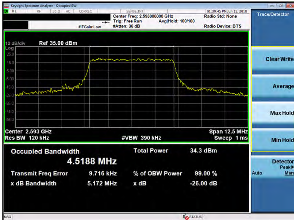
Plot 7-56. Occupied Bandwidth Plot (Band 41 PC2 - 5.0MHz 16-QAM - Full RB Configuration)
