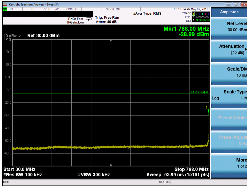
Plot 7-5. Conducted Spurious Plot (LTE B14 – 10.0MHz QPSK – RB Size 1, RB Offset 0 – Mid Channel)
