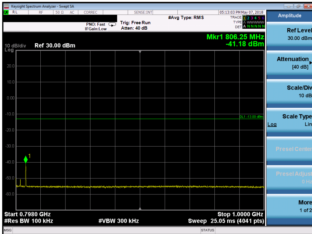
Plot 7-6. Conducted Spurious Plot (LTE B14 – 5100MHz QPSK – RB Size 1, RB Offset 0 – Mid Channel)
