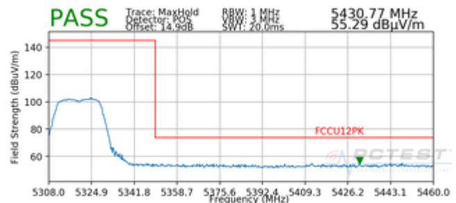
Plot 7-86. Radiated Upper Band Edge Plot SISO ANT1 (Peak – UNII Band 2A)
