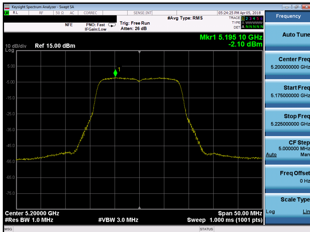
Plot 7-40. Power Spectral Density Plot SISO ANT1 (802.11a (UNII Band 1) – Ch. 40)
