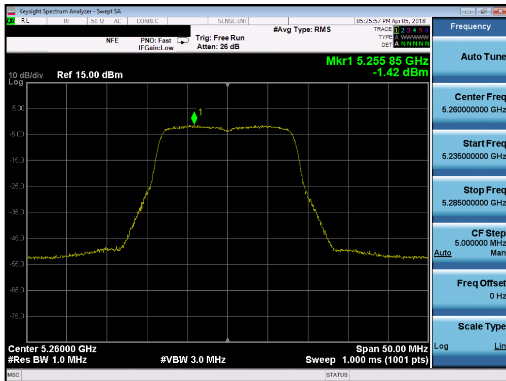
Plot 7-48. Power Spectral Density Plot SISO ANT1 (802.11a (UNII Band 2A) – Ch. 52)
