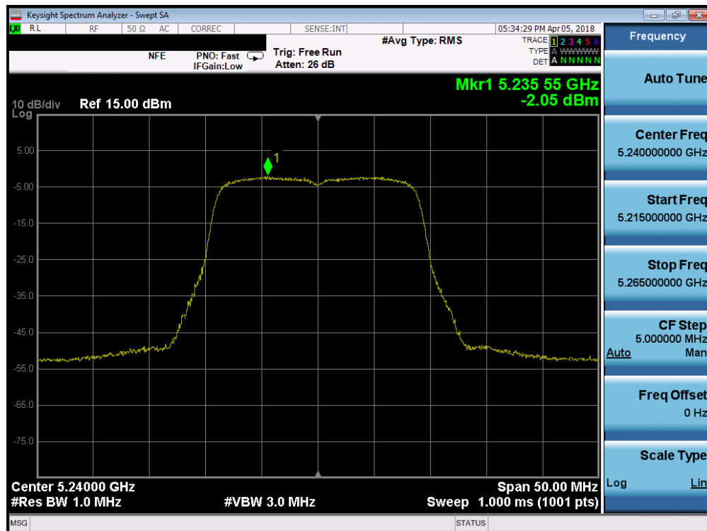
Plot 7-44. Power Spectral Density Plot SISO ANT1 (20MHz BW 802.11n (UNII Band 1) – Ch. 48)
