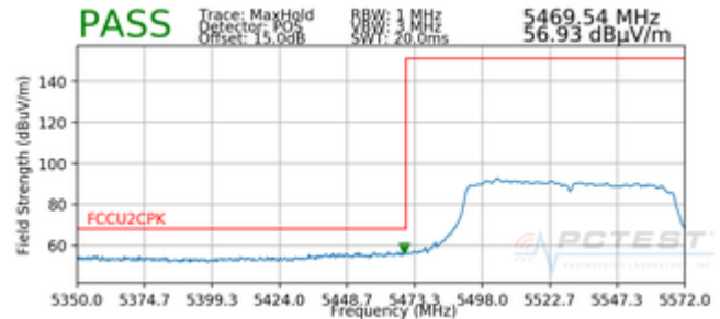
Plot 7-106. Radiated Lower Band Edge Plot SISO ANT1 (Peak – UNII Band 2C)
