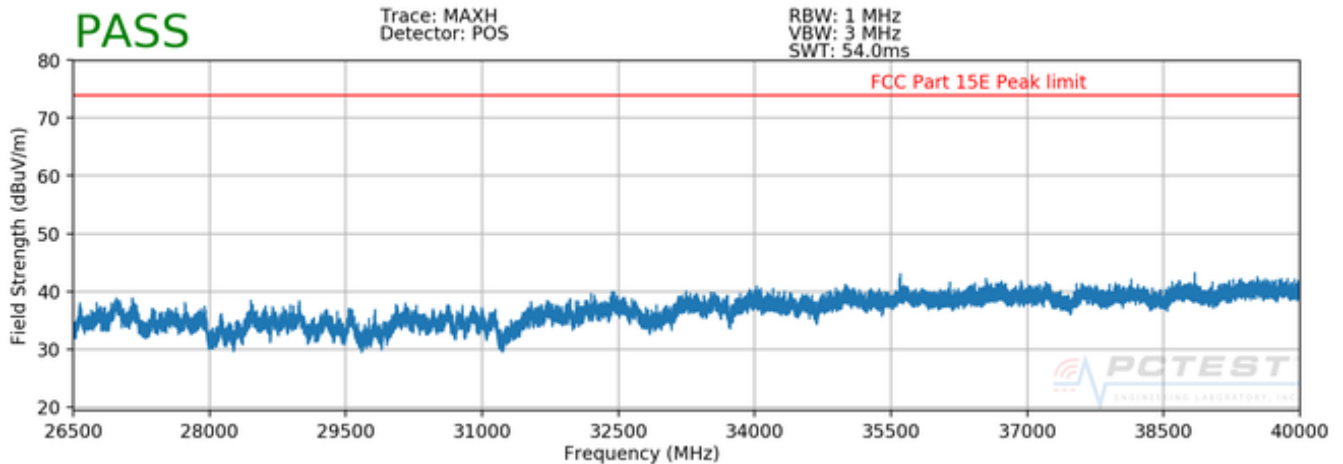
Plot 7-82. Radiated Spurious Plot 26.5GHz - 40GHz SISO ANT1 (802.11a)
