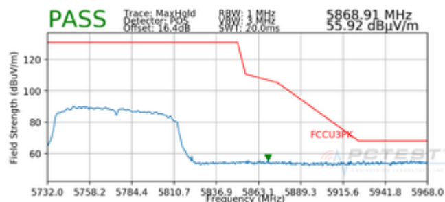
Plot 7-108. Radiated Upper Band Edge Plot SISO ANT1 (Peak – UNII Band 3)
