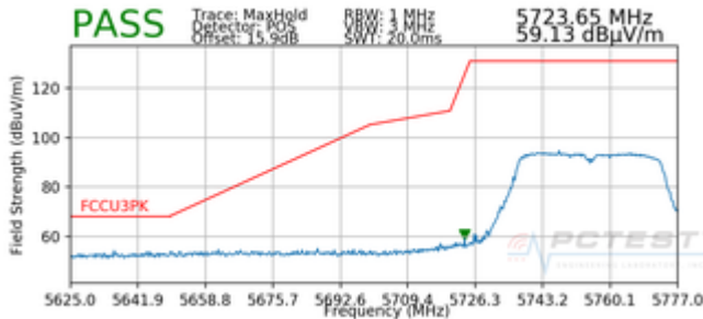
Plot 7-99. Radiated Lower Band Edge Plot SISO ANT1 (Peak – UNII Band 3)
