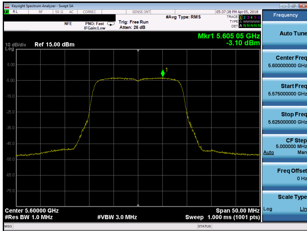
Plot 7-61. Power Spectral Density Plot SISO ANT1 (20MHz BW 802.11n (UNII Band 2C) – Ch. 120)
