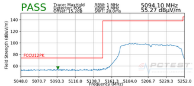
Plot 7-102. Radiated Lower Band Edge Plot SISO ANT1 (Peak – UNII Band 1)
