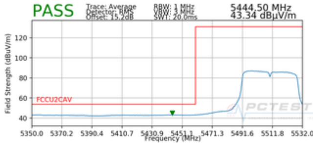
Plot 7-96. Radiated Lower Band Edge Plot SISO ANT1 (Average – UNII Band 2C)
