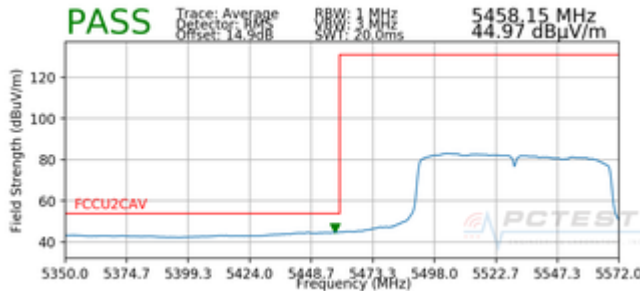
Plot 7-105. Radiated Lower Band Edge Plot SISO ANT1 (Average – UNII Band 2C)
