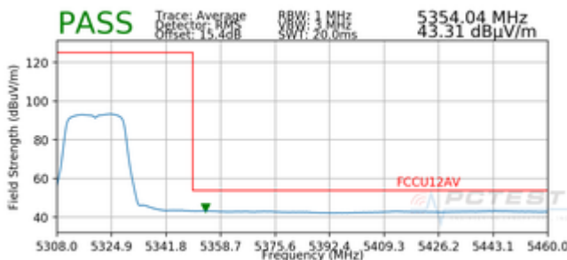
Plot 7-85. Radiated Upper Band Edge Plot SISO ANT1 (Average – UNII Band 2A)
