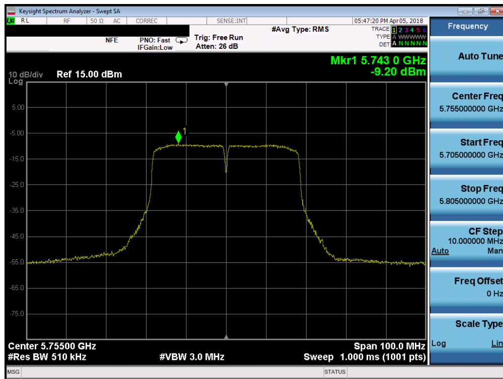
Plot 7-74. Power Spectral Density Plot SISO ANT1 (40MHz BW 802.11n (UNII Band 3) – Ch. 151)
