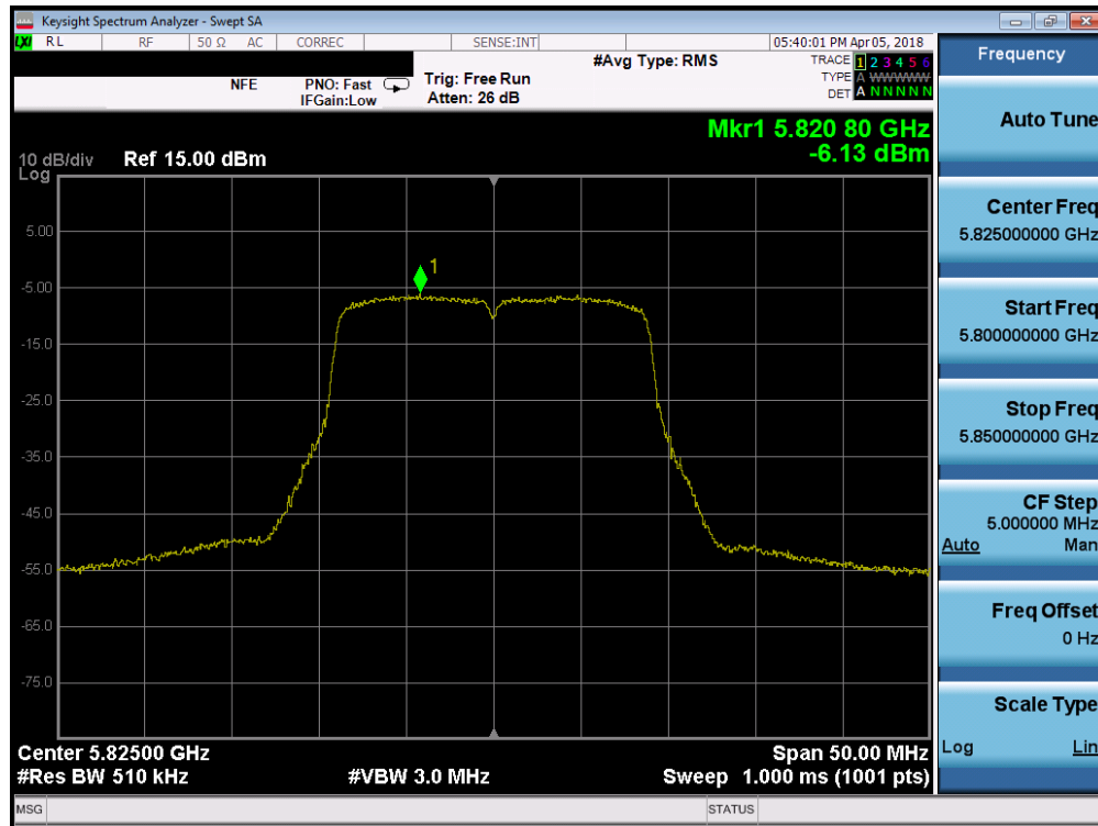
Plot 7-73. Power Spectral Density Plot SISO ANT1 (20MHz BW 802.11n (UNII Band 3) – Ch. 165)
