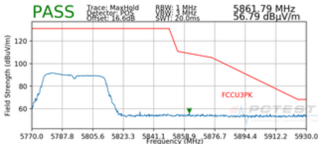
Plot 7-100. Radiated Upper Band Edge Plot SISO ANT1 (Peak – UNII Band 3)
