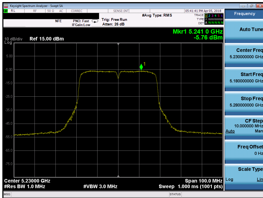
Plot 7-46. Power Spectral Density Plot SISO ANT1 (40MHz BW 802.11n (UNII Band 1) – Ch. 46)
