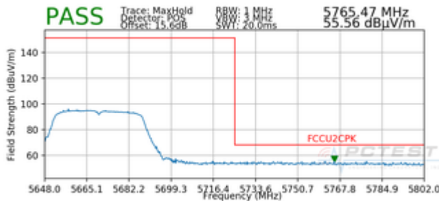
Plot 7-98. Radiated Upper Band Edge Plot SISO ANT1 (Peak – UNII Band 2C)
