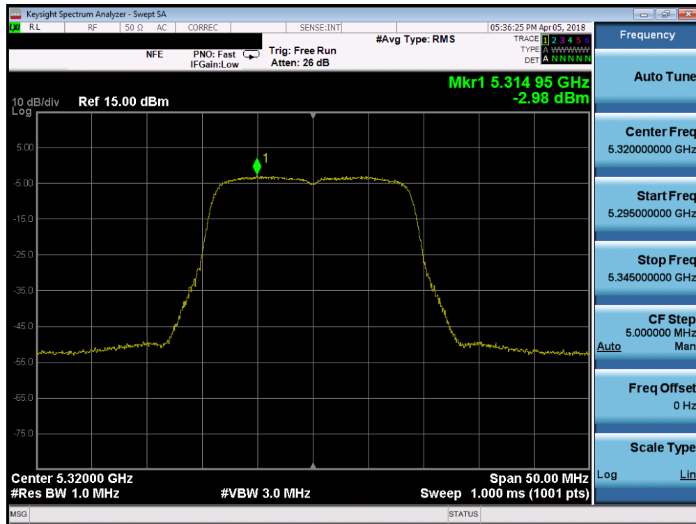
Plot 7-53. Power Spectral Density Plot SISO ANT1 (20MHz BW 802.11n (UNII Band 2A) – Ch. 64)
