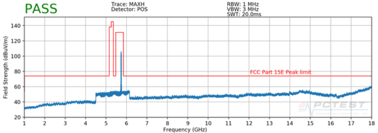
Plot 7-80. Radiated Spurious Plot above 1GHz SISO ANT1 (802.11a – U3 Ch. 157)
