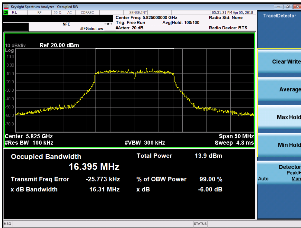
Plot 7-32. 6dB Bandwidth Plot SISO ANT1 (802.11a (UNII Band 3) – Ch. 165)
