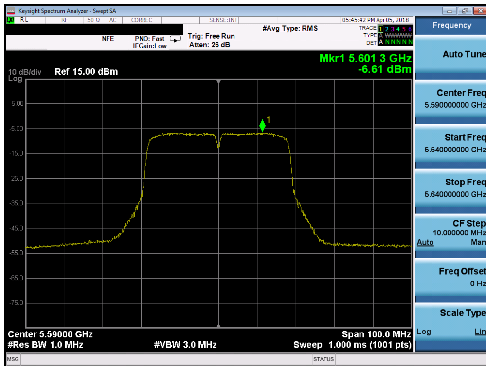
Plot 7-64. Power Spectral Density Plot SISO ANT1 (40MHz BW 802.11n (UNII Band 2C) – Ch. 118)
