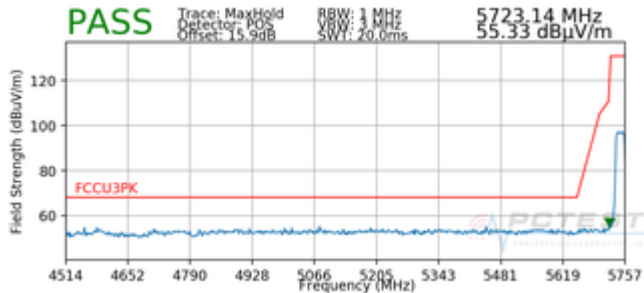
Plot 7-90. Radiated Lower Band Edge Plot SISO ANT1 (Peak – UNII Band 3)
