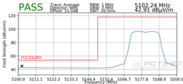
Plot 7-83. Radiated Lower Band Edge Plot SISO ANT1 (Average – UNII Band 1)
