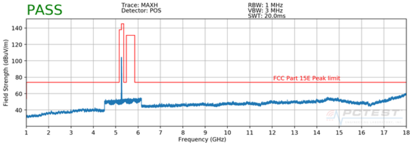
Plot 7-78. Radiated Spurious Plot above 1GHz SISO ANT1 (802.11a – U2A Ch. 56)
