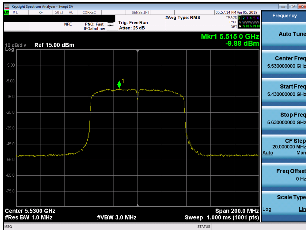
Plot 7-66. Power Spectral Density Plot SISO ANT1 (80MHz BW 802.11ac (UNII Band 2C) – Ch. 106)
