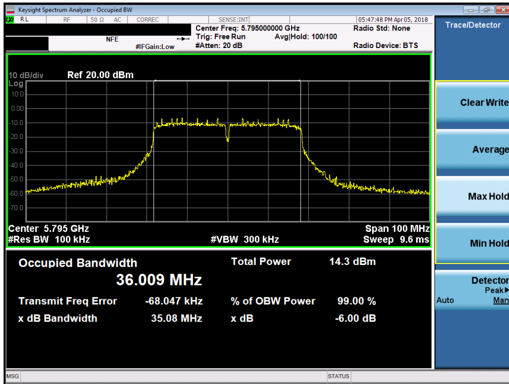
Plot 7-37. 6dB Bandwidth Plot SISO ANT1 (40MHz BW 802.11n (UNII Band 3) – Ch. 159)
