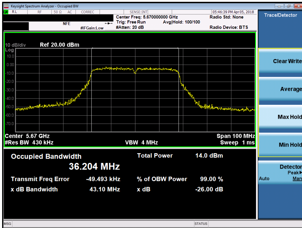
Plot 7-27. 26dB Bandwidth Plot SISO ANT1 (40MHz BW 802.11n (UNII Band 2C) – Ch. 134)
