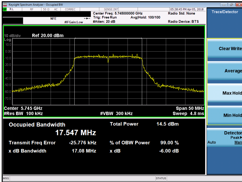
Plot 7-33. 6dB Bandwidth Plot SISO ANT1 (20MHz BW 802.11n (UNII Band 3) – Ch. 149)
