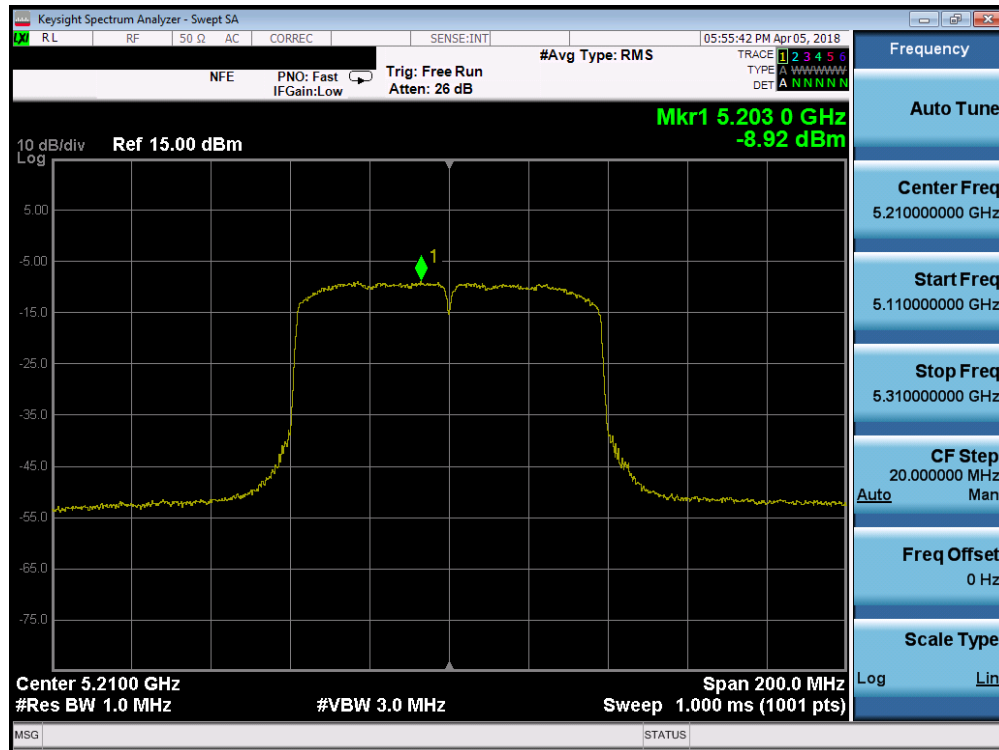
Plot 7-47. Power Spectral Density Plot SISO ANT1 (80MHz BW 802.11ac (UNII Band 1) – Ch. 42)
