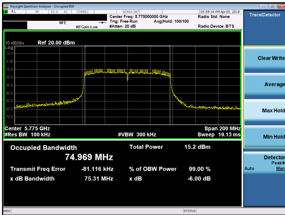
Plot 7-38. 6dB Bandwidth Plot SISO ANT1 (80MHz BW 802.11ac (UNII Band 3) – Ch. 155)
