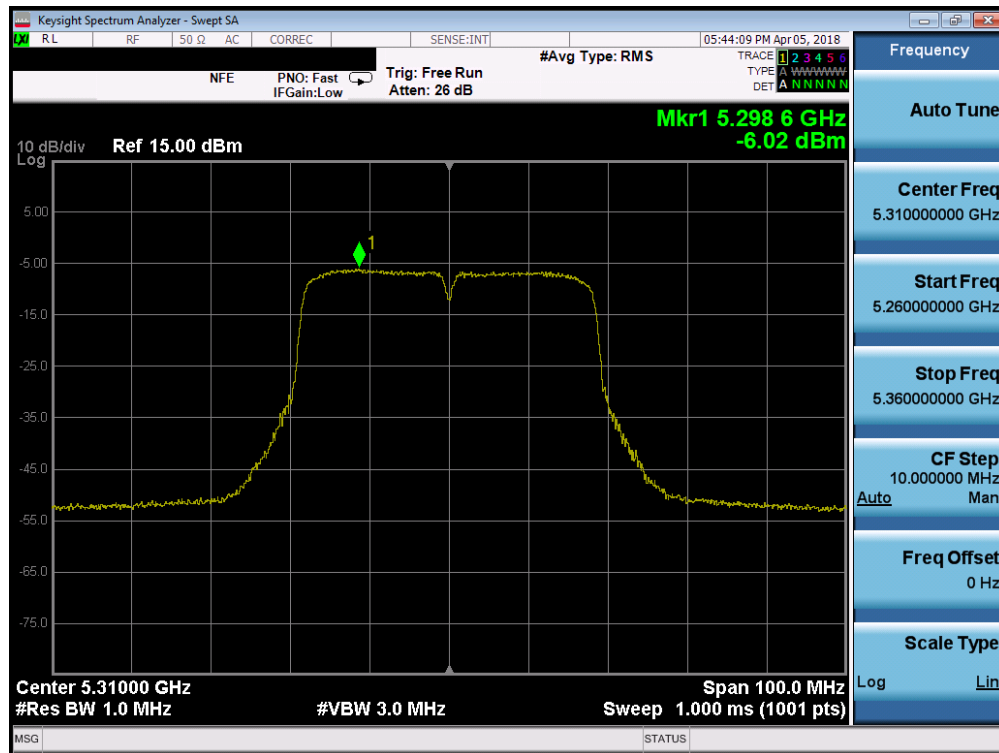
Plot 7-55. Power Spectral Density Plot SISO ANT1 (40MHz BW 802.11n (UNII Band 2A) – Ch. 62)
