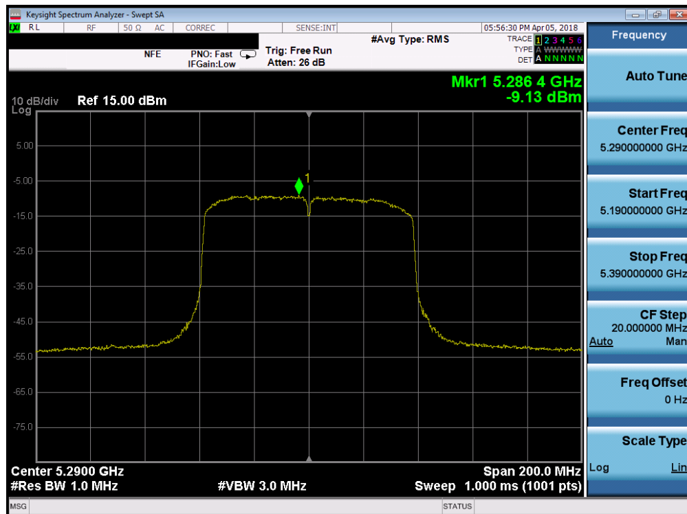
Plot 7-56. Power Spectral Density Plot SISO ANT1 (80MHz BW 802.11ac (UNII Band 2A) – Ch. 58)
