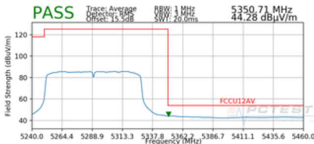
Plot 7-103. Radiated Upper Band Edge Plot SISO ANT1 (Average – UNII Band 2A)
