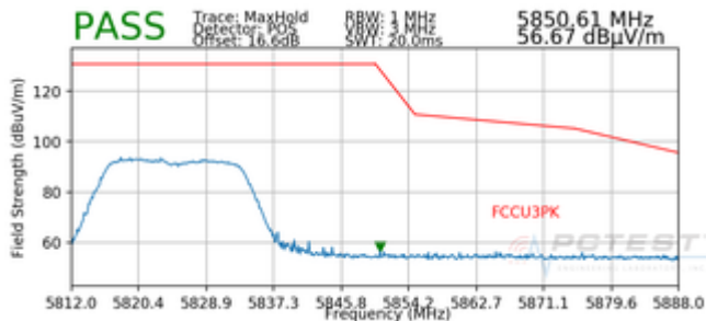
Plot 7-91. Radiated Upper Band Edge Plot SISO ANT1 (Peak – UNII Band 3)
