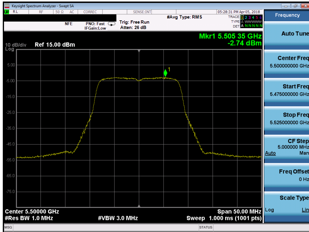
Plot 7-57. Power Spectral Density Plot SISO ANT1 (802.11a (UNII Band 2C) – Ch. 100)
