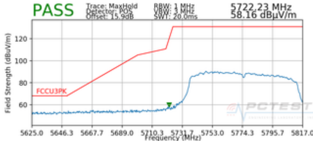
Plot 7-107. Radiated Lower Band Edge Plot SISO ANT1 (Peak – UNII Band 3)
