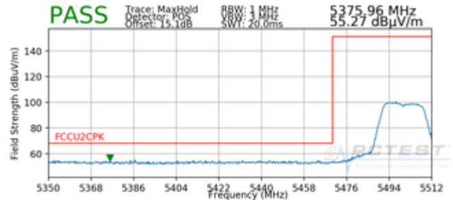
Plot 7-88. Radiated Lower Band Edge Plot SISO ANT1 (Peak – UNII Band 2C)
