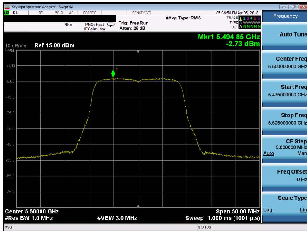
Plot 7-60. Power Spectral Density Plot SISO ANT1 (20MHz BW 802.11n (UNII Band 2C) – Ch. 100)
