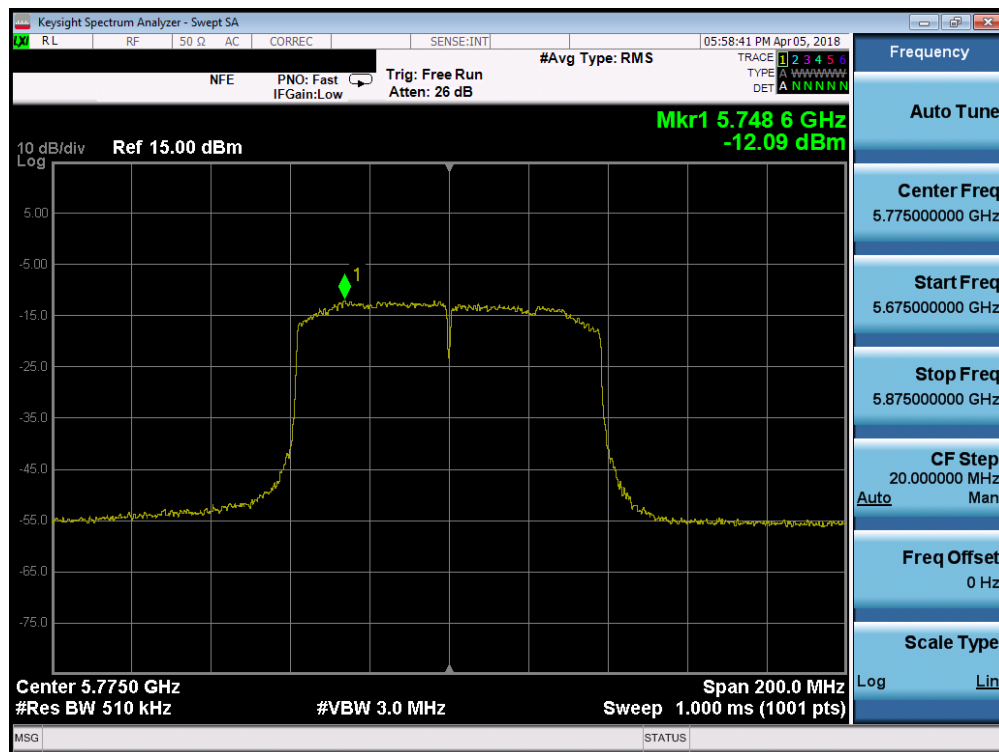
Plot 7-76. Power Spectral Density Plot SISO ANT1 (80MHz BW 802.11ac (UNII Band 3) – Ch. 155)
