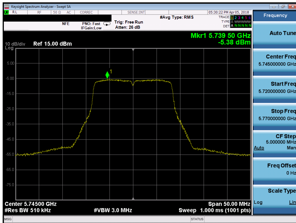
Plot 7-68. Power Spectral Density Plot SISO ANT1 (802.11a (UNII Band 3) – Ch. 149)
