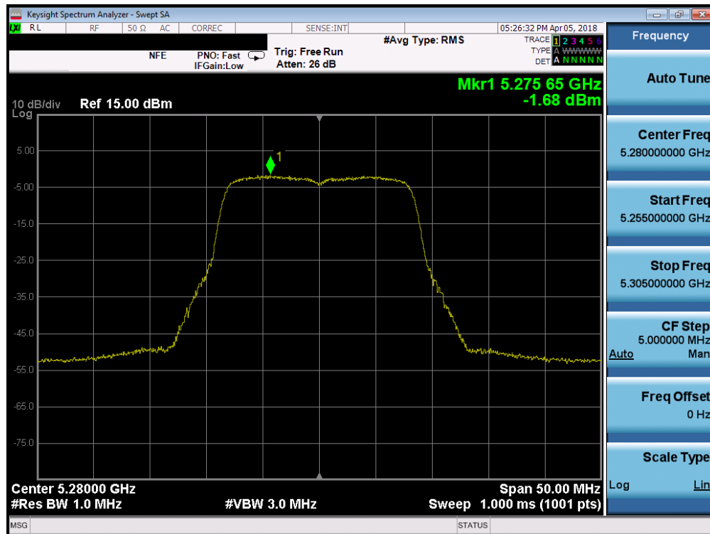
Plot 7-49. Power Spectral Density Plot SISO ANT1 (802.11a (UNII Band 2A) – Ch. 56)
