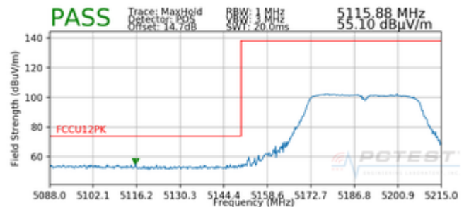
Plot 7-93. Radiated Lower Band Edge Plot SISO ANT1 (Peak – UNII Band 1)
