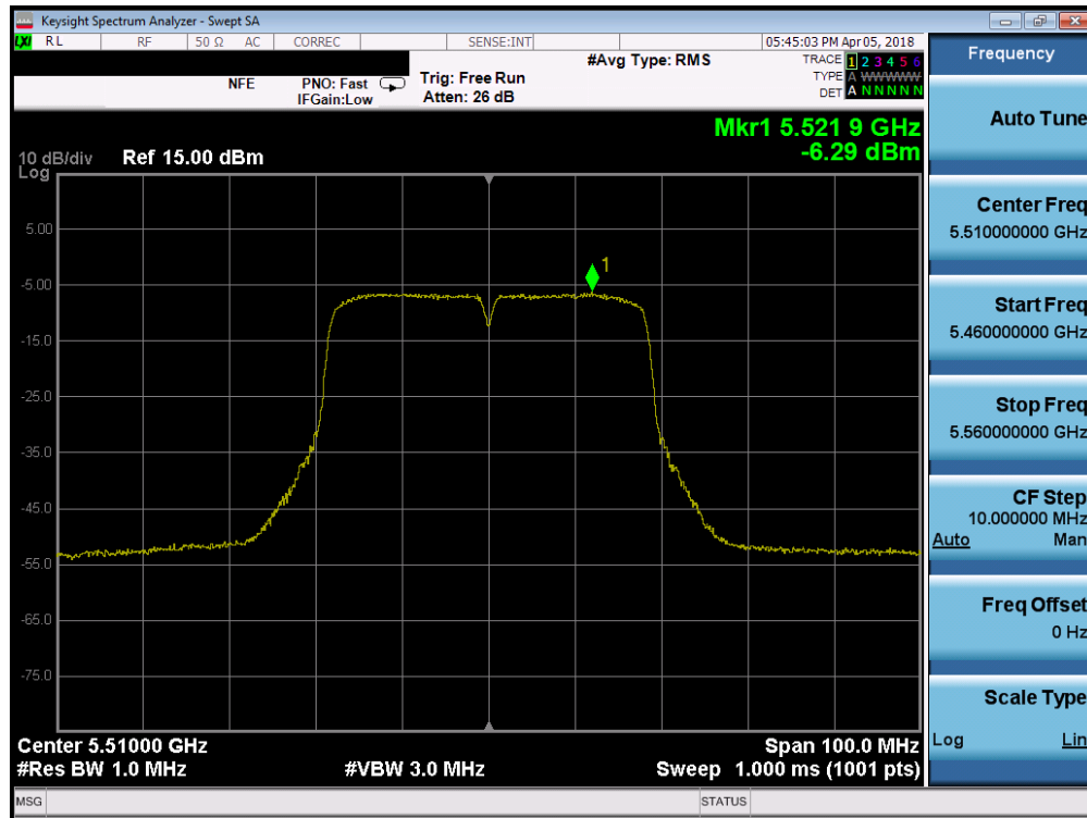
Plot 7-63. Power Spectral Density Plot SISO ANT1 (40MHz BW 802.11n (UNII Band 2C) – Ch. 102)
