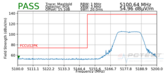
Plot 7-84. Radiated Lower Band Edge Plot SISO ANT1 (Peak – UNII Band 1)
