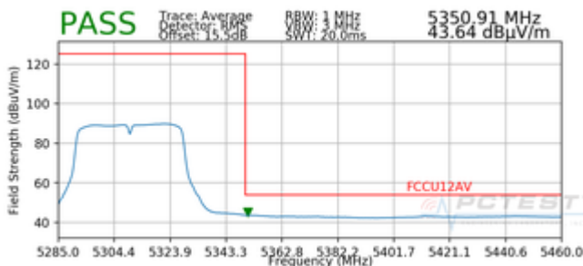
Plot 7-94. Radiated Upper Band Edge Plot SISO ANT1 (Average – UNII Band 2A)
