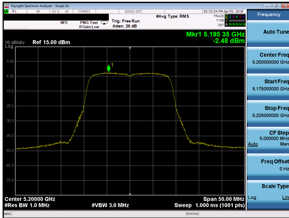
Plot 7-43. Power Spectral Density Plot SISO ANT1 (20MHz BW 802.11n (UNII Band 1) – Ch. 40)
