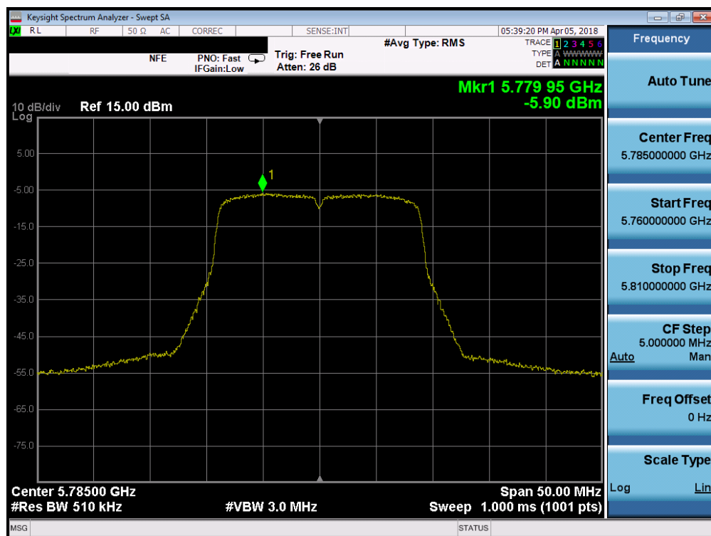
Plot 7-72. Power Spectral Density Plot SISO ANT1 (20MHz BW 802.11n (UNII Band 3) – Ch. 157)
