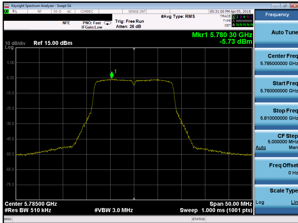
Plot 7-69. Power Spectral Density Plot SISO ANT1 (802.11a (UNII Band 3) – Ch. 157)
