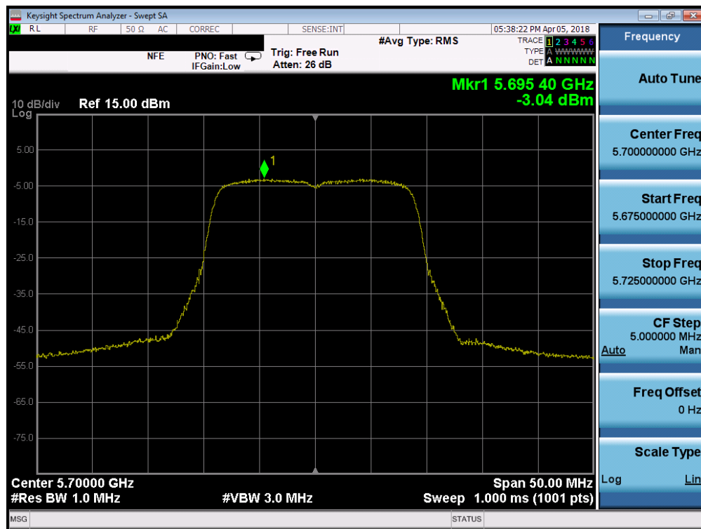
Plot 7-62. Power Spectral Density Plot SISO ANT1 (20MHz BW 802.11n (UNII Band 2C) – Ch. 140)
