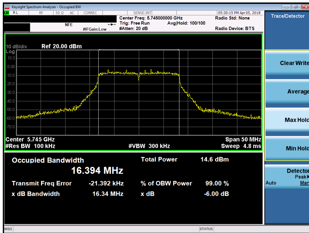
Plot 7-30. 6dB Bandwidth Plot SISO ANT1 (802.11a (UNII Band 3) – Ch. 149)
