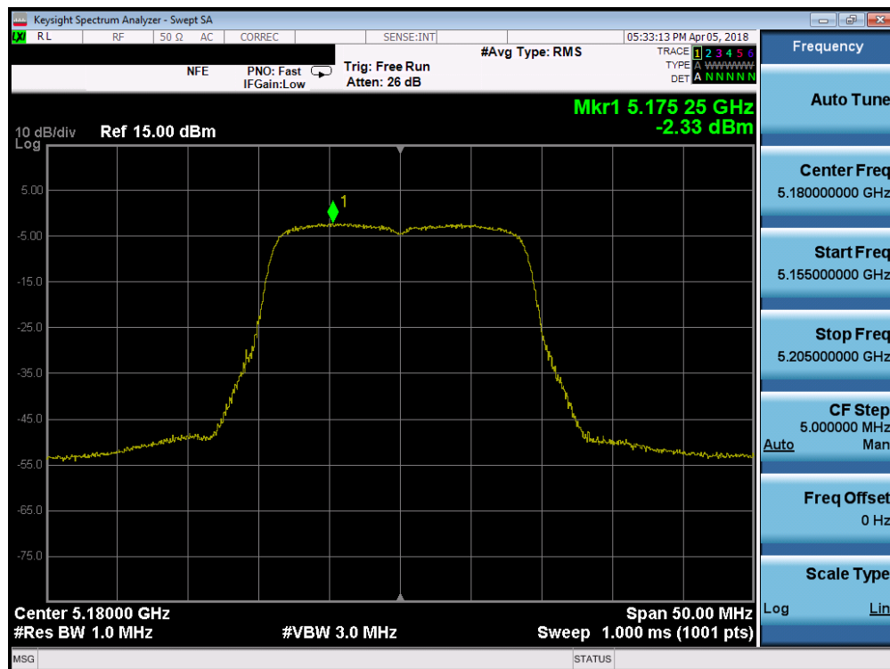
Plot 7-42. Power Spectral Density Plot SISO ANT1 (20MHz BW 802.11n (UNII Band 1) – Ch. 36)
