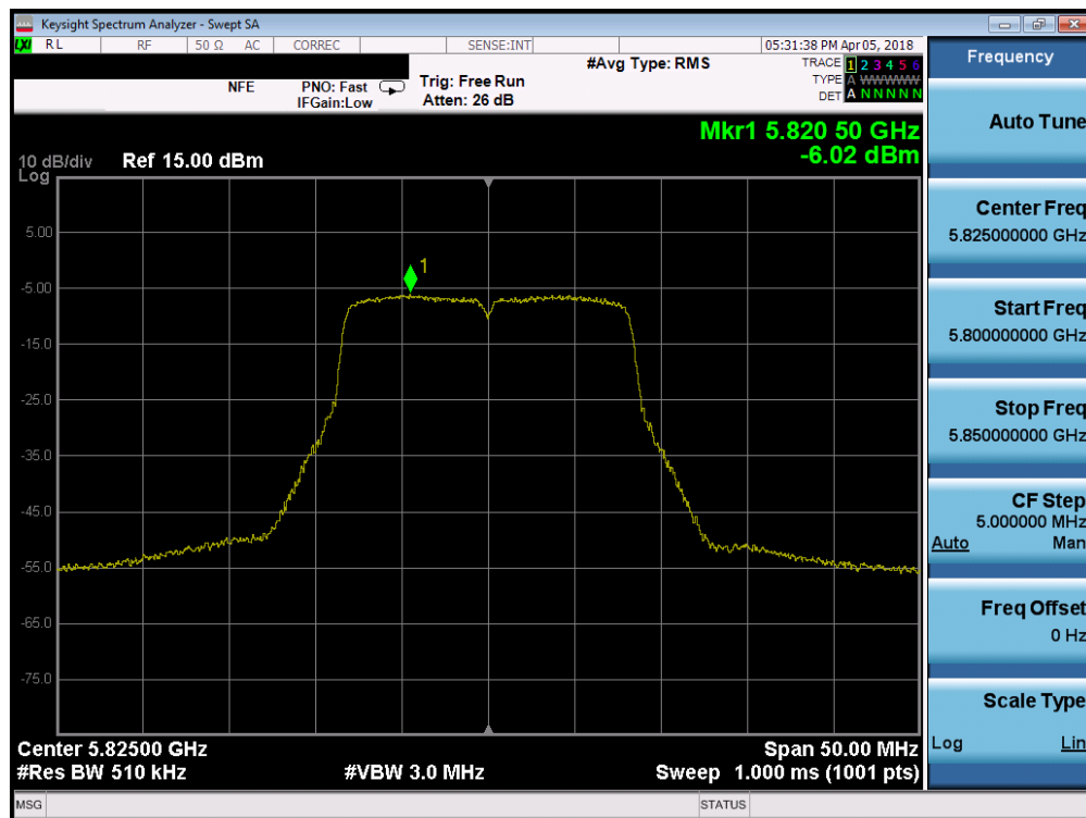
Plot 7-70. Power Spectral Density Plot SISO ANT1 (802.11a (UNII Band 3) – Ch. 165)
