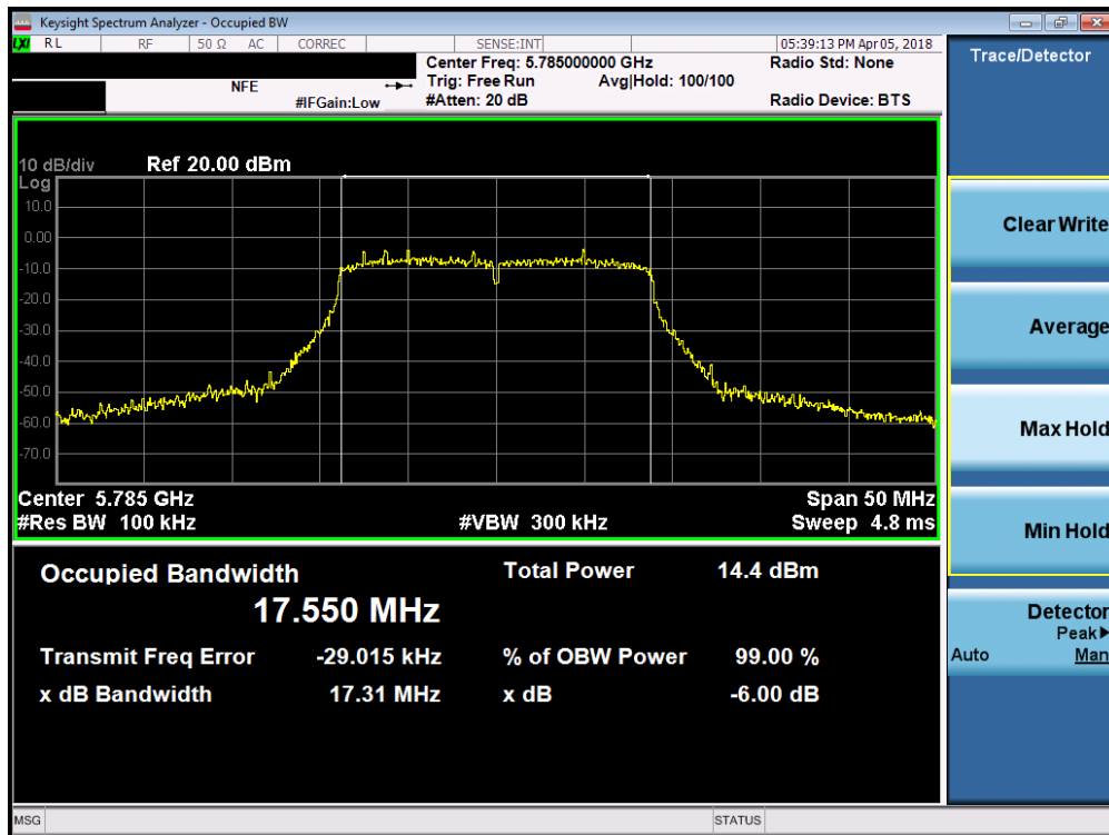
Plot 7-34. 6dB Bandwidth Plot SISO ANT1 (20MHz BW 802.11n (UNII Band 3) – Ch. 157)
