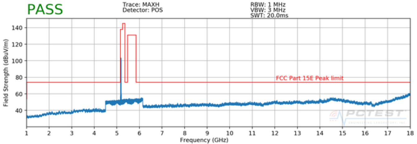
Plot 7-77. Radiated Spurious Plot above 1GHz SISO ANT1 (802.11a – U1 Ch. 40)
