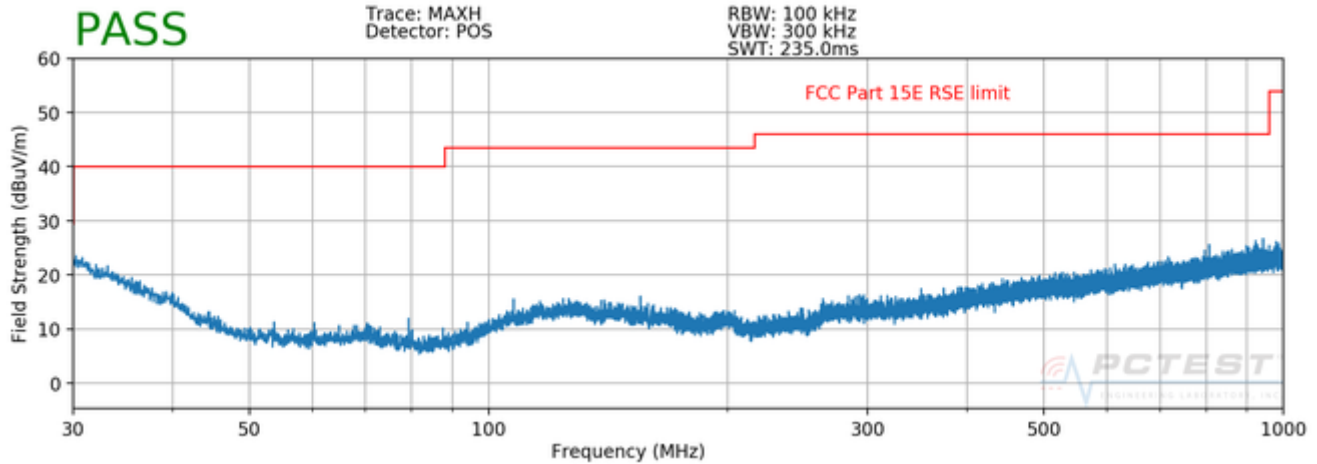
Plot 7-109. Radiated Spurious Plot below 1GHz SISO ANT1 (802.11a – U3 Ch. 157)
