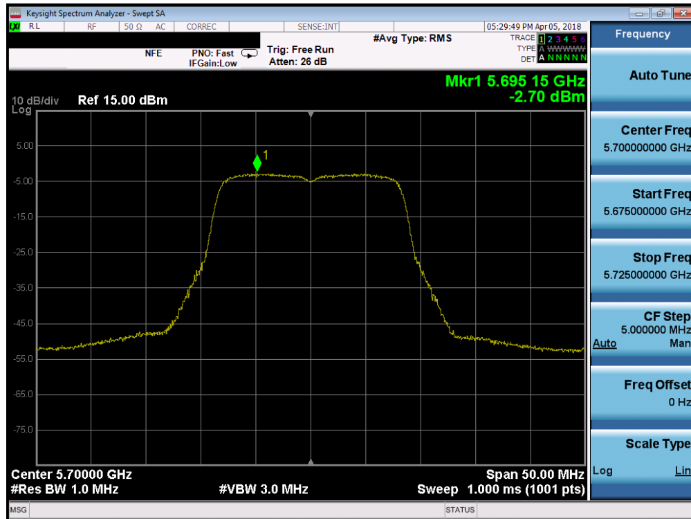
Plot 7-59. Power Spectral Density Plot SISO ANT1 (802.11a (UNII Band 2C) – Ch. 140)
