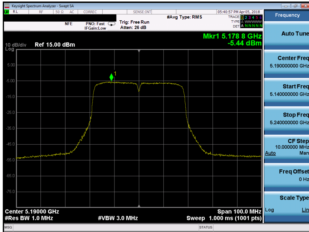
Plot 7-45. Power Spectral Density Plot SISO ANT1 (40MHz BW 802.11n (UNII Band 1) – Ch. 38)
