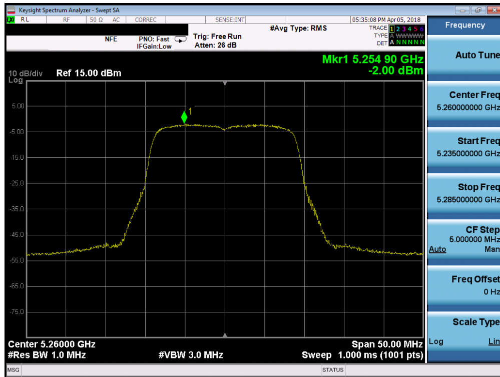
Plot 7-51. Power Spectral Density Plot SISO ANT1 (20MHz BW 802.11n (UNII Band 2A) – Ch. 52)
