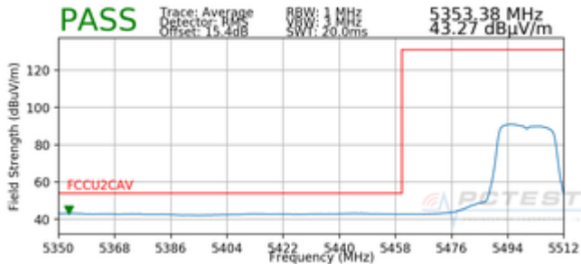
Plot 7-87. Radiated Lower Band Edge Plot SISO ANT1 (Average – UNII Band 2C)
