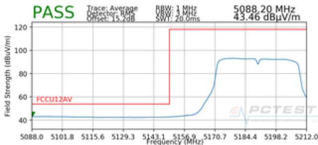
Plot 7-92. Radiated Lower Band Edge Plot SISO ANT1 (Average – UNII Band 1)
