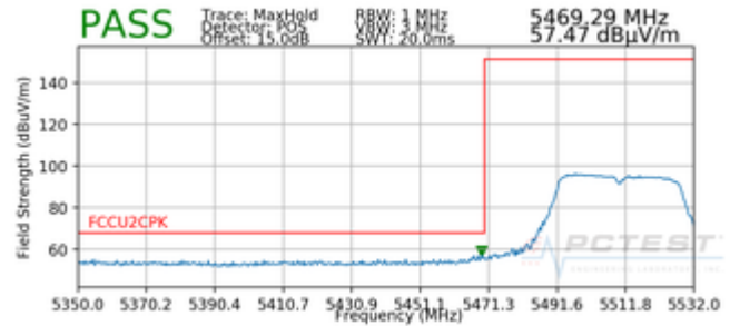
Plot 7-97. Radiated Lower Band Edge Plot SISO ANT1 (Peak – UNII Band 2C)
