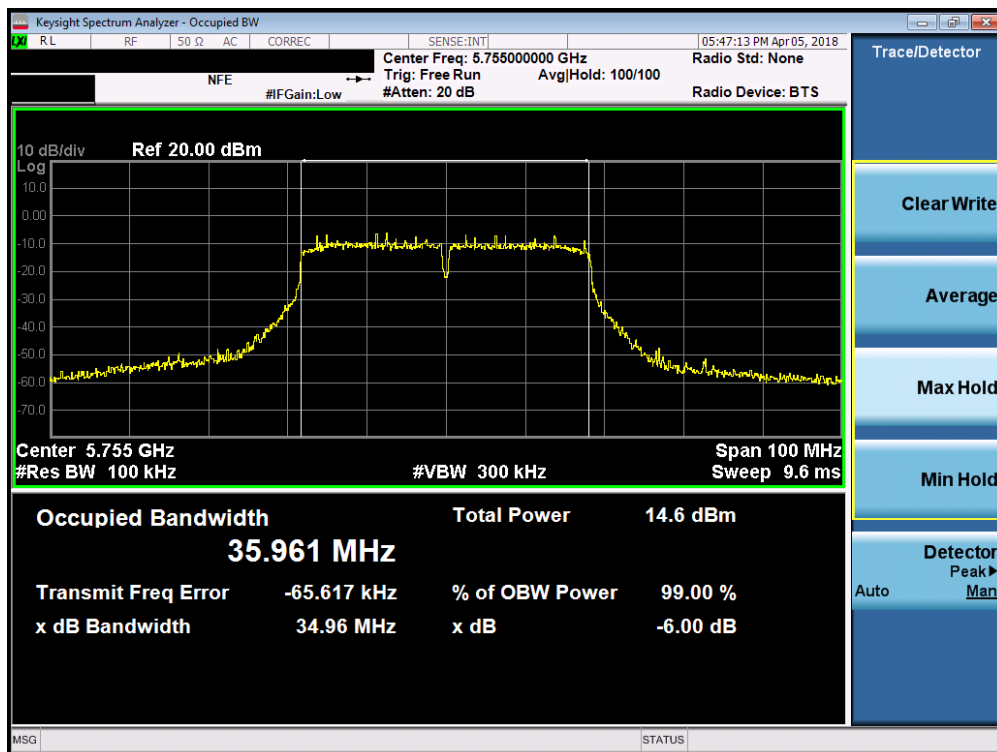
Plot 7-36. 6dB Bandwidth Plot SISO ANT1 (40MHz BW 802.11n (UNII Band 3) – Ch. 151)
