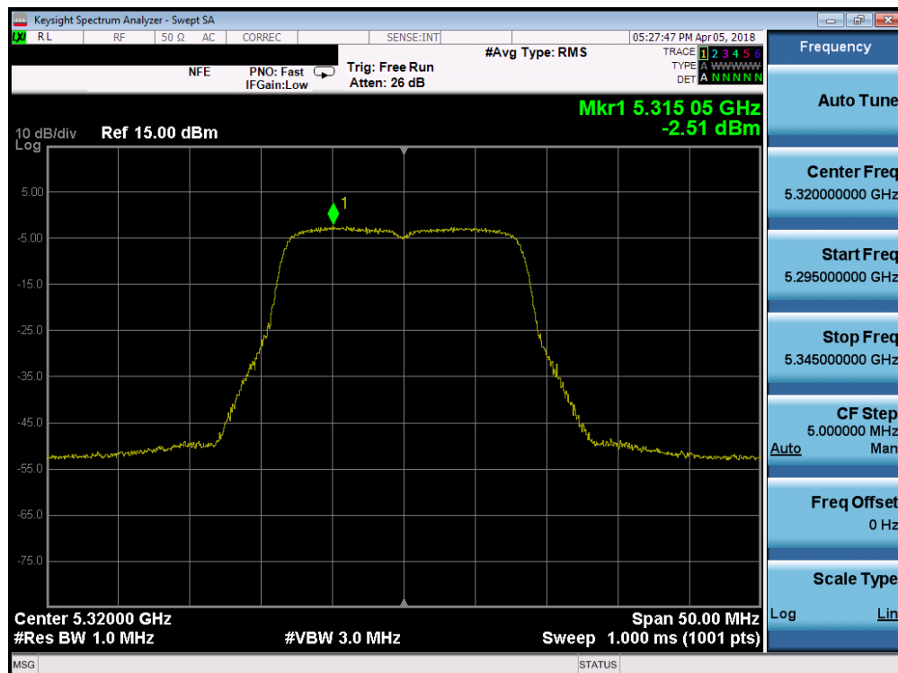
Plot 7-50. Power Spectral Density Plot SISO ANT1 (802.11a (UNII Band 2A) – Ch. 64)
