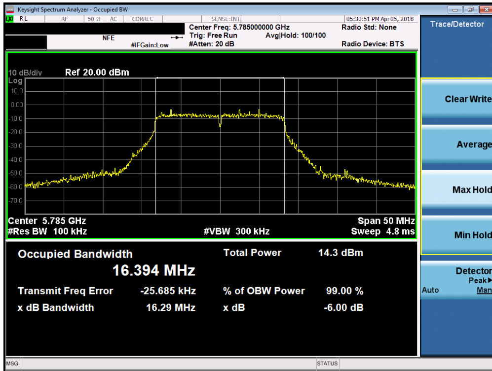
Plot 7-31. 6dB Bandwidth Plot SISO ANT1 (802.11a (UNII Band 3) – Ch. 157)
