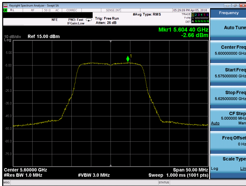
Plot 7-58. Power Spectral Density Plot SISO ANT1 (802.11a (UNII Band 2C) – Ch. 120)
