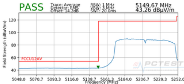
Plot 7-101. Radiated Lower Band Edge Plot SISO ANT1 (Average – UNII Band 1)
