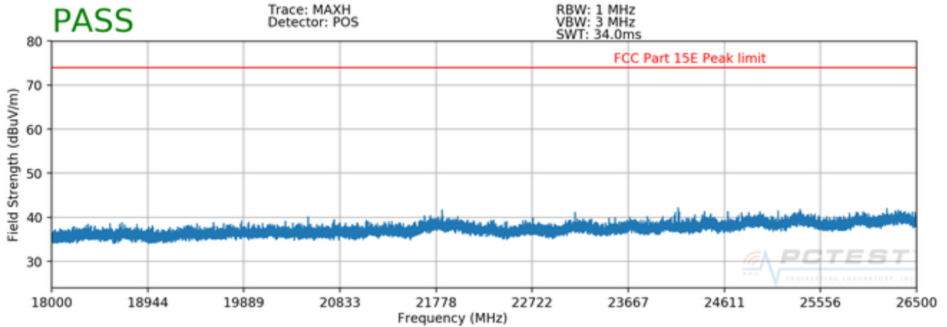
Plot 7-81. Radiated Spurious Plot 18GHz - 26.5GHz SISO ANT1 (802.11a)
