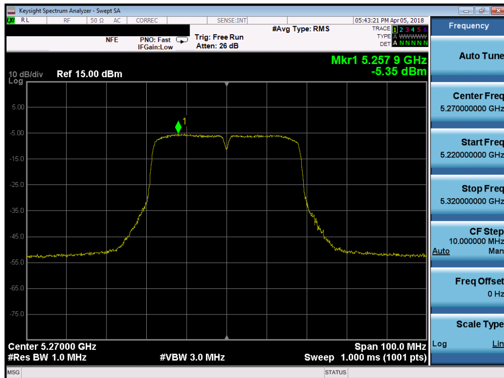
Plot 7-54. Power Spectral Density Plot SISO ANT1 (40MHz BW 802.11n (UNII Band 2A) – Ch. 54)
