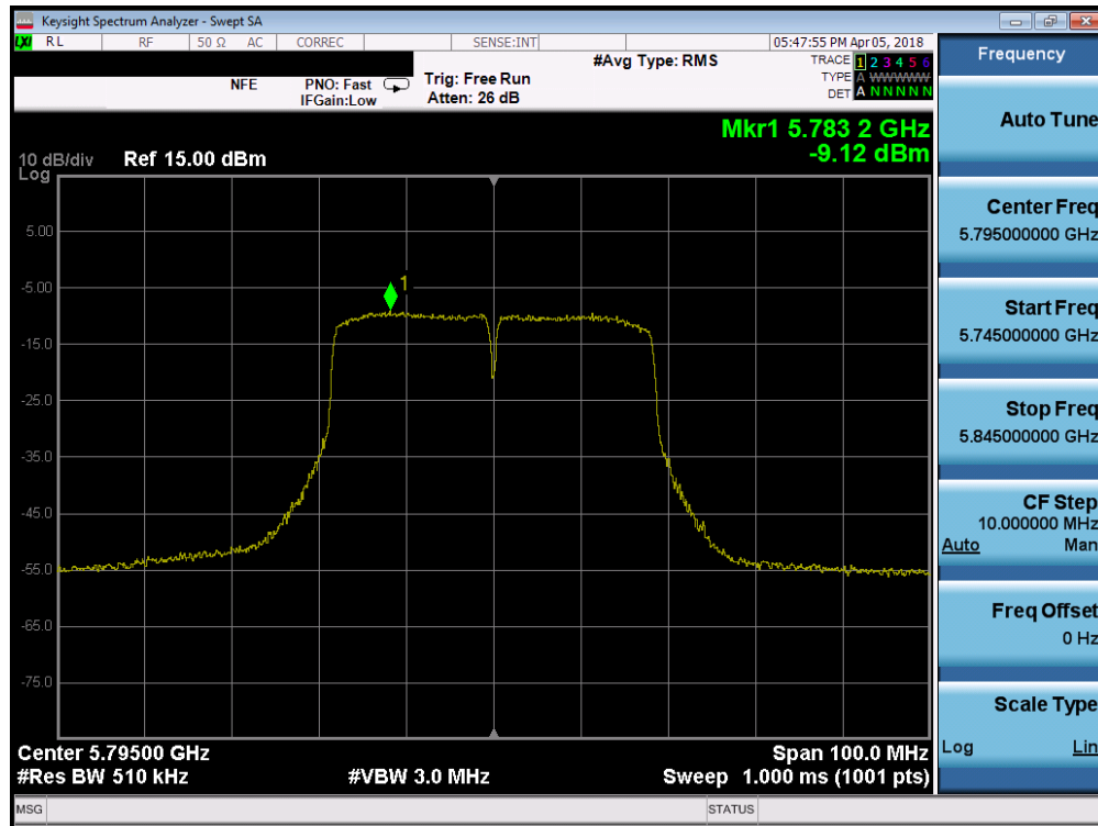
Plot 7-75. Power Spectral Density Plot SISO ANT1 (40MHz BW 802.11n (UNII Band 3) – Ch. 159)
