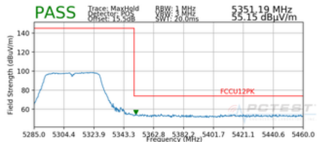
Plot 7-95. Radiated Upper Band Edge Plot SISO ANT1 (Peak – UNII Band 2A)
