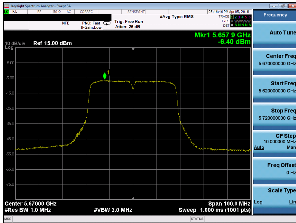
Plot 7-65. Power Spectral Density Plot SISO ANT1 (40MHz BW 802.11n (UNII Band 2C) – Ch. 134)
