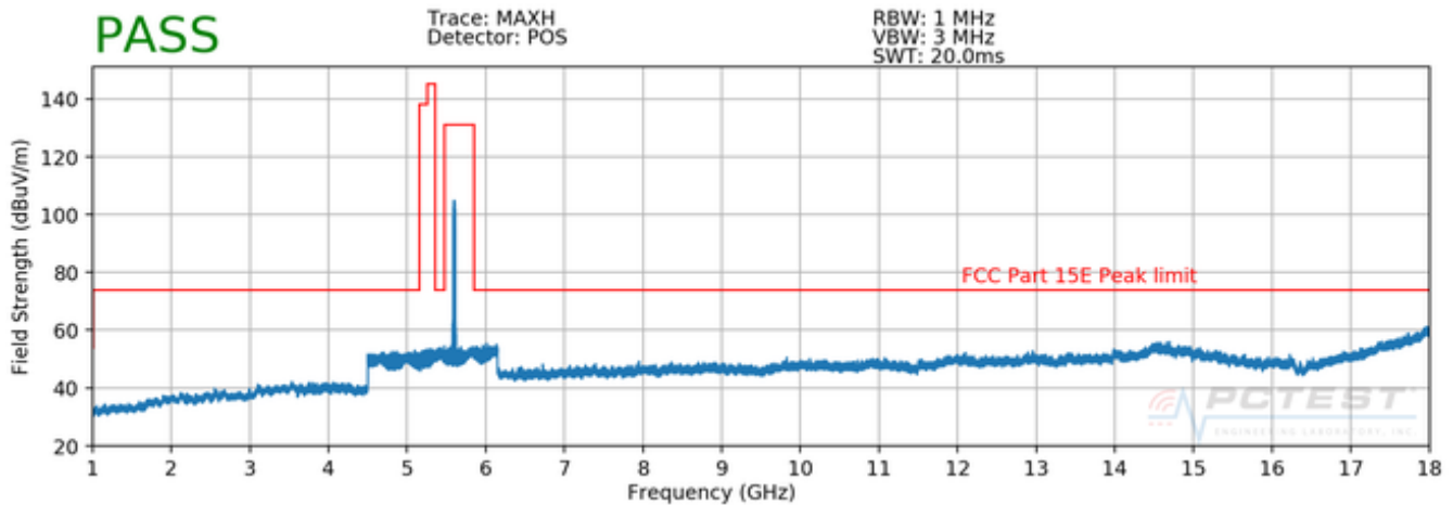
Plot 7-79. Radiated Spurious Plot above 1GHz SISO ANT1 (802.11a – U2C Ch. 120)
