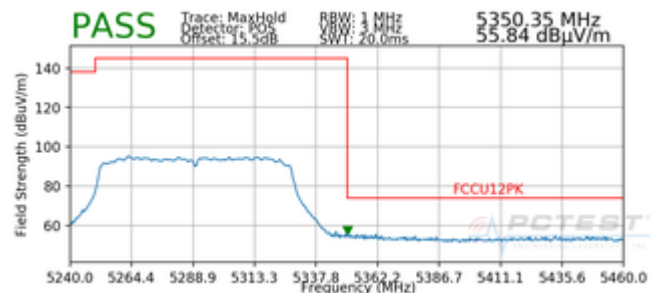
Plot 7-104. Radiated Upper Band Edge Plot SISO ANT1 (Peak – UNII Band 2A)
