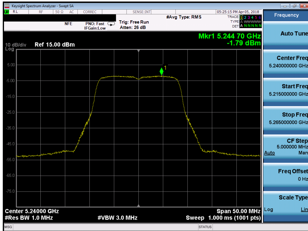
Plot 7-41. Power Spectral Density Plot SISO ANT1 (802.11a (UNII Band 1) – Ch. 48)
