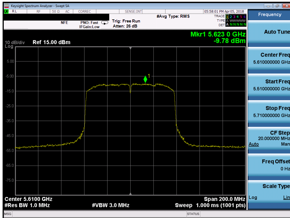
Plot 7-67. Power Spectral Density Plot SISO ANT1 (80MHz BW 802.11ac (UNII Band 2C) – Ch. 122)
