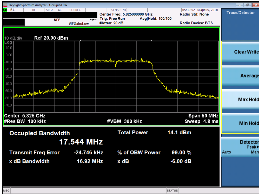
Plot 7-35. 6dB Bandwidth Plot SISO ANT1 (20MHz BW 802.11n (UNII Band 3) – Ch. 165)
