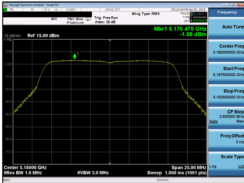
Plot 7-39. Power Spectral Density Plot SISO ANT1 (802.11a (UNII Band 1) – Ch. 36)
