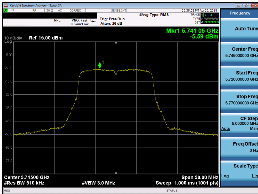
Plot 7-71. Power Spectral Density Plot SISO ANT1 (20MHz BW 802.11n (UNII Band 3) – Ch. 149)
