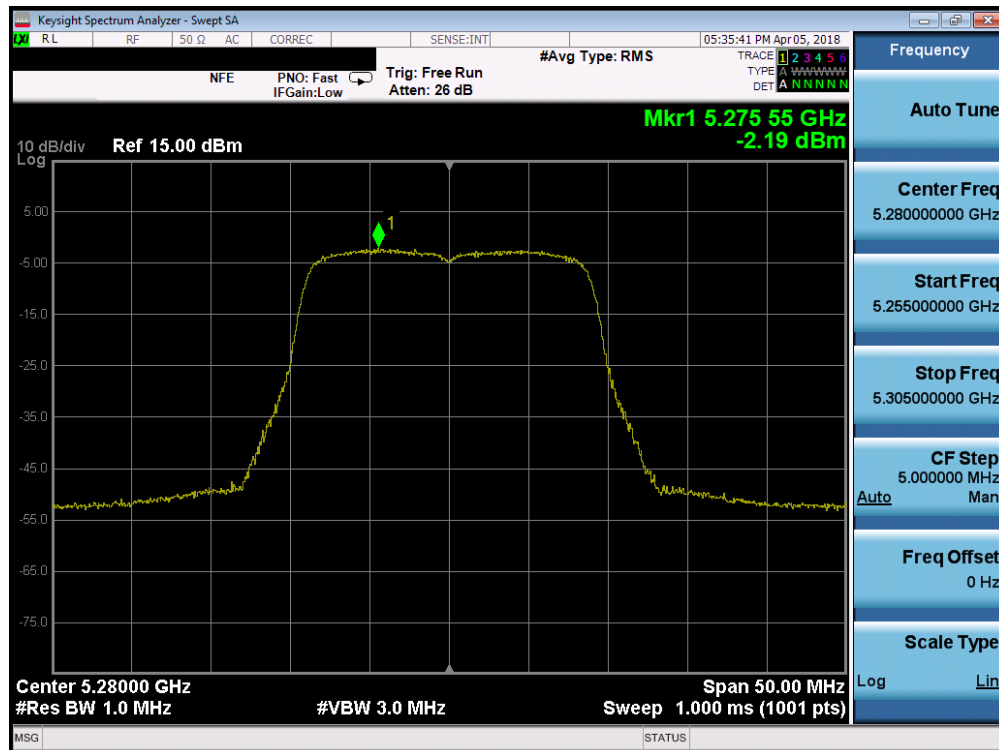
Plot 7-52. Power Spectral Density Plot SISO ANT1 (20MHz BW 802.11n (UNII Band 2A) – Ch. 56)
