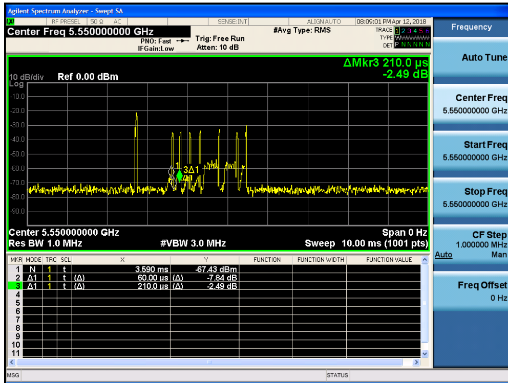
Figure 5-2. Band 2C Pulse Width
