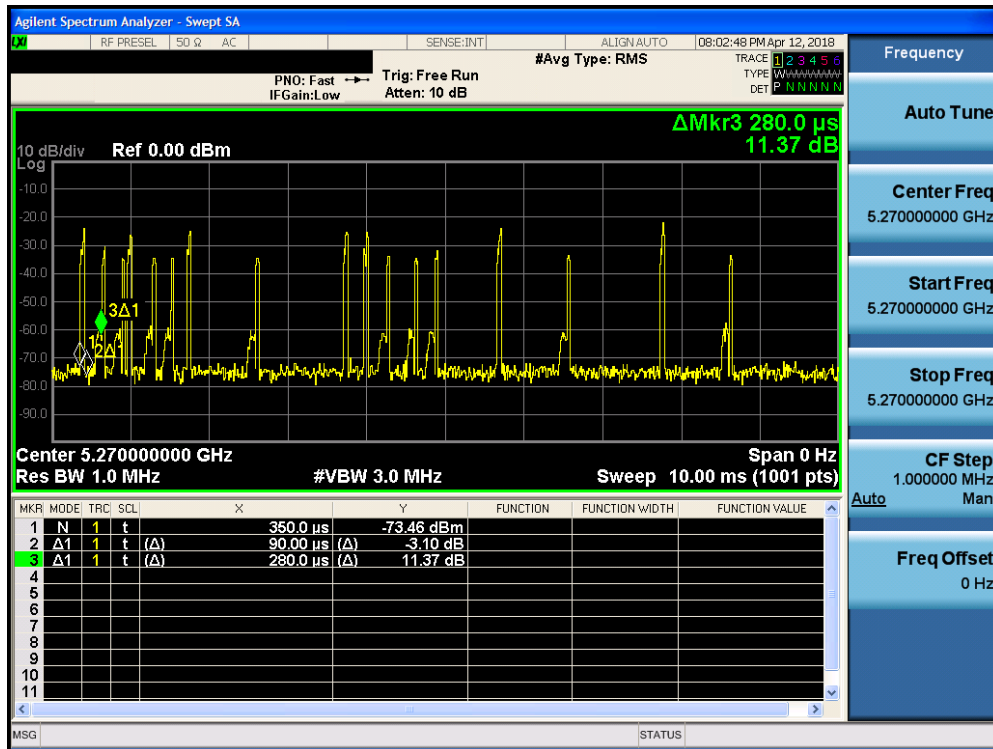
Figure 5-1. Band 2A Channel Loading
