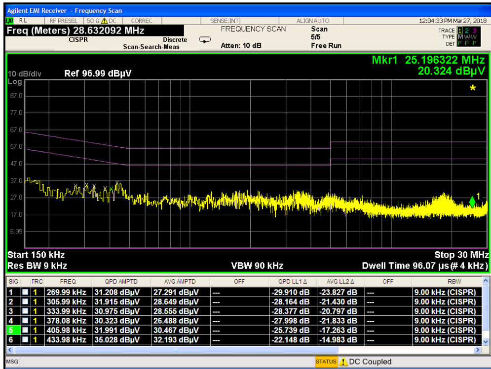
Plot 7-8. Line-Conducted Test Plot (L1) (with Antenna terminated)
