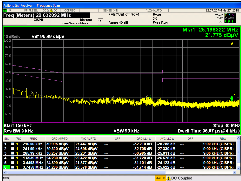
Plot 7-9. Line-Conducted Test Plot (N) (with Antenna terminated)
