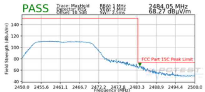
Plot 7-38. Radiated Restricted Upper Band Edge Measurement (Peak)
