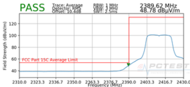
Plot 7-35. Radiated Restricted Lower Band Edge Measurement (Average)
