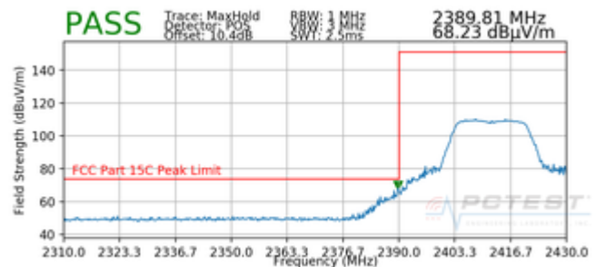
Plot 7-36. Radiated Restricted Lower Band Edge Measurement (Peak)
