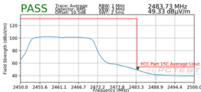
Plot 7-37. Radiated Restricted Upper Band Edge Measurement (Average)
