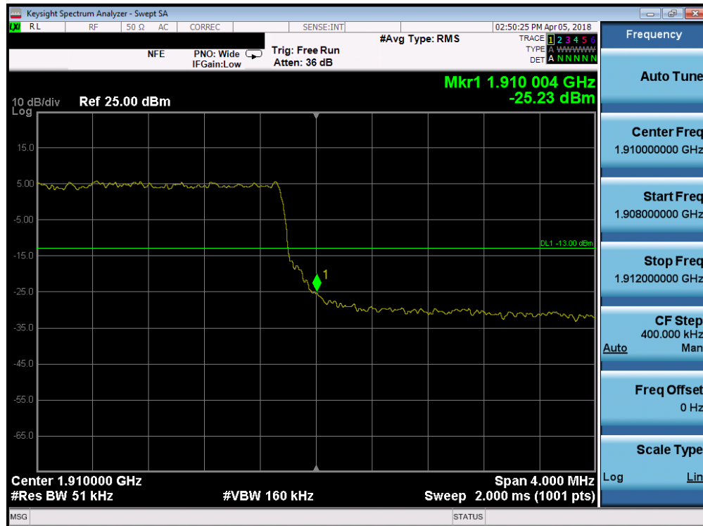
Plot 7-129. Upper Band Edge Plot (Band 2 - 5.0MHz QPSK - Full RB Configuration)
