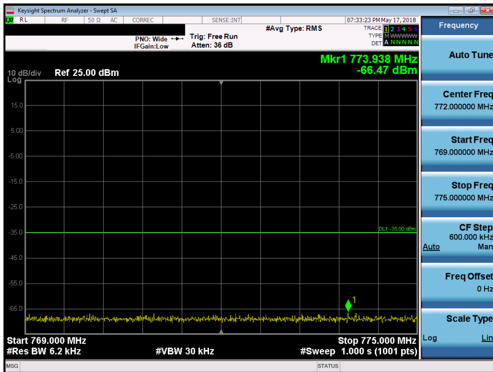
Plot 7-13. Lower Emission Mask Plot (LTE B14 10MHz QPSK – RB Size 50)
