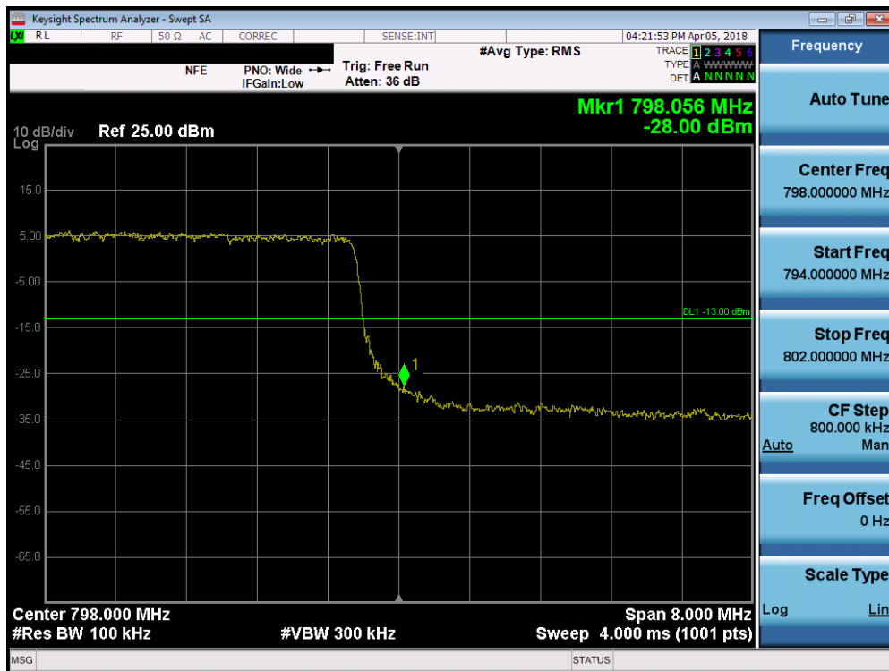
Plot 7-14. Upper Band Edge Plot (LTE B14 10MHz QPSK – RB Size 50)
