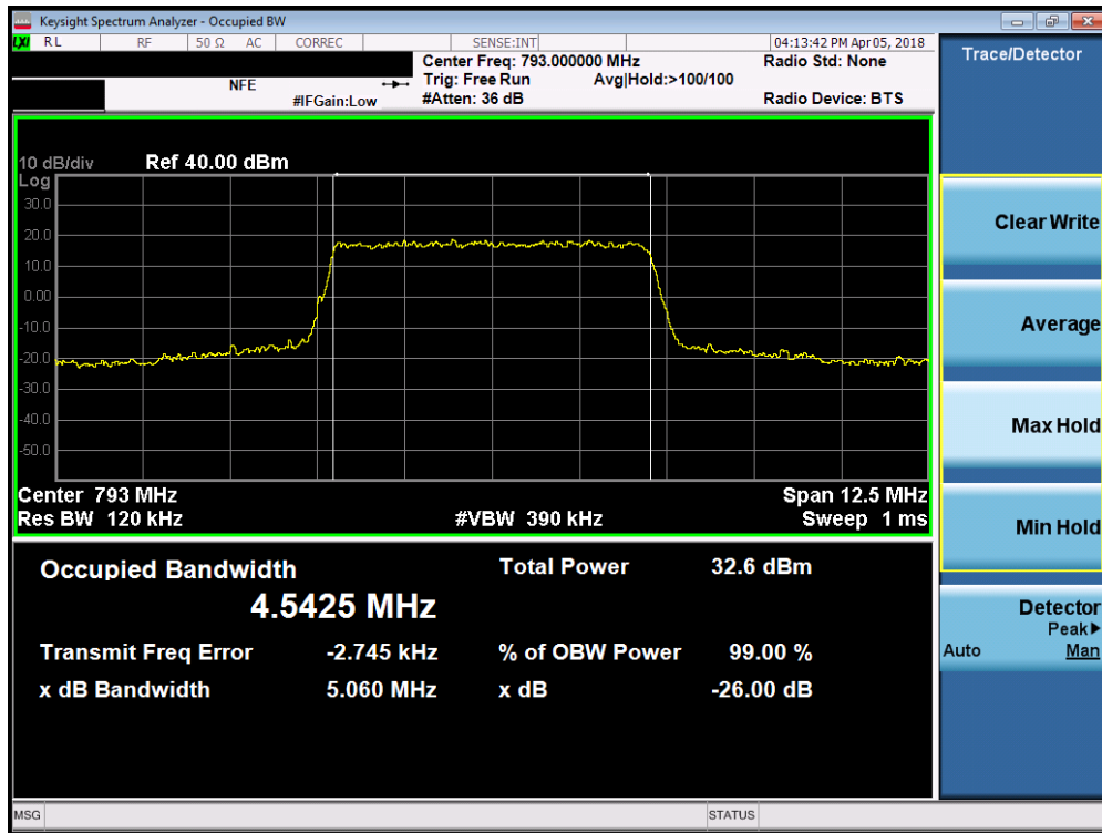
Plot 7-1. Occupied Bandwidth Plot (LTE B14 - 5.0MHz QPSK – RB Size 25)
