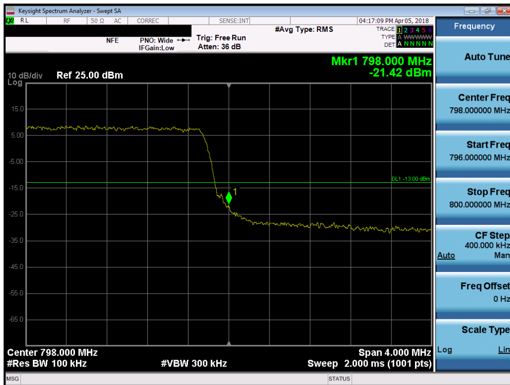
Plot 7-10. Upper Band Edge Plot (LTE B14 5MHz QPSK – RB Size 25)
