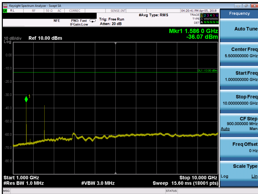
Plot 7-7. Conducted Spurious Plot (LTE B14 – 10.0MHz QPSK – RB Size 1, RB Offset 0)
