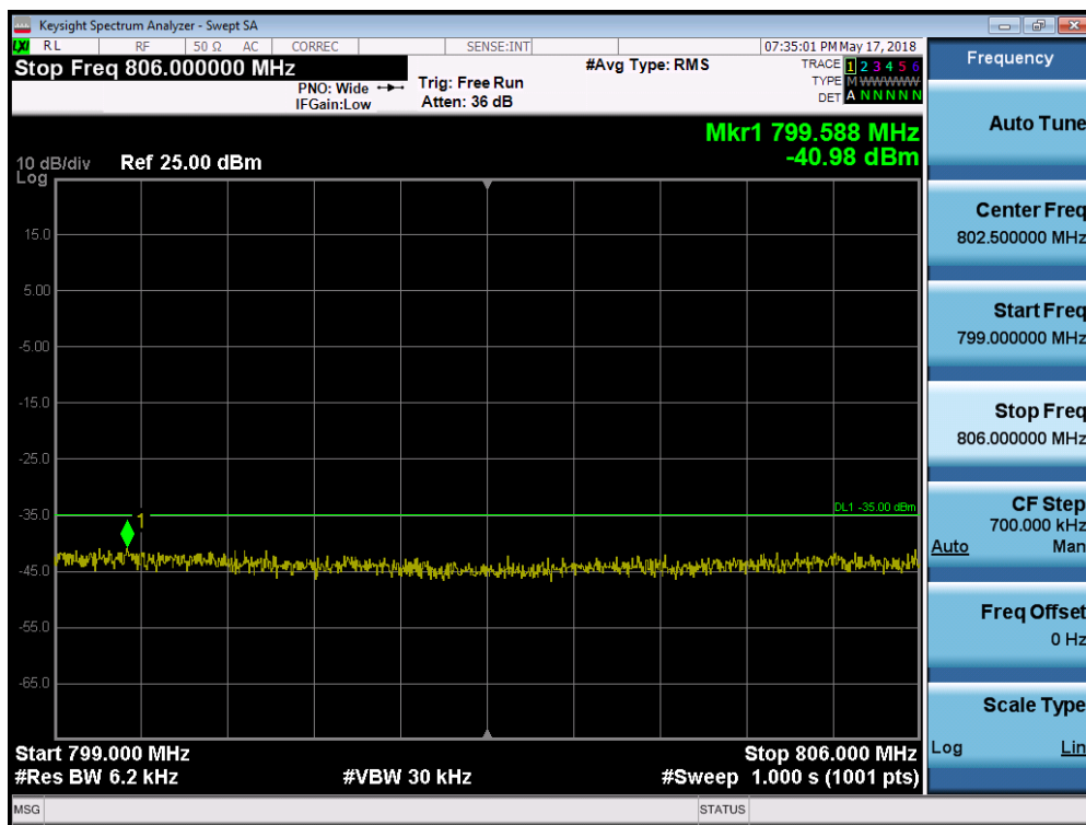
Plot 7-15. Upper Emission Mask Plot (LTE B14 10MHz QPSK – RB Size 50)
