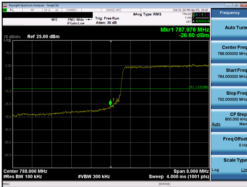
Plot 7-12. Lower Band Edge Plot (LTE B14 10MHz QPSK – RB Size 50)
