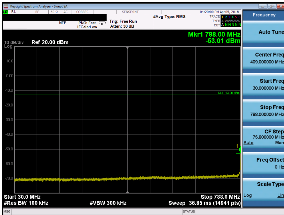
Plot 7-5. Conducted Spurious Plot (LTE B14 – 10.0MHz QPSK – RB Size 1, RB Offset 0)
