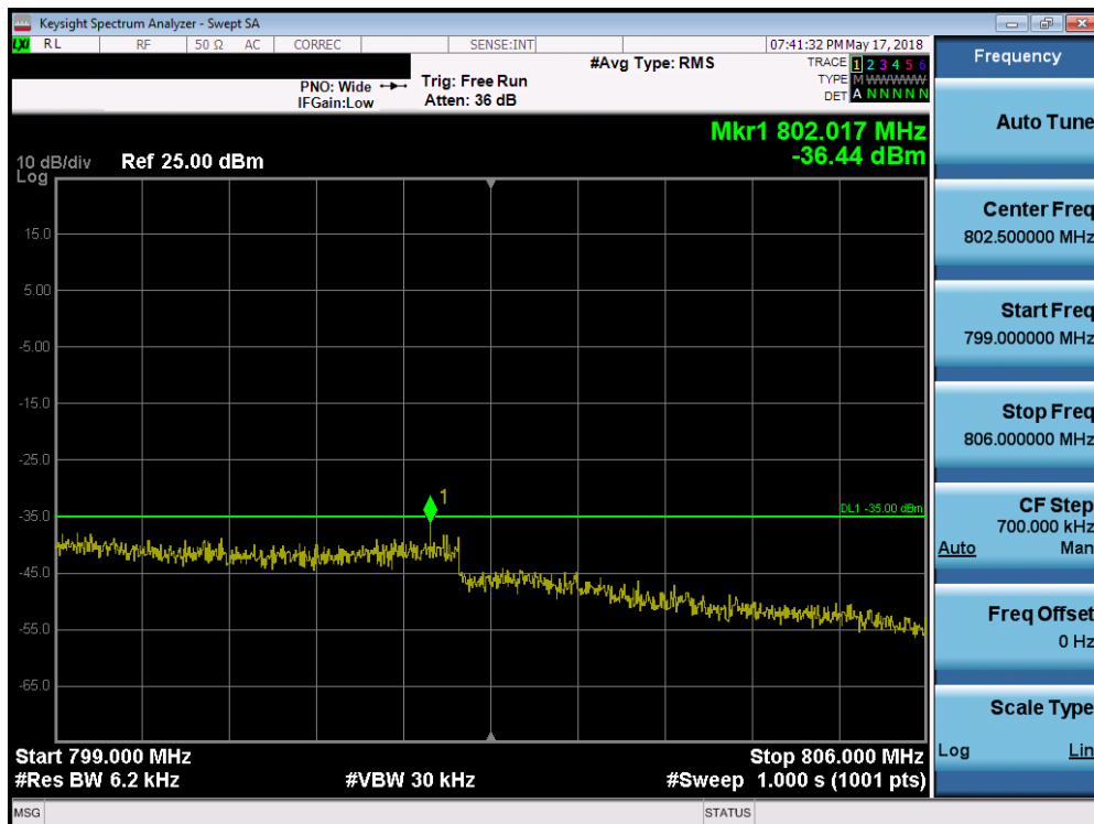
Plot 7-11. Upper Emission Mask Plot (LTE B14 5MHz QPSK – RB Size 25)
