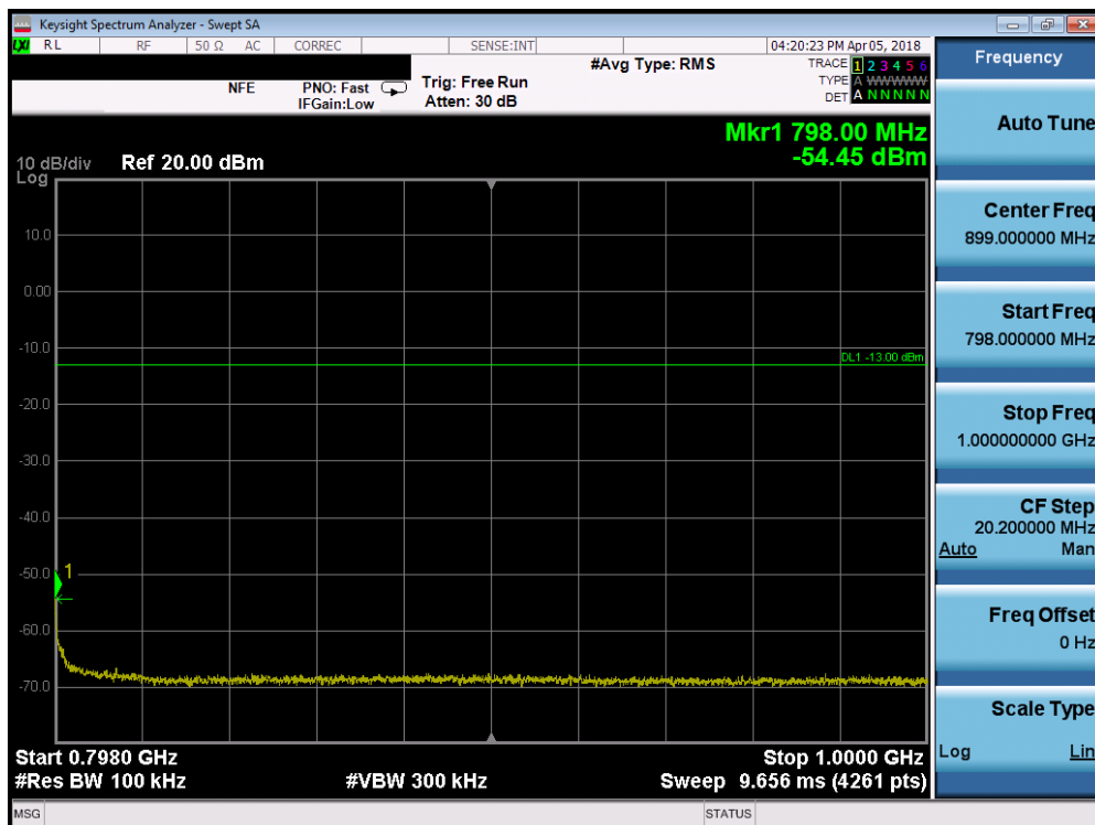
Plot 7-6. Conducted Spurious Plot (LTE B14 – 10.0MHz QPSK – RB Size 1, RB Offset 0)
