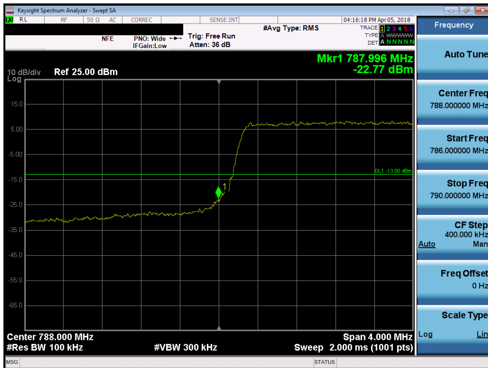
Plot 7-8. Lower Band Edge Plot (LTE B14 5MHz QPSK – RB Size 25)
