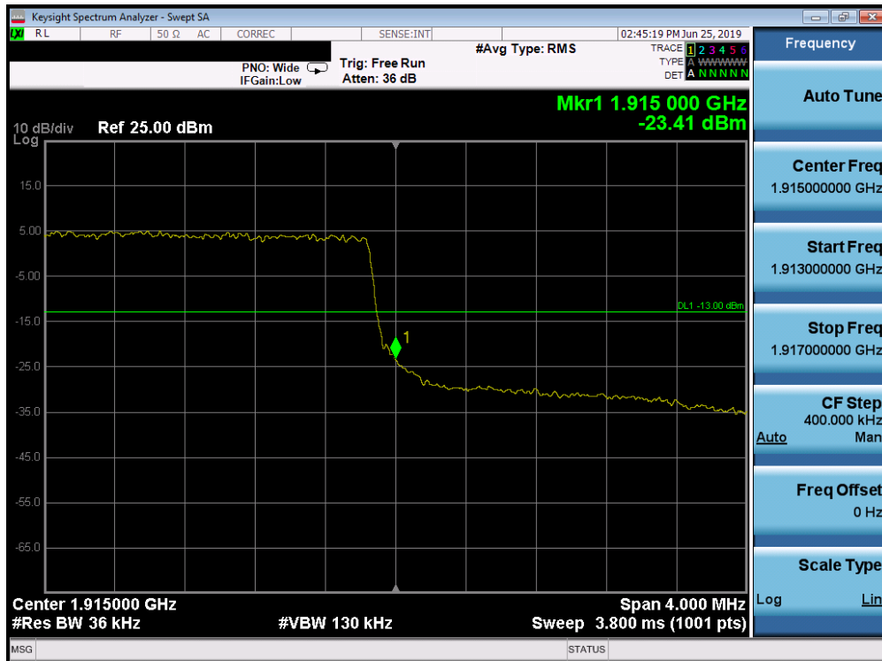
Plot 7-245. Upper Band Edge Plot (Band 25 - 3.0MHz QPSK - Full RB Configuration)
