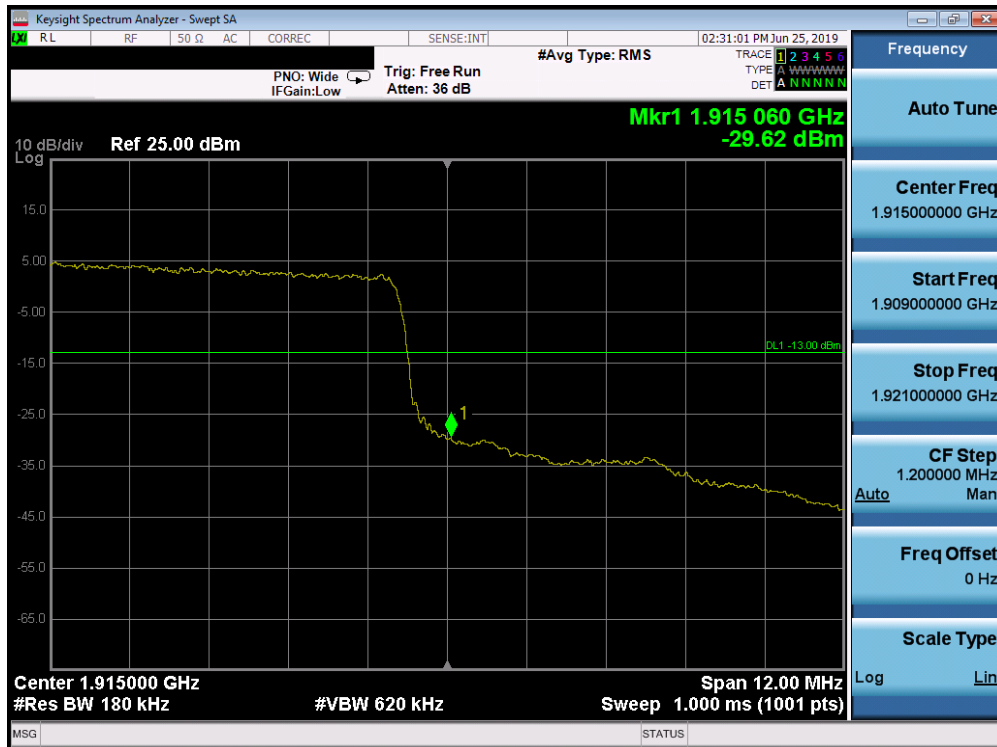
Plot 7-263. Upper Band Edge Plot (Band 25 - 15.0MHz QPSK - Full RB Configuration)
