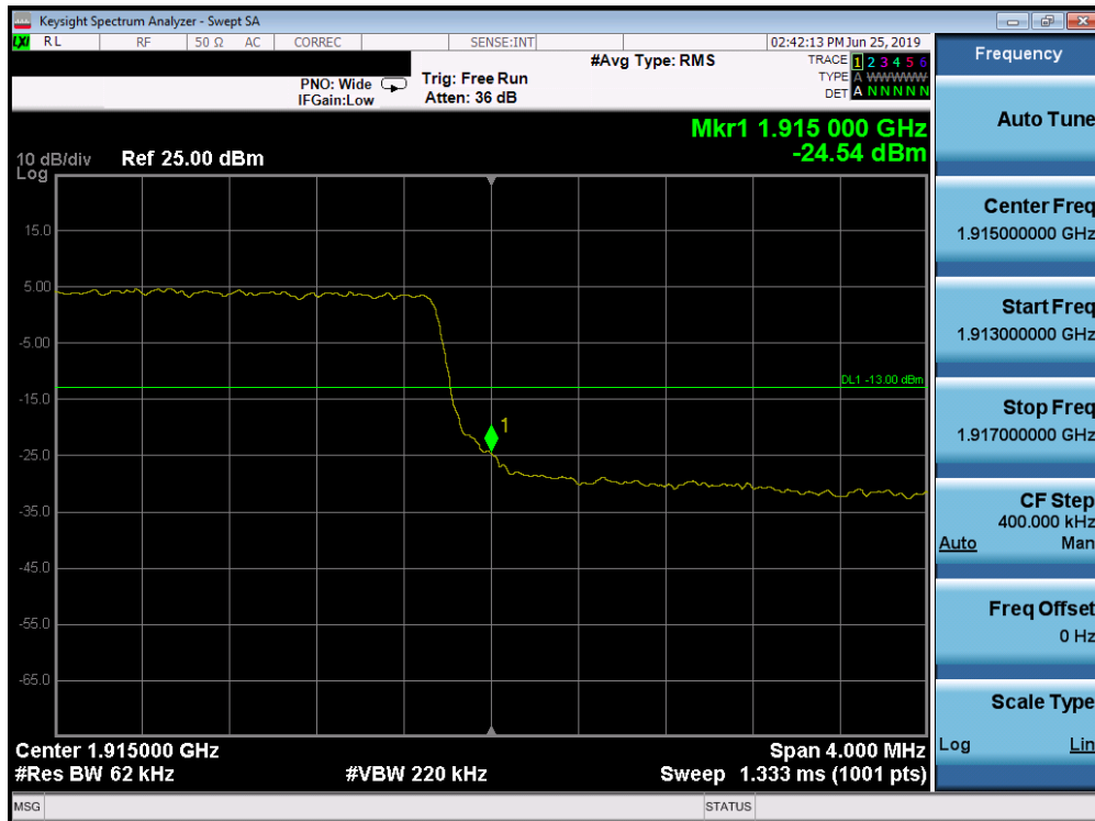
Plot 7-251. Upper Band Edge Plot (Band 25 - 5.0MHz QPSK - Full RB Configuration)
