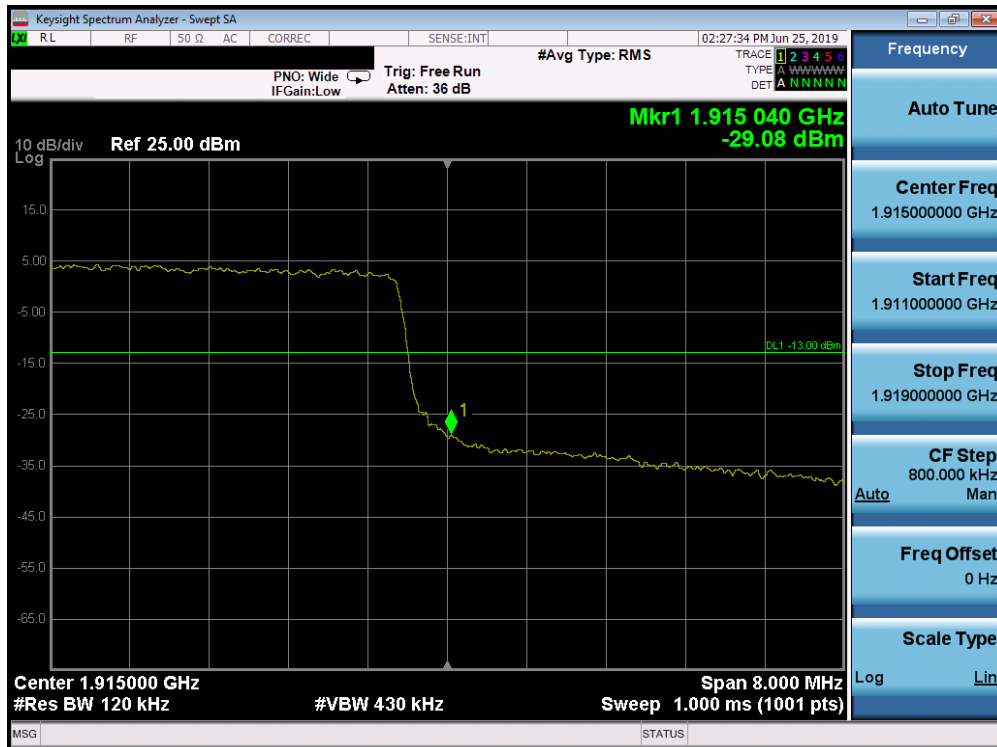
Plot 7-257. Upper Band Edge Plot (Band 25 - 10.0MHz QPSK - Full RB Configuration)
