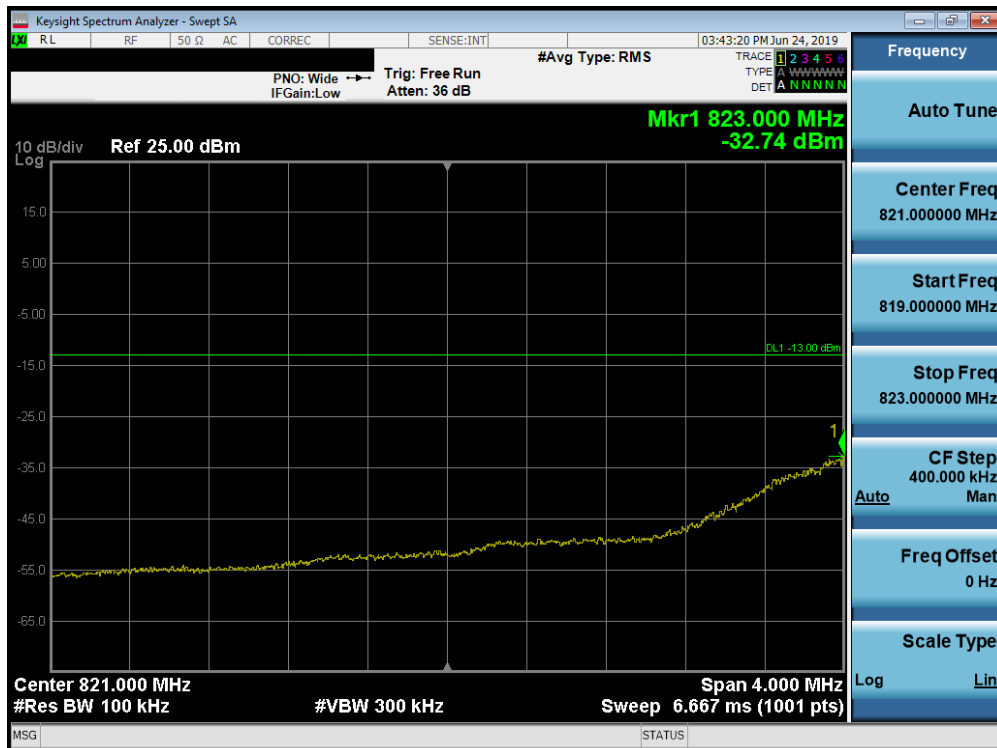
Plot 7-188. Lower Extended Band Edge Plot (Band 26/5 - 1.4MHz QPSK - Full RB Configuration)
