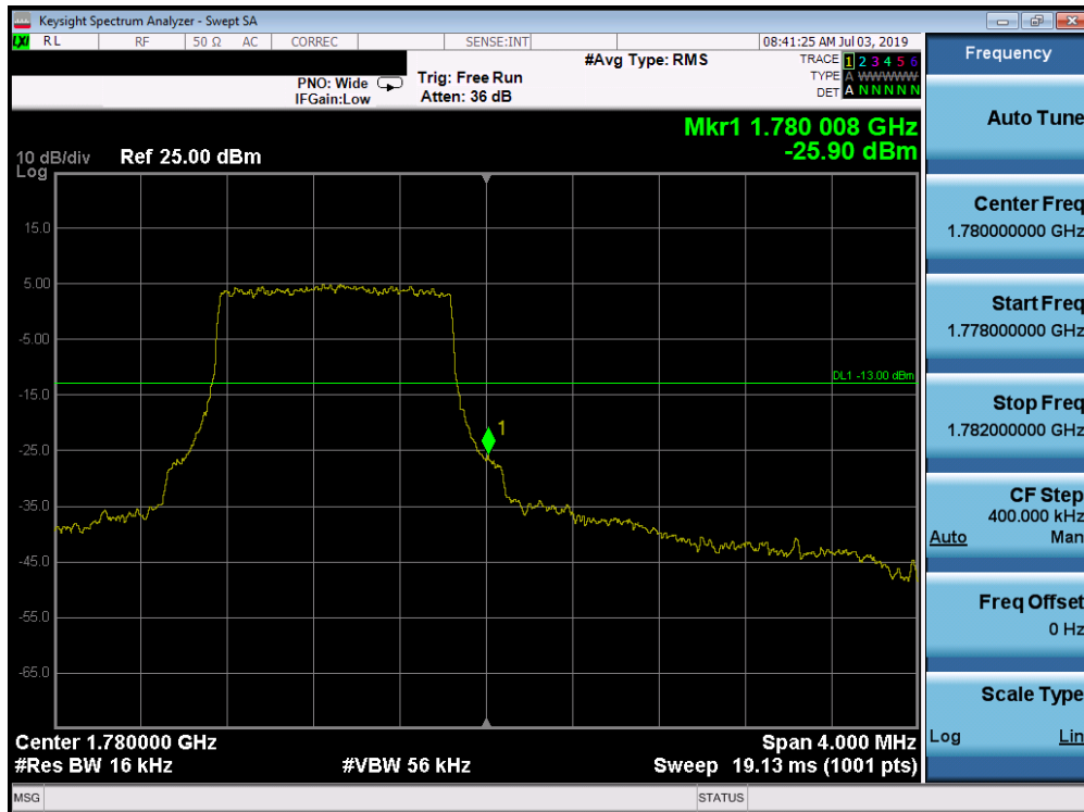
Plot 7-203. Upper Band Edge Plot (Band 66 - 1.4MHz QPSK - Full RB Configuration)
