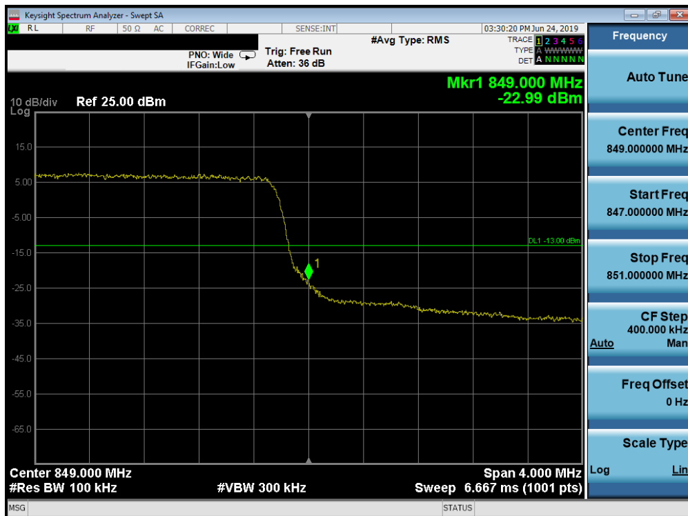
Plot 7-194. Upper Band Edge Plot (Band 26/5 - 5.0MHz QPSK - Full RB Configuration)
