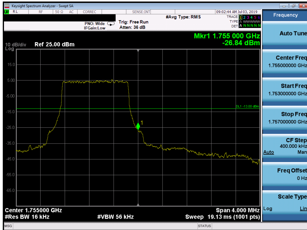
Plot 7-201. Upper Band Edge Plot (Band 4 - 1.4MHz QPSK - Full RB Configuration)
