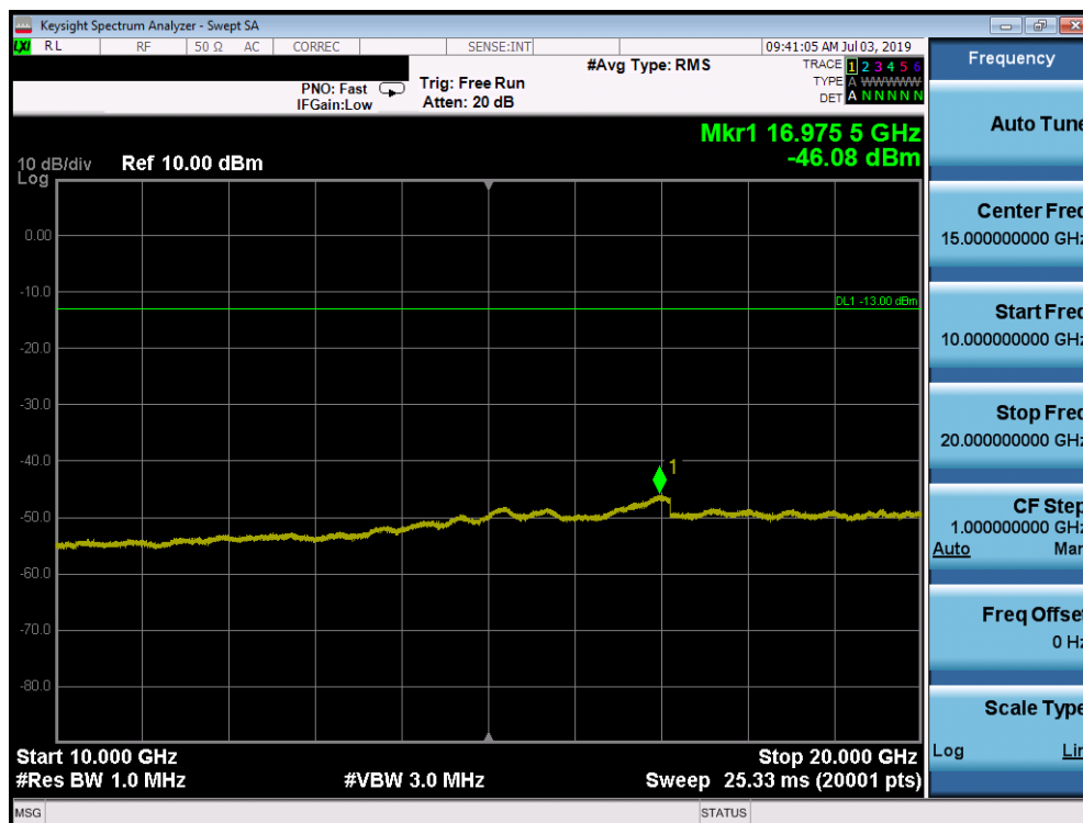
Plot 7-60. Conducted Spurious Plot (AWS WCDMA Mode - Mid Channel)
