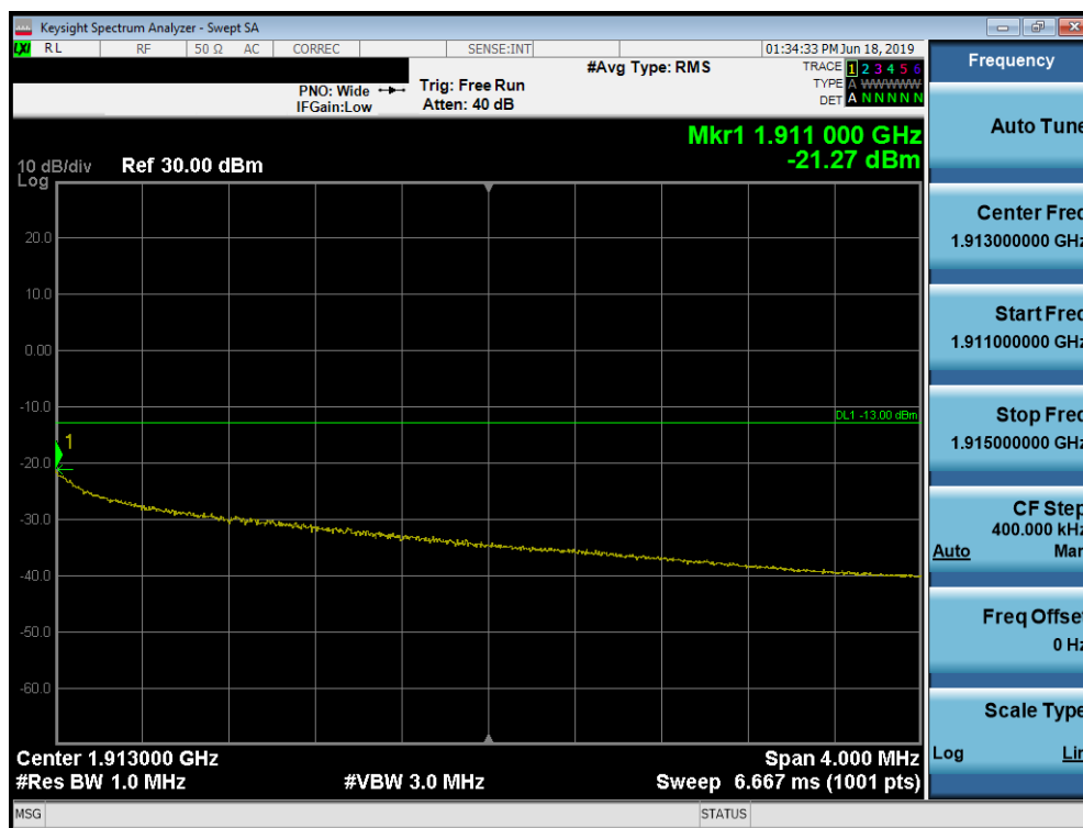
Plot 7-86. 4MHz Span Plot (PCS CDMA Mode - High Channel)
