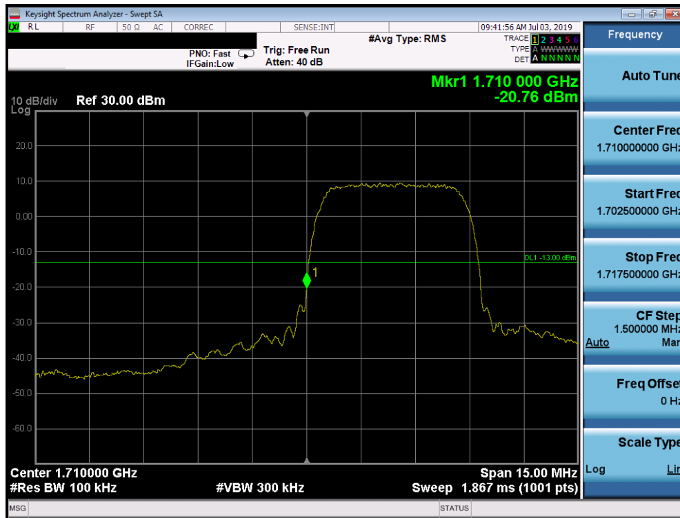
Plot 7-89. Band Edge Plot (AWS WCDMA Mode - Low Channel)
