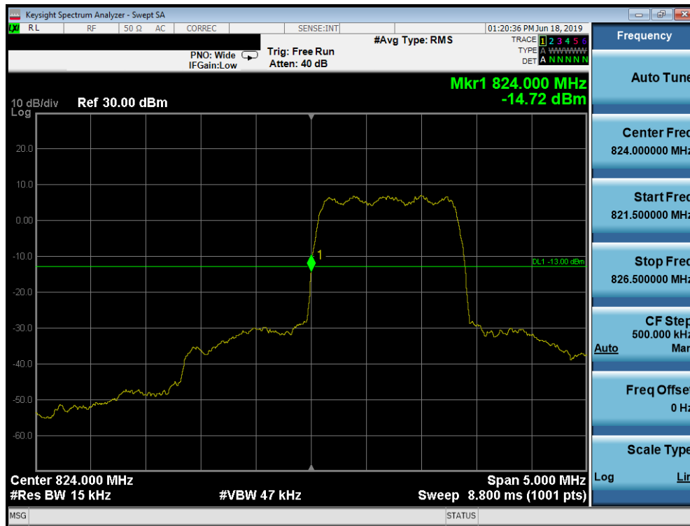
Plot 7-79. Band Edge Plot (Cellular CDMA Mode - Low Channel)
