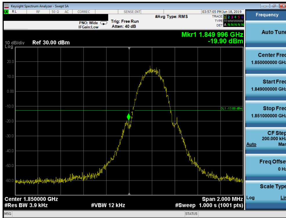
Plot 7-75. Band Edge Plot (PCS GSM Mode - Low Channel)
