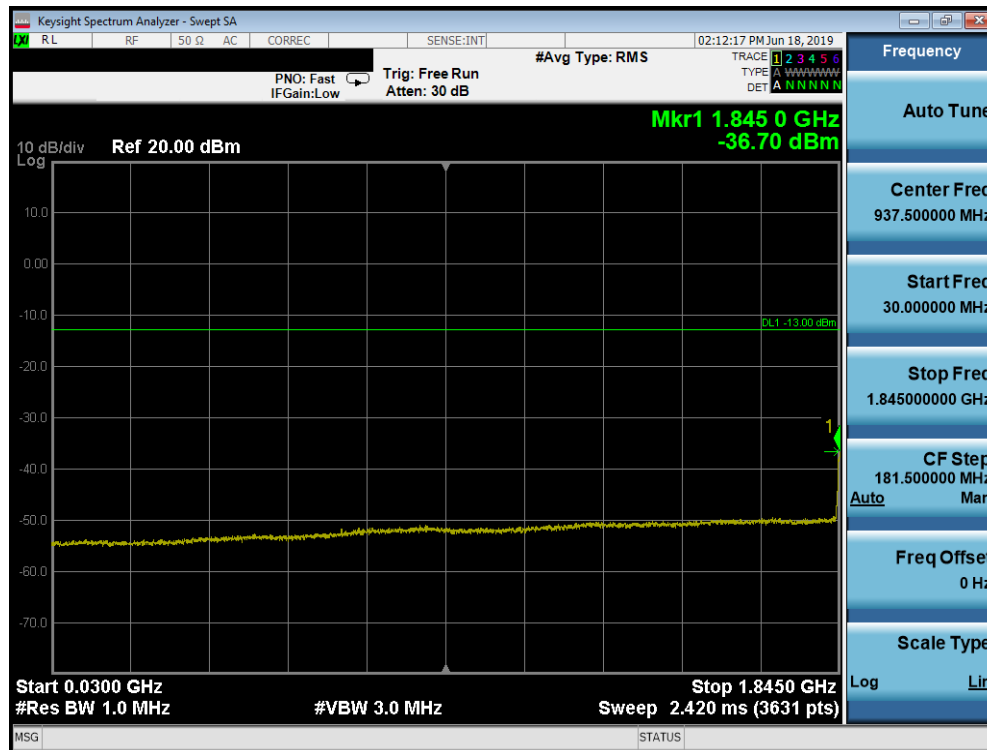
Plot 7-64. Conducted Spurious Plot (PCS WCDMA Mode - Low Channel)
