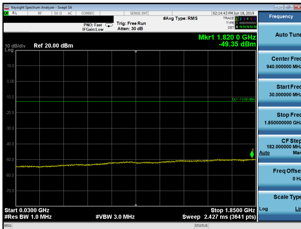
Plot 7-70. Conducted Spurious Plot (PCS WCDMA Mode - High Channel)
