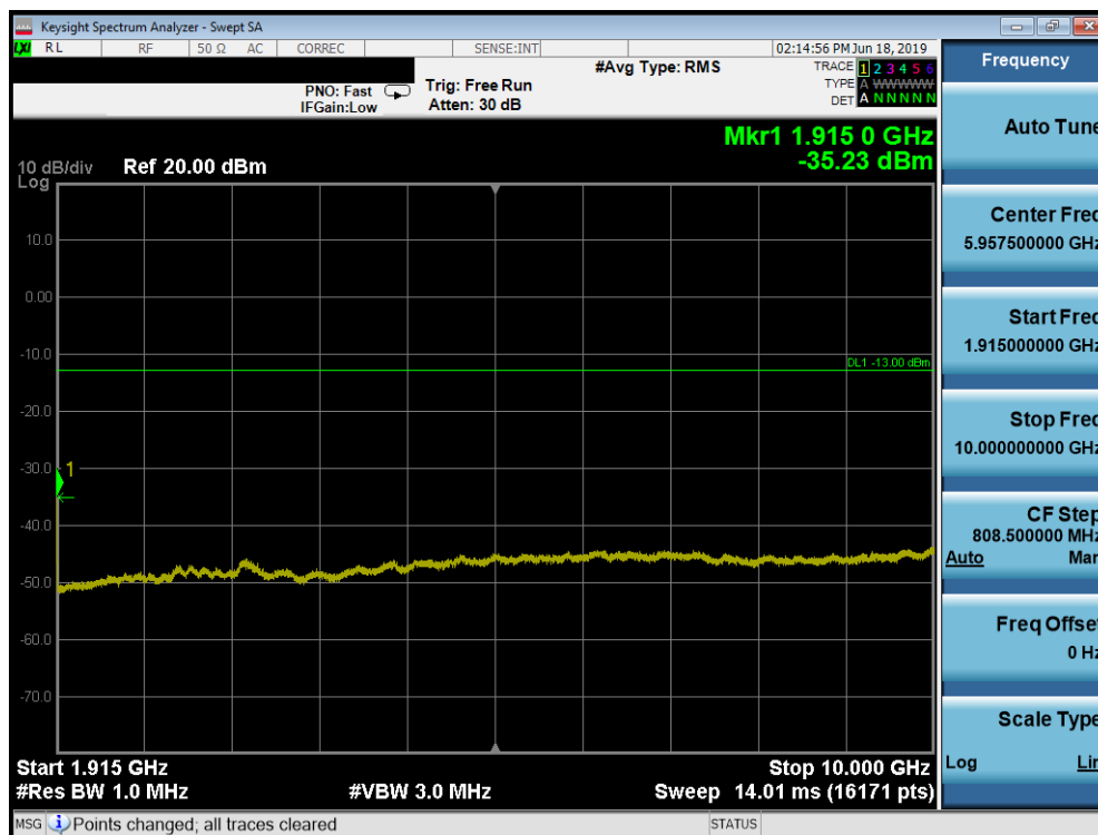
Plot 7-71. Conducted Spurious Plot (PCS WCDMA Mode - High Channel)
