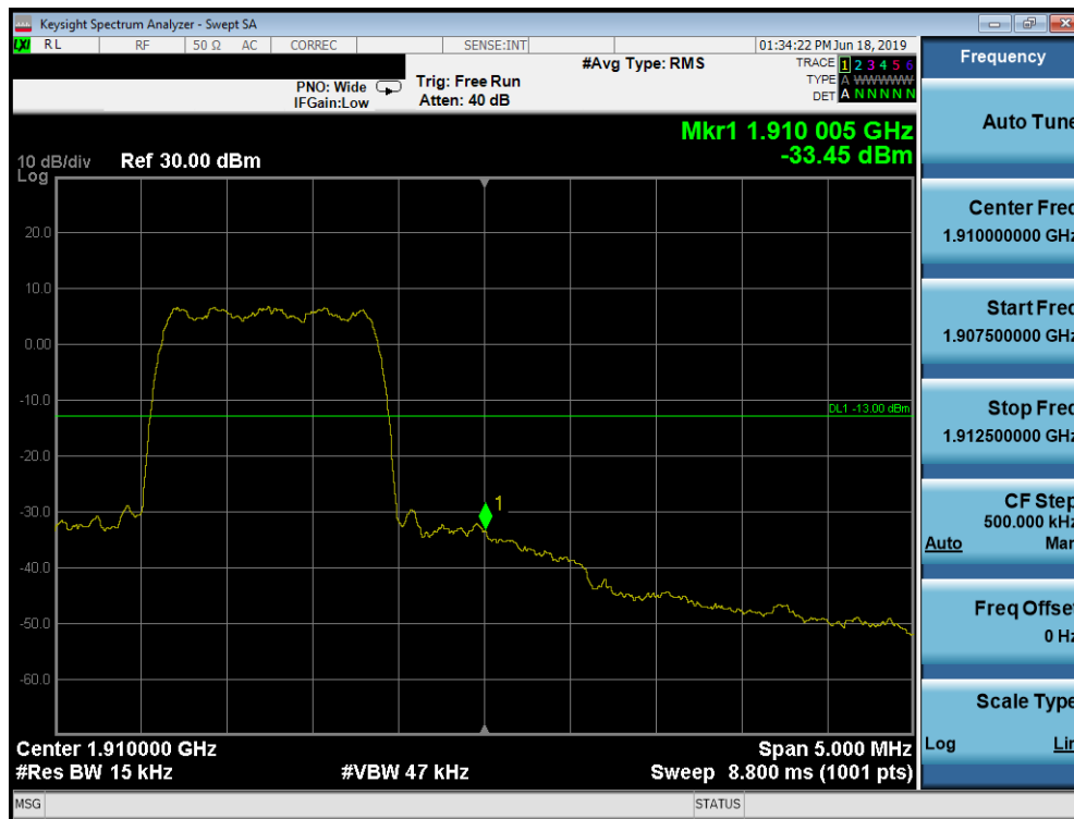
Plot 7-85. Band Edge Plot (PCS CDMA Mode - High Channel)
