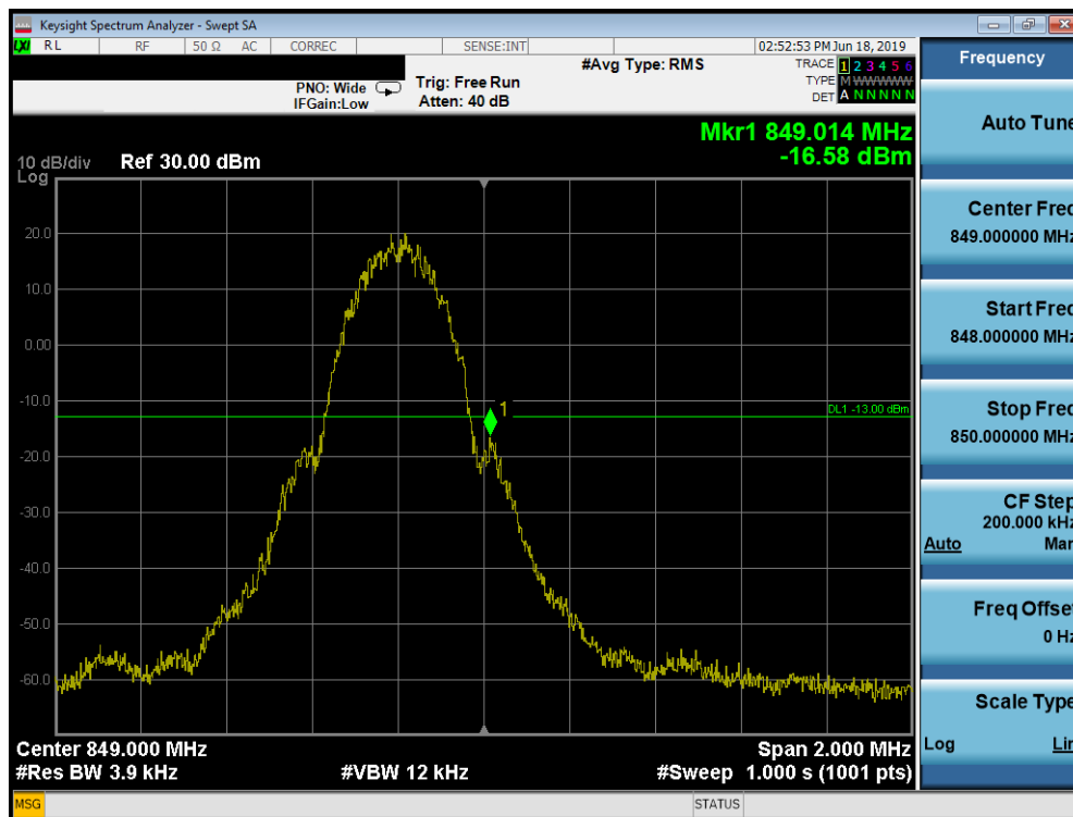
Plot 7-74. Band Edge Plot (Cellular GSM Mode - High Channel)
