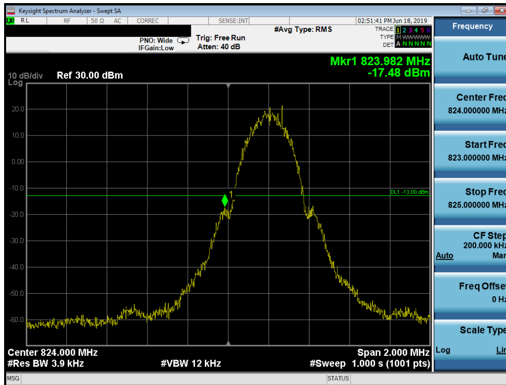
Plot 7-73. Band Edge Plot (Cellular GSM Mode - Low Channel)
