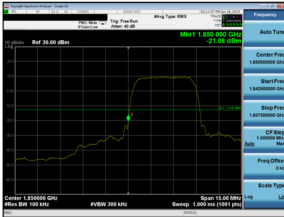
Plot 7-93. Band Edge Plot (PCS WCDMA Mode - Low Channel)
