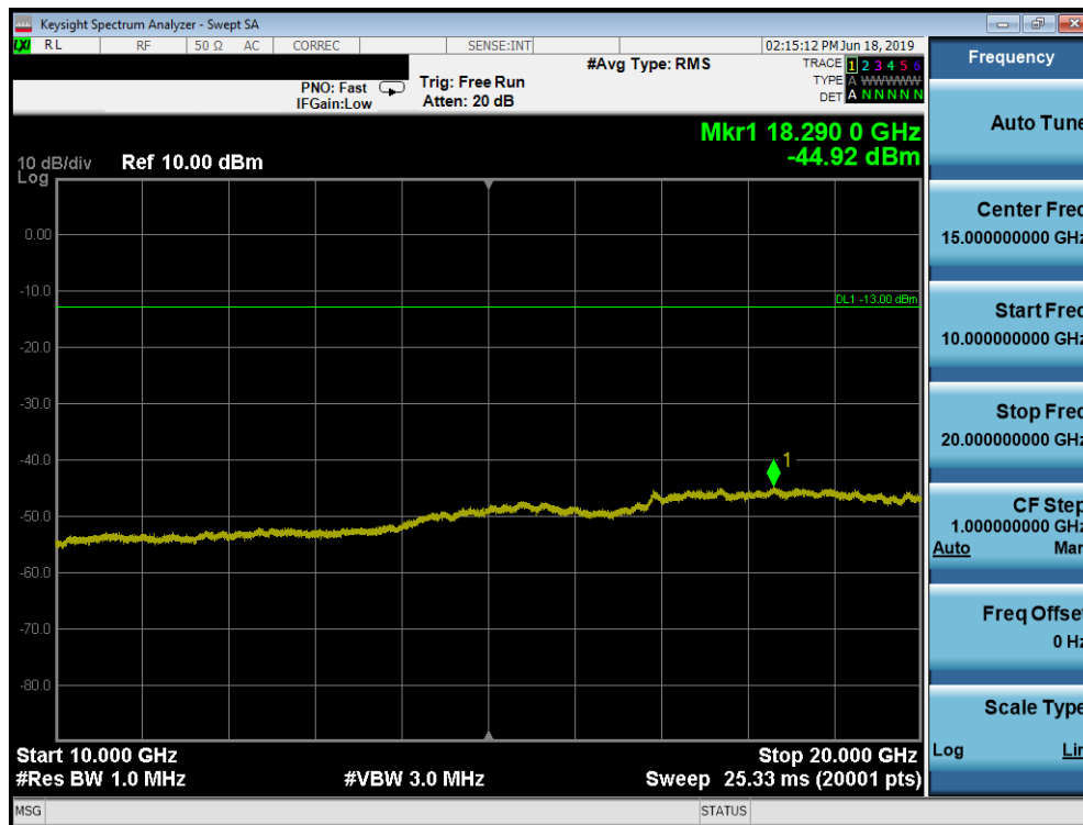
Plot 7-72. Conducted Spurious Plot (PCS WCDMA Mode - High Channel)
