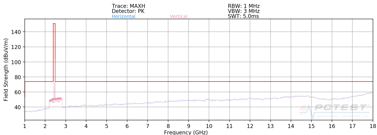
Plot 7-2. Radiated Spurious Plot above 1GHz (BT- Ch. 39)
