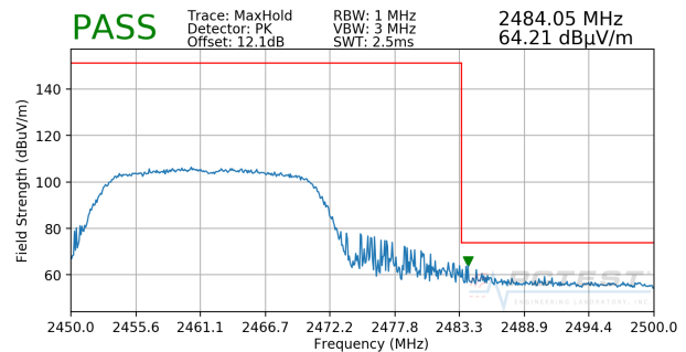
Plot 7-12. Radiated Restricted Upper Band Edge Measurement (Peak)
