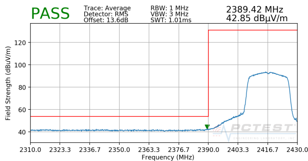
Plot 7-7. Radiated Restricted Lower Band Edge Measurement (Average)
