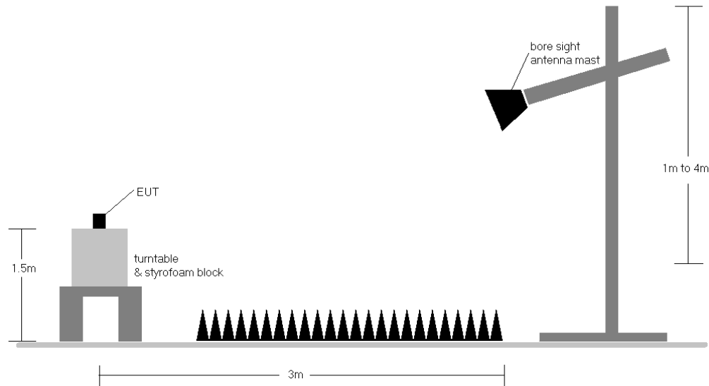
Figure 7-1. Test Instrument & Measurement Setup
