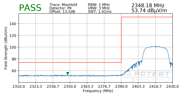
Plot 7-8. Radiated Restricted Lower Band Edge Measurement (Peak)
