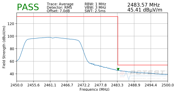
Plot 7-11. Radiated Restricted Upper Band Edge Measurement (Average)
