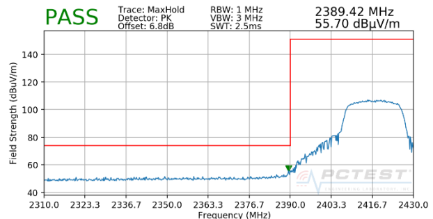
Plot 7-44. Radiated Restricted Upper Band Edge Measurement (Peak)
