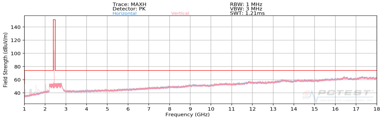
Plot 7-43. Radiated Spurious Plot above 1GHz (BT – Ch. 39)
