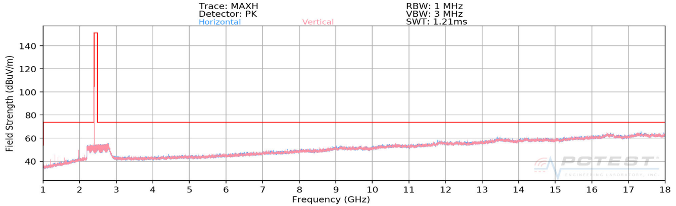
Plot 7-42. Radiated Spurious Plot above 1GHz (BT – Ch. 0)
