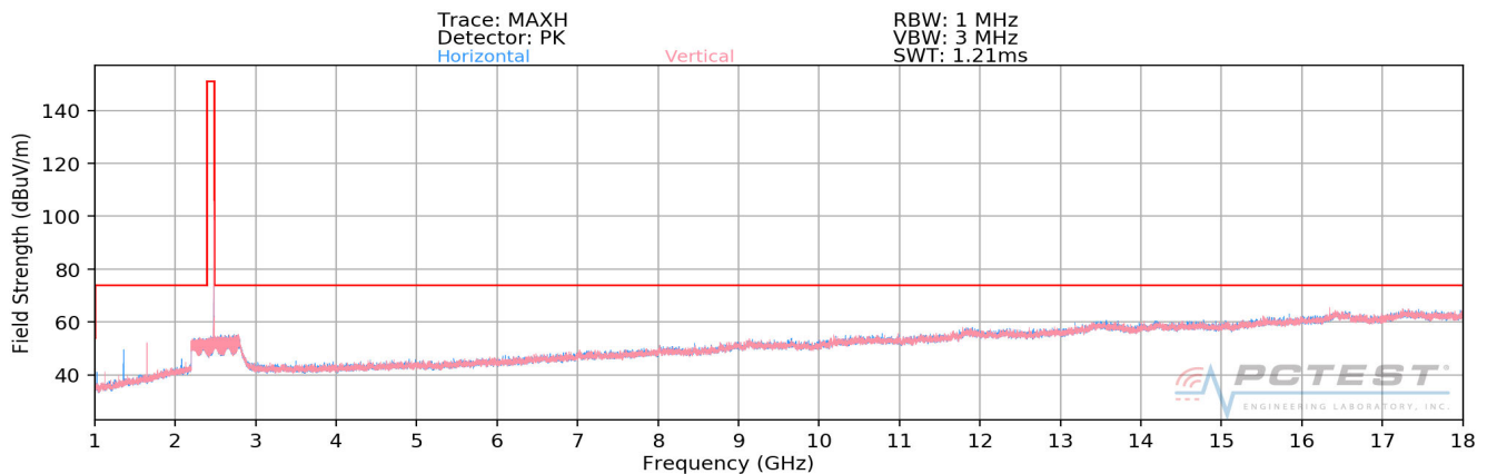
Plot 7-44. Radiated Spurious Plot above 1GHz (BT – Ch. 78)
