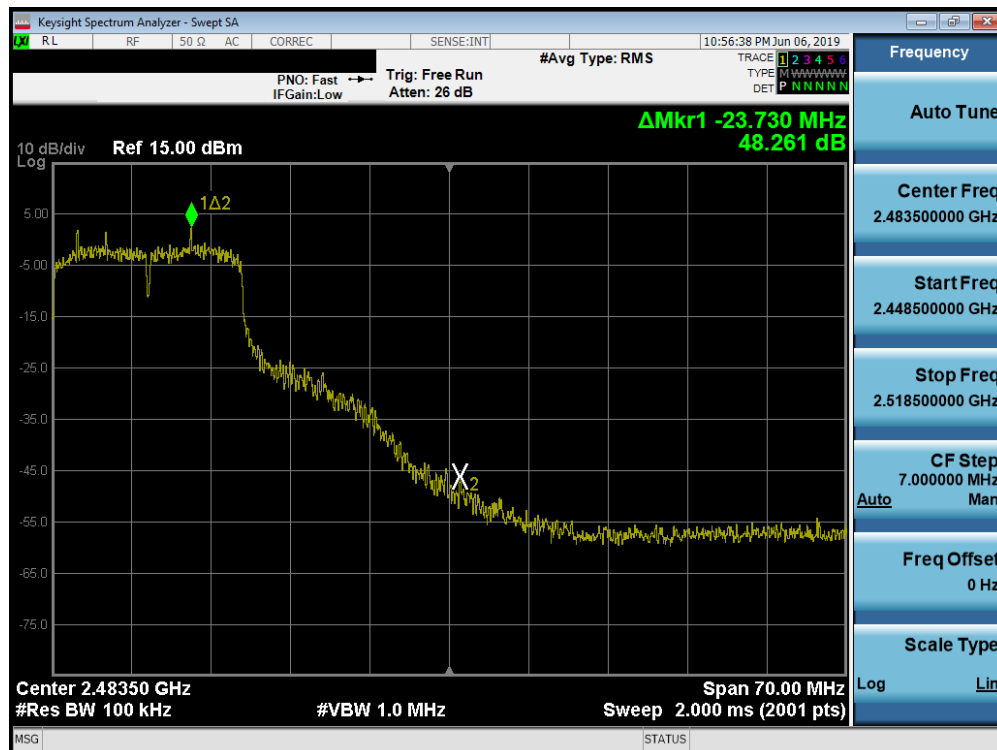
Plot 7-22. Band Edge Plot (802.11g – Ch. 10)
