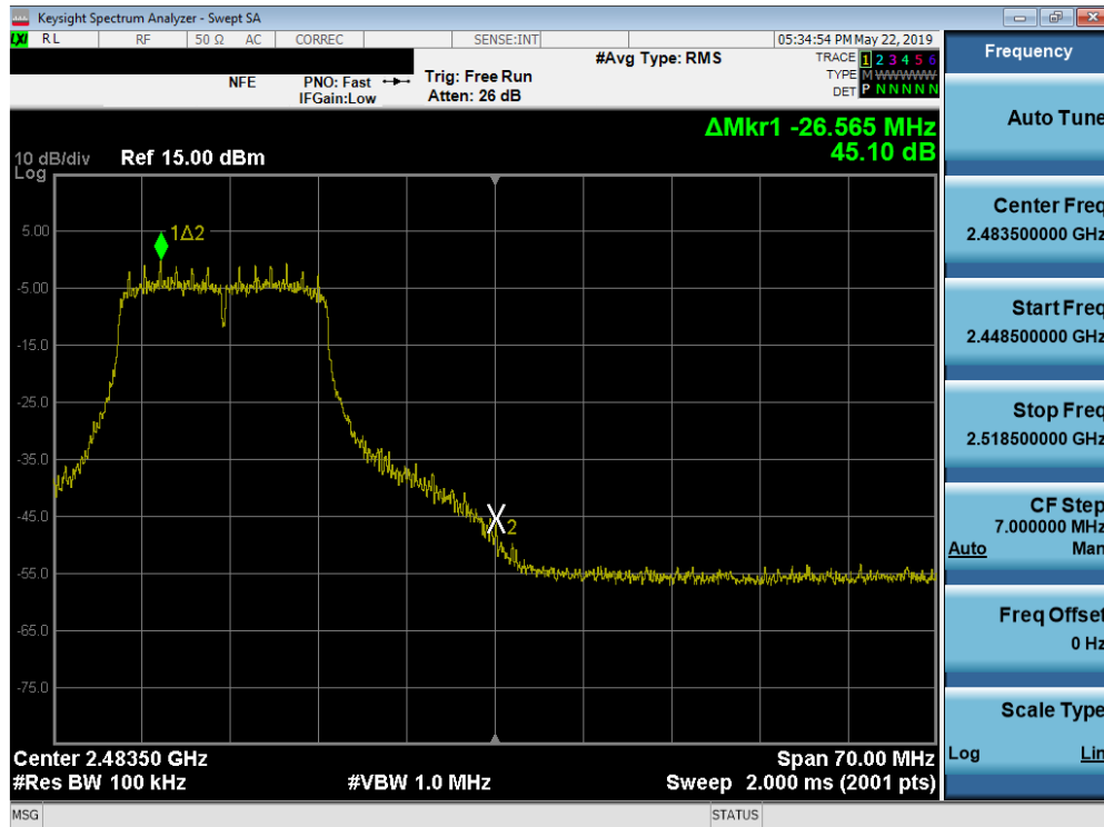
Plot 7-23. Band Edge Plot (802.11g – Ch. 11)
