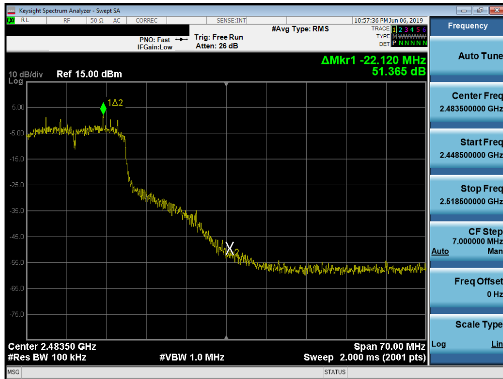
Plot 7-25. Band Edge Plot (802.11n (2.4GHz) – Ch. 10)
