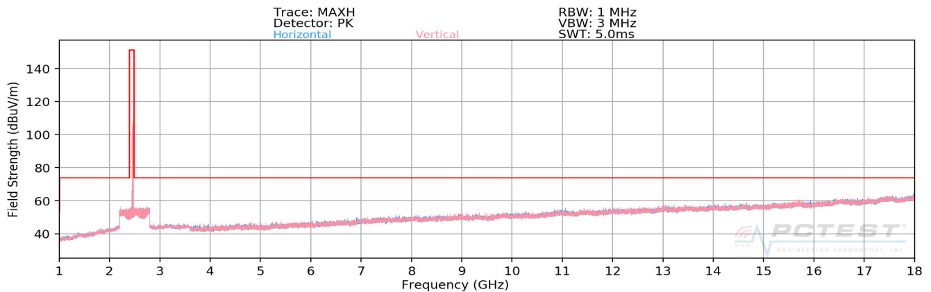
Plot 7-35. Radiated Spurious Plot above 1GHz (802.11b – Ch. 11)
