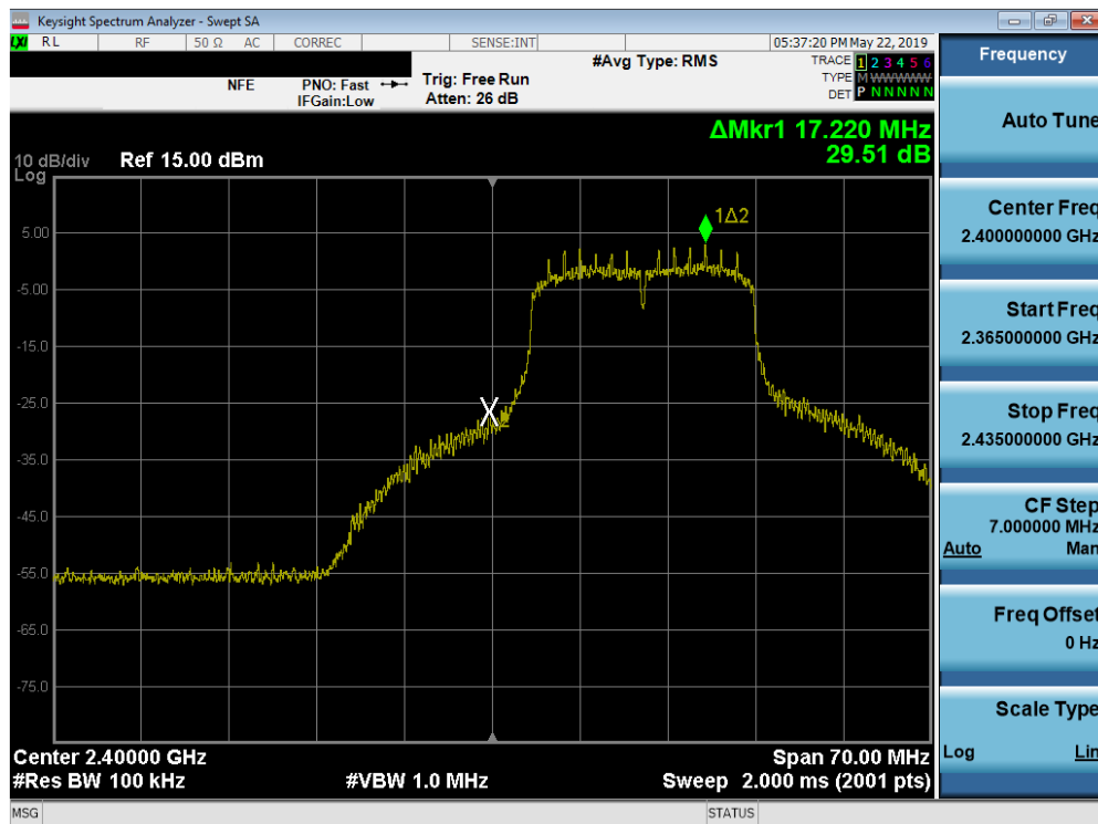
Plot 7-24. Band Edge Plot (802.11n (2.4GHz) – Ch. 1)
