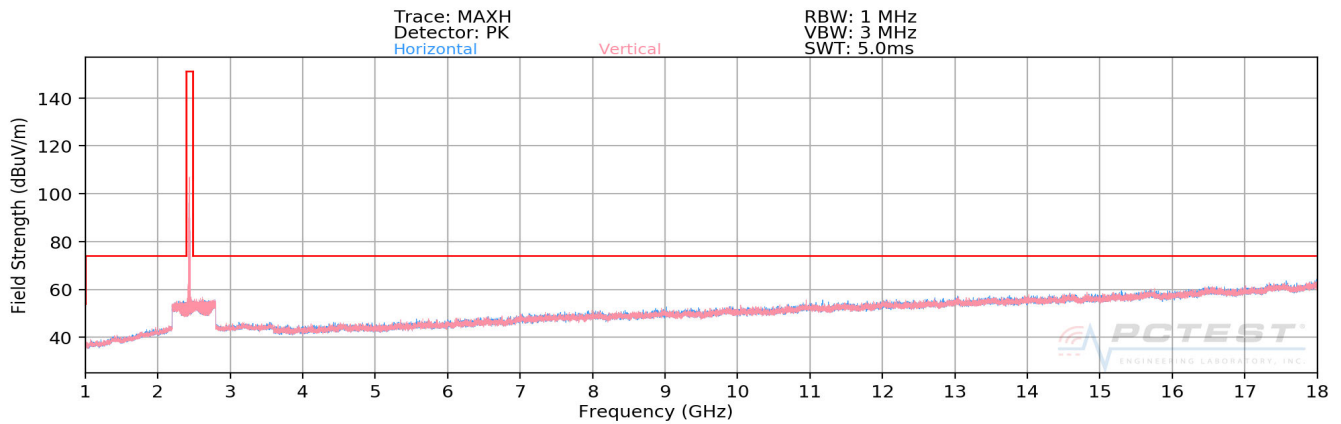
Plot 7-34. Radiated Spurious Plot above 1GHz (802.11b – Ch. 6)
