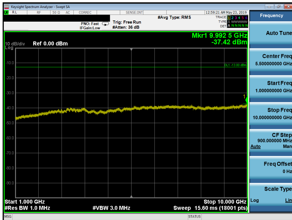
Plot 7-7. Conducted Spurious Plot (LTE Band 14, 5 MHz QPSK – RB Size 1, RB Offset 0)
