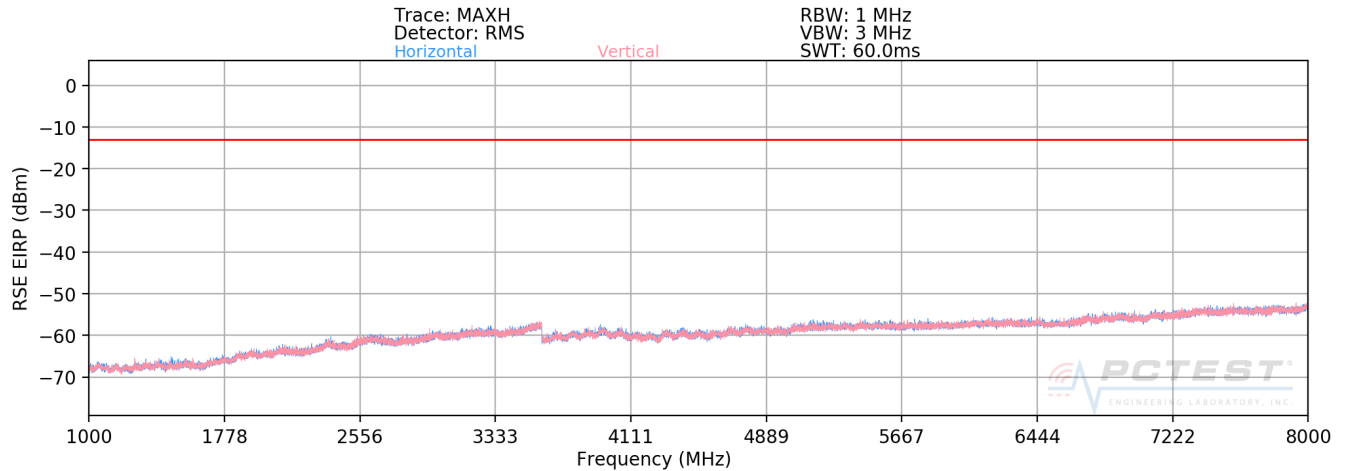
Plot 7-17. Radiated Spurious Plot above 1GHz (LTE Band 14 - Mid Channel)
