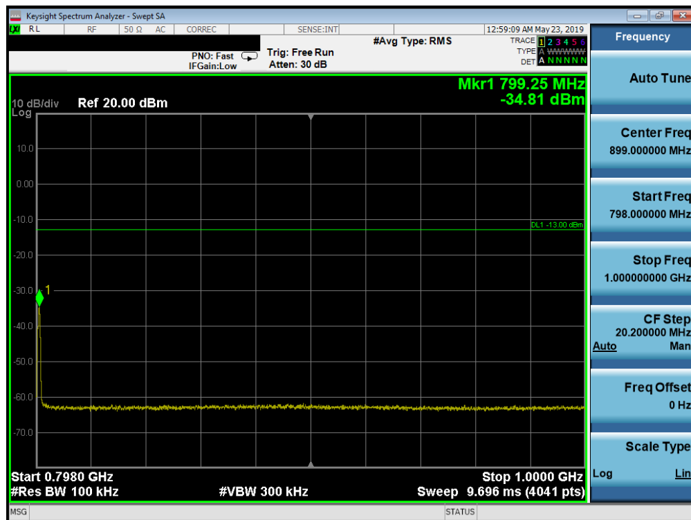
Plot 7-6. Conducted Spurious Plot (LTE Band 14, 5 MHz QPSK – RB Size 1, RB Offset 0)
