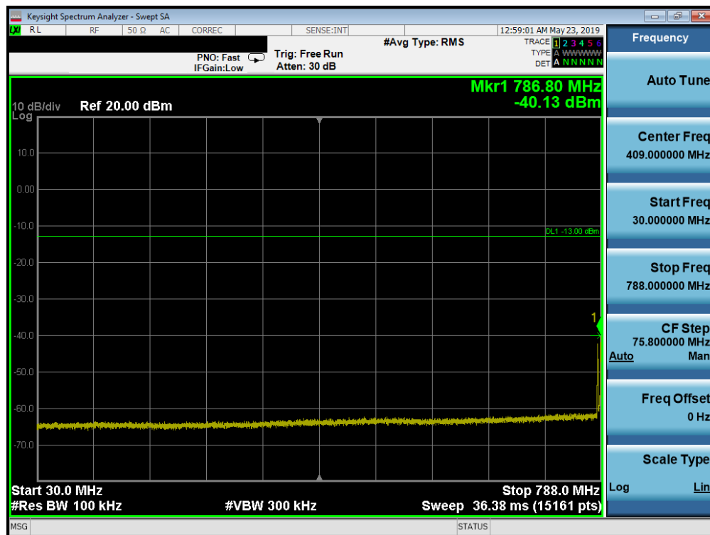
Plot 7-5. Conducted Spurious Plot (LTE Band 14, 5 MHz QPSK – RB Size 1, RB Offset 0)
